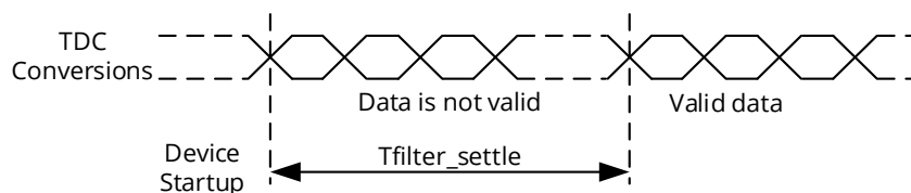
Figure 16. TDC filter output settling
