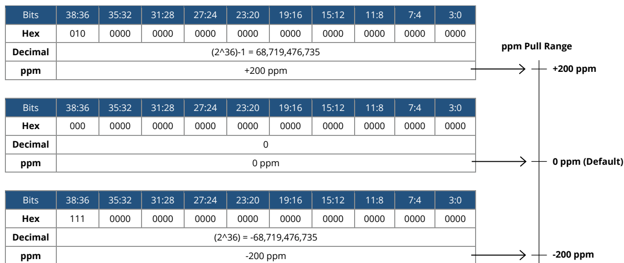
Figure 14. Frequency Control Word
