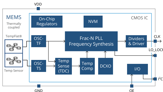
ENDR-OTT Block Diagram
