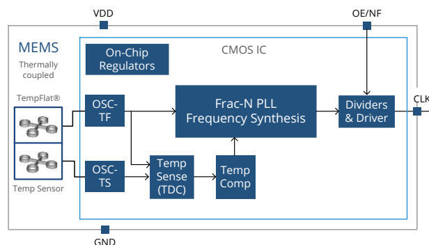
Figure 9. Block Diagram – TCXO
