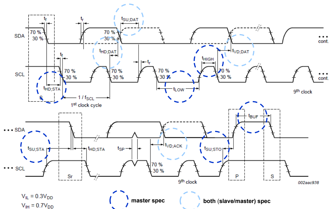
Figure 23. I²C Timing Diagram
