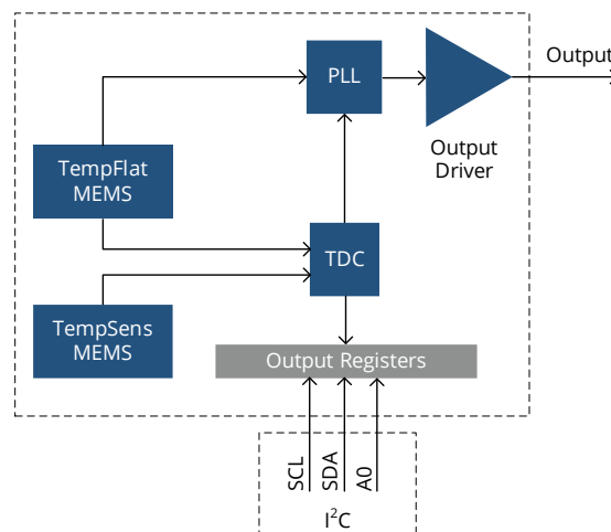
Figure 15. SiTime Super TCXO with temperature readout (based on I²C example)
