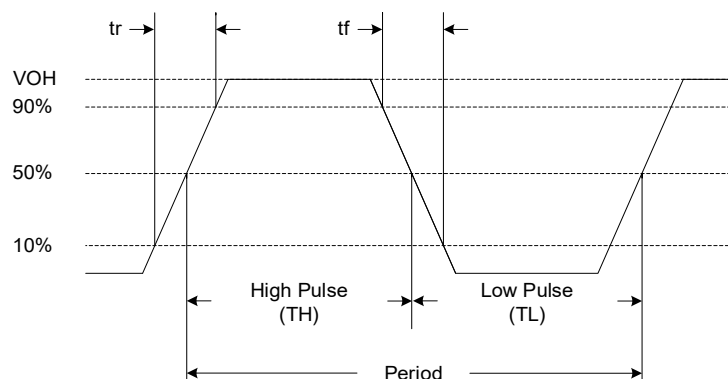
Figure 6. Regulated LVC MOS Waveform Diagram
