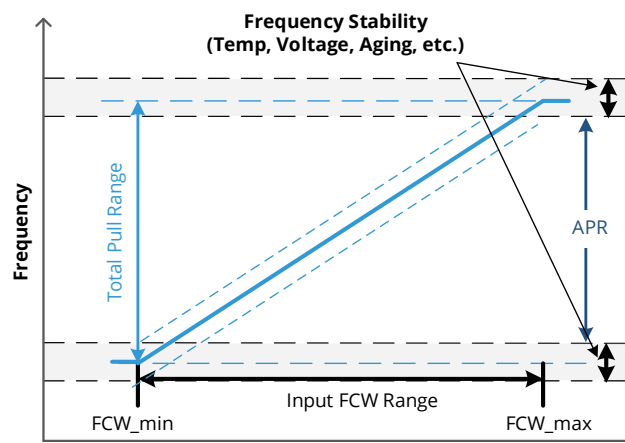
Figure 12. Typical SiTime DCTCXO Frequency vs FCW plot
