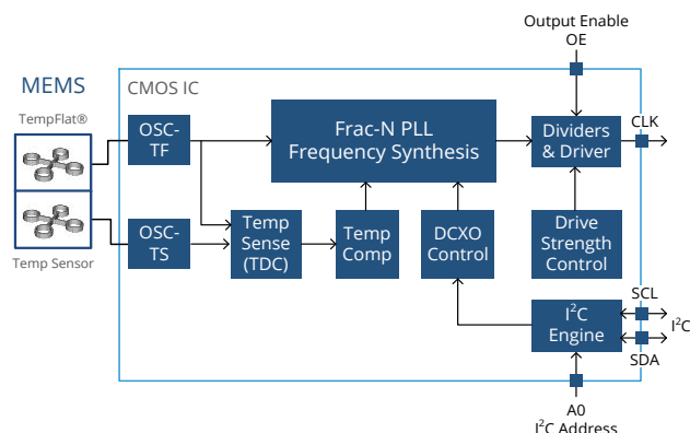
Figure 11. Block Diagram (on example of I²C interface)
