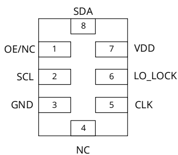
Figure 3. DCTCXO
