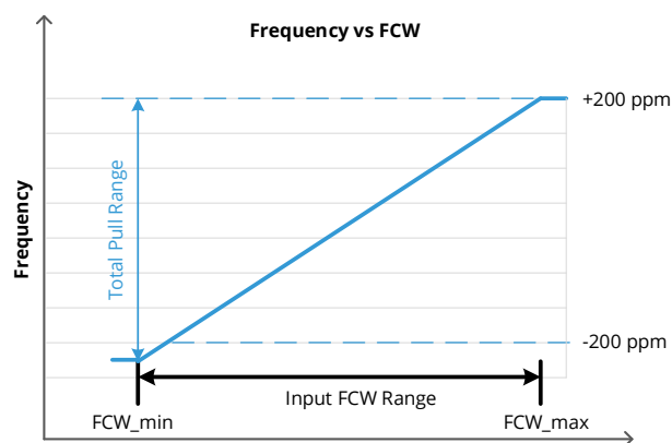
Figure 13. DCXO_Clip Illustration
