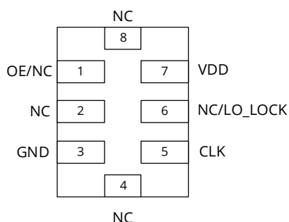
Figure 2. TCXO
