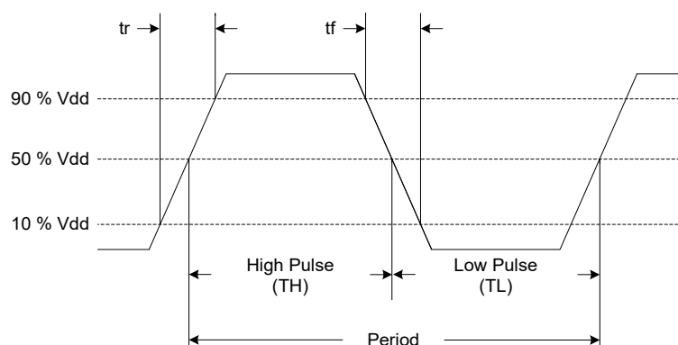
Figure 8. LVC MOS Waveform Diagram
