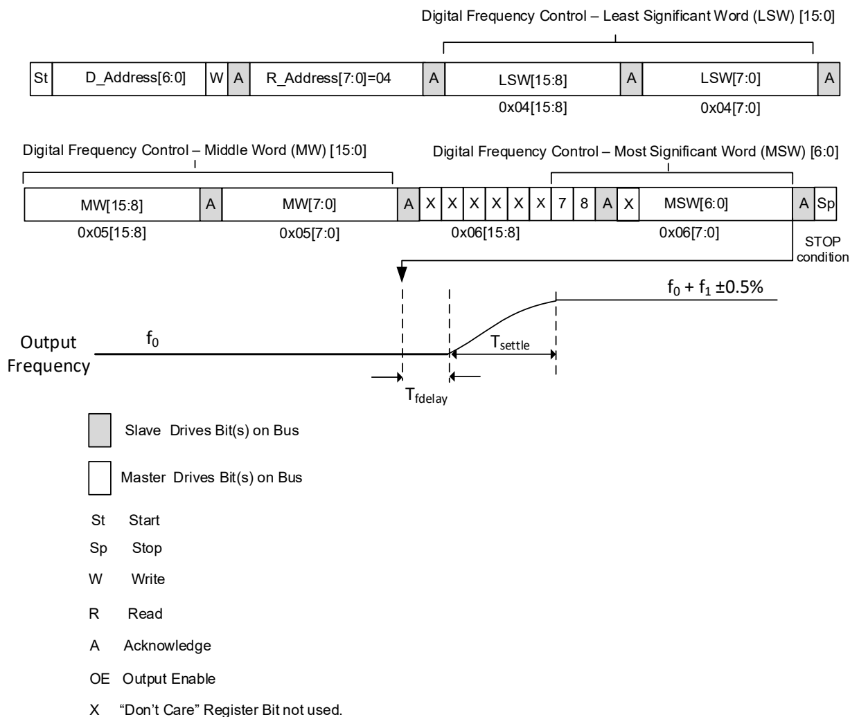
Figure 22. Writing the Frequency Control Word
