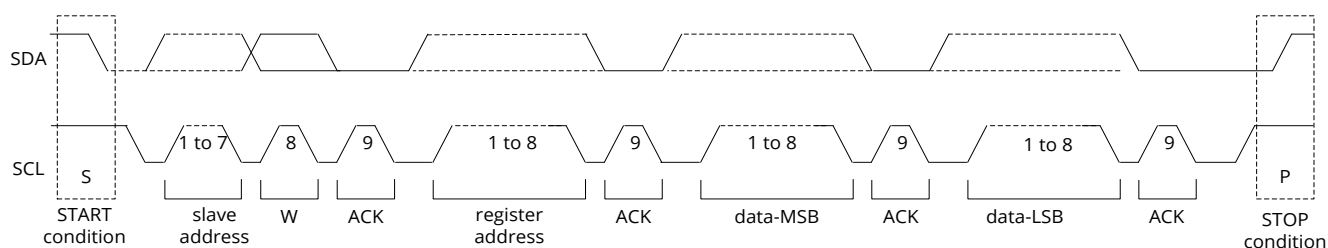
Figure 20. Parallel data byte format, write operation
