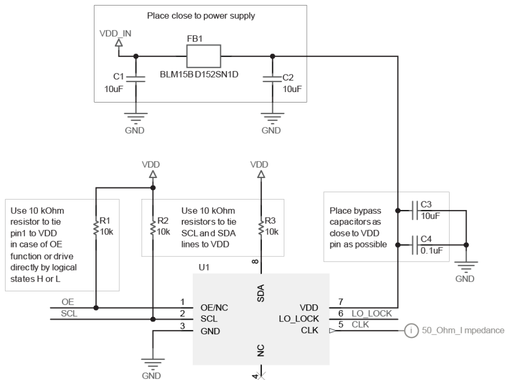
Figure 5. Schematic Example DCTXO (with LO_Lock)
