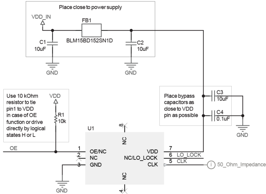
Figure 4. Schematic Example TCXO
