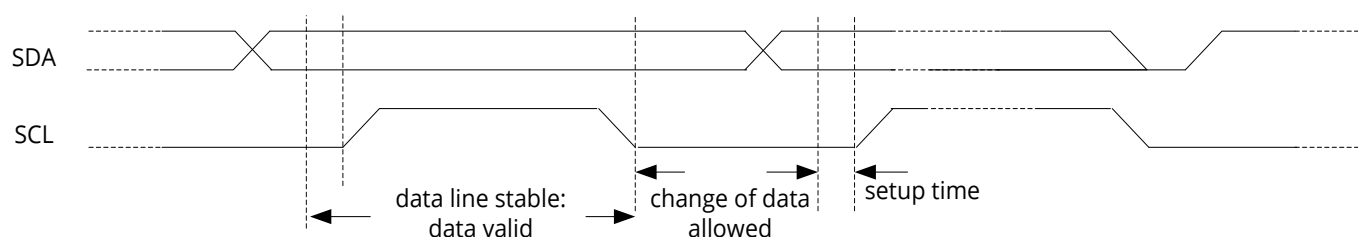
Figure 17. Data and clock timing relation in I 2 C bus
