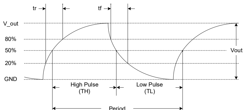
Figure 7. Clipped Sinewave Waveform Diagram
