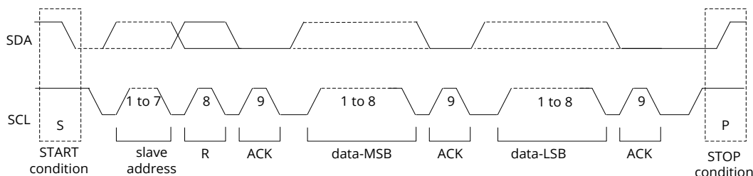
Figure 21. Parallel data byte format, read operation
