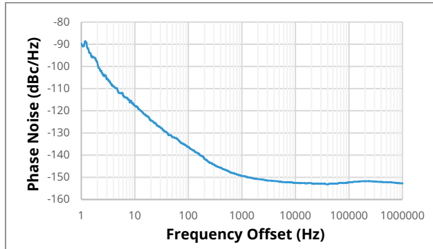
Figure 1. ENDR-OTT Phase Noise – 10 MHz Fc
