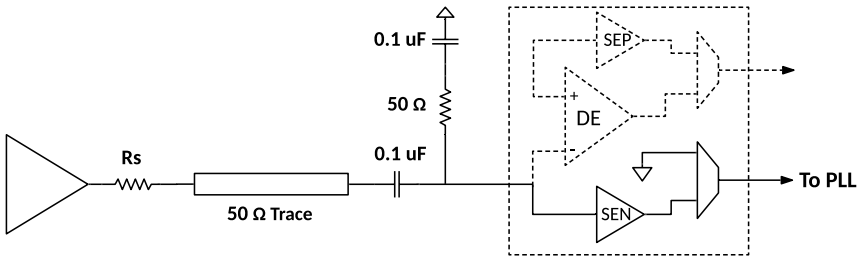
Figure 17. Interface Type III SE AC Coupled with 50 ohm termination
