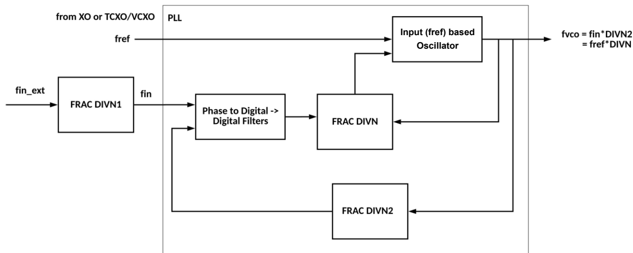
Figure 5. PLL Internals
