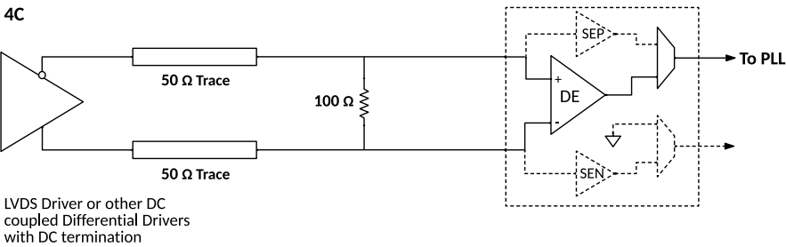
Figure 20. Interface Type IV Differential DC Coupled 4C
