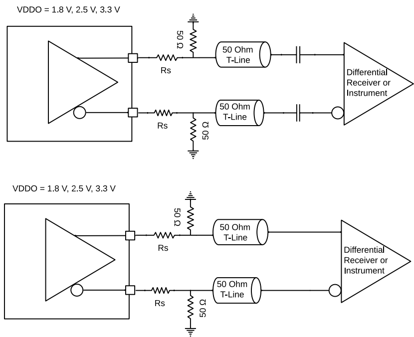
Figure 39. Output Driver used with traditional HCSL receiver.
