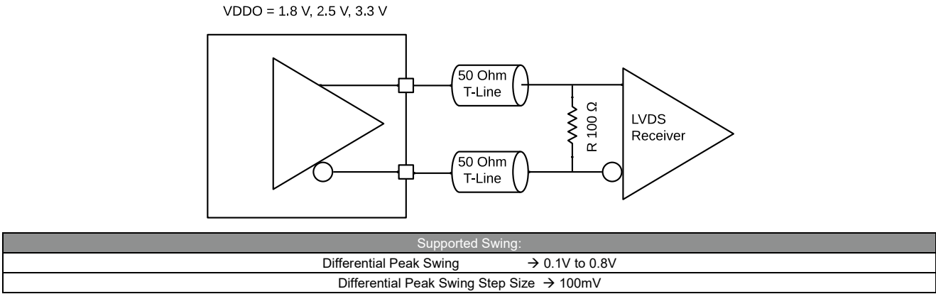
Figure 34. Output Driver used with traditional DC Coupled LVDS receiver
