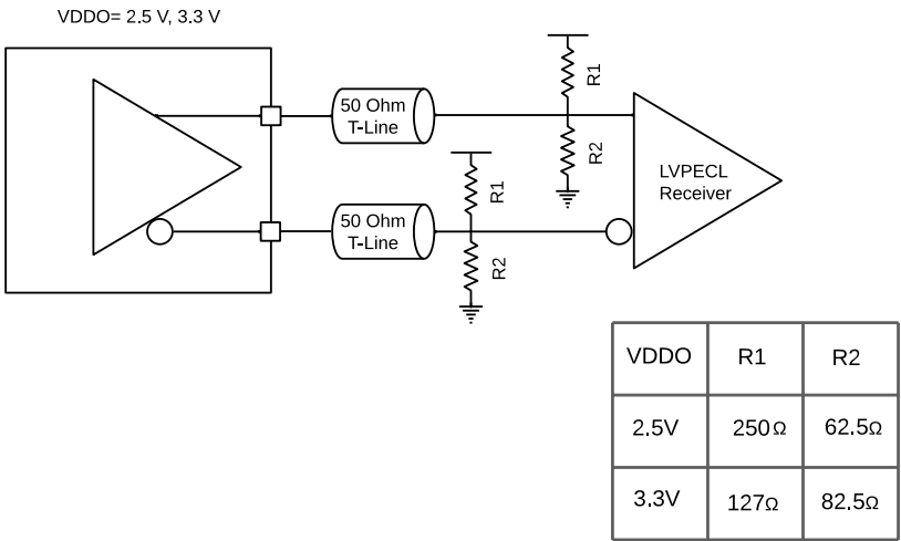
Figure 36. LVPECL Alternate DC termination: Thevenin
