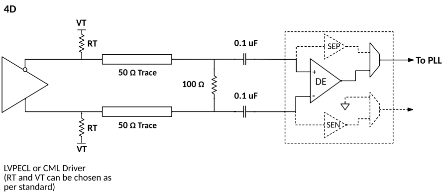
Figure 21. Interface Type IV Differential AC Coupled 4C
