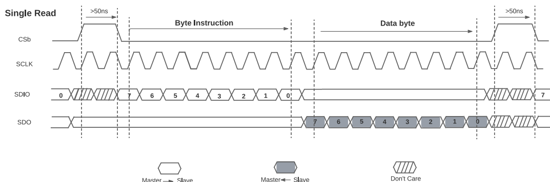
Figure 57. SPI Single Read
