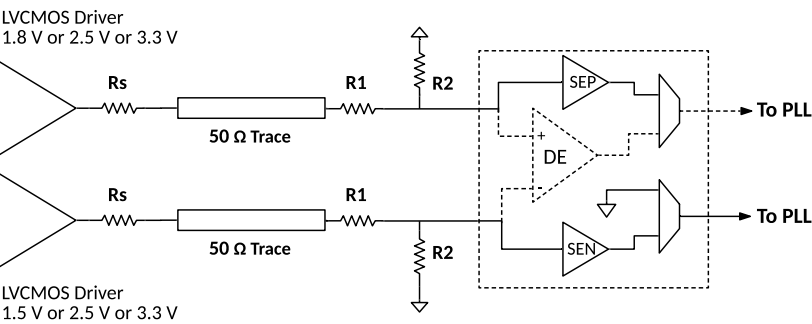
Figure 15. Interface Type-I: Single Ended DC Coupled
