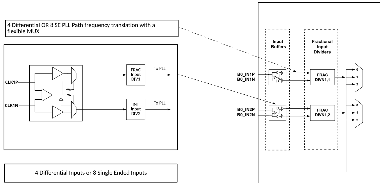
Figure 12. SiT95924 Input Slave Architecture
