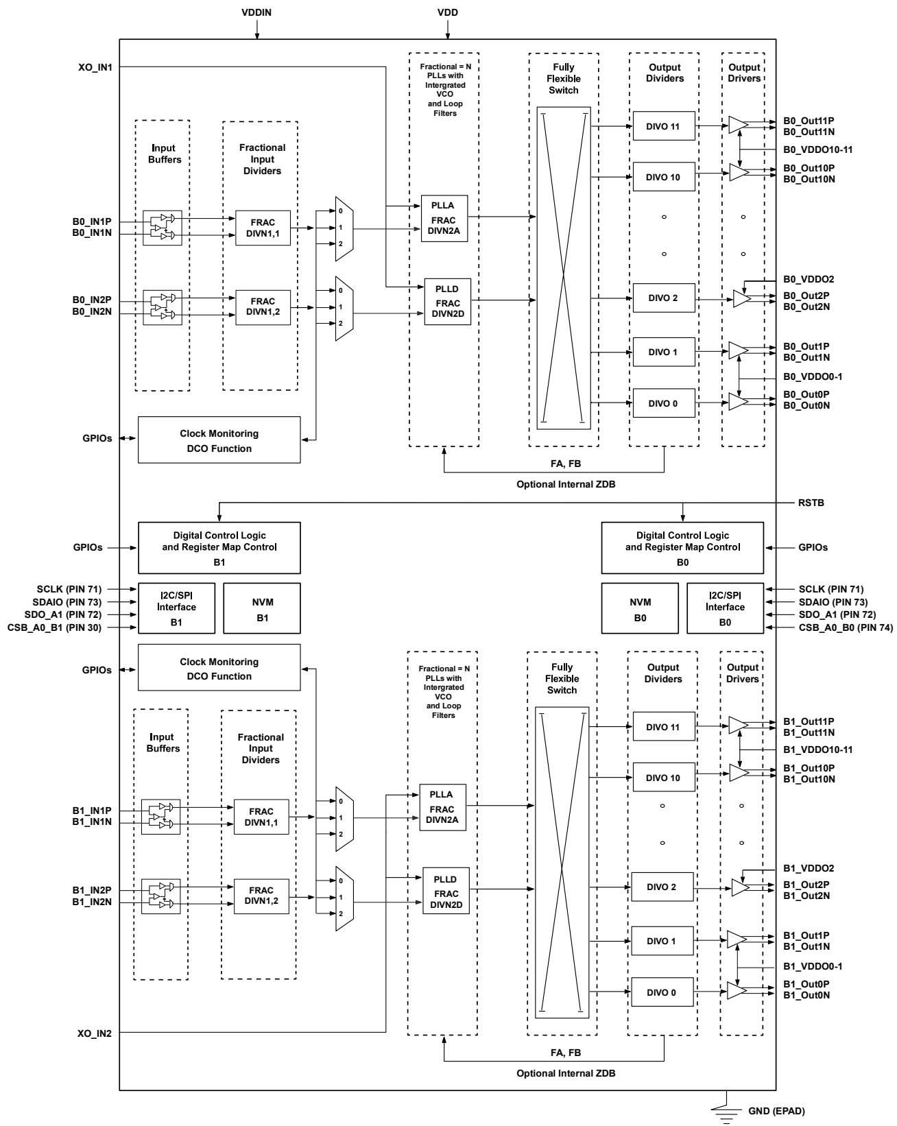
Figure 3. SiT95924 Functional Block Diagram
