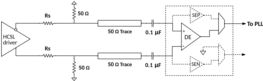
Figure 24. Interface Type V Differential AC Coupled 5C
