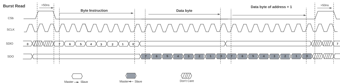
Figure 59. SPI Burst Read
