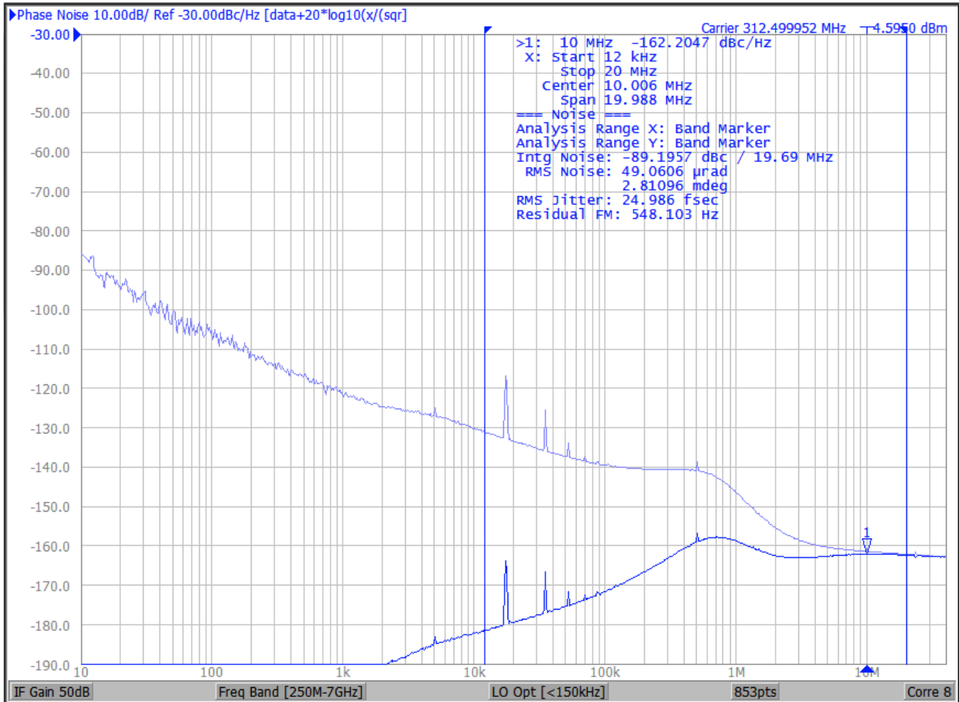
SiT95924: 312.5MHz Output (LVDS) with SiT5975AI-SE TCXO providing 86.206896M XO reference.
