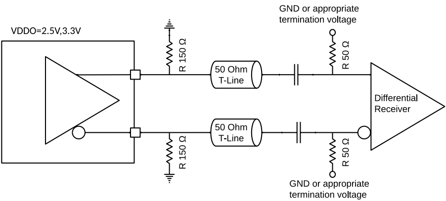
Figure 40. Alternate AC Coupled HCSL with DC Coupled resistors on Chip side.
