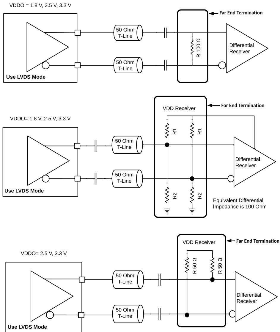
Figure 37. LVDS Output Driver used with AC Coupled terminations for various receivers.
