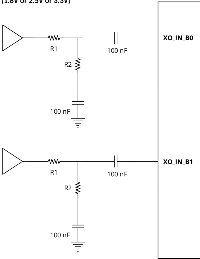
Figure 10. CMOS XO Connections
