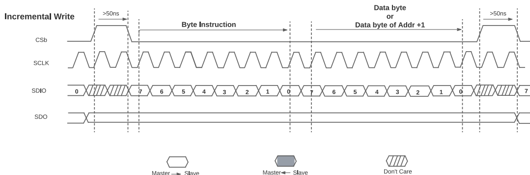
Figure 55. SPI Incremental Write
