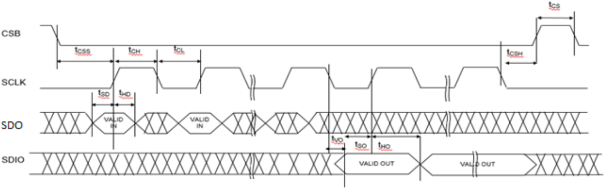
Figure 53. SPI Timing Diagram
