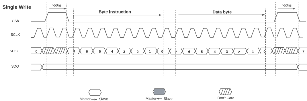
Figure 54. SPI Single Write
