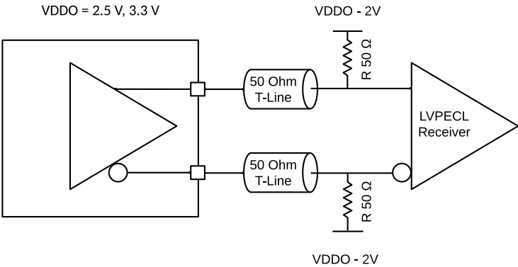
Figure 35. Output Driver used with traditional LVPECL DC Coupled receiver. (DC Termination to VDDO - 2V)
