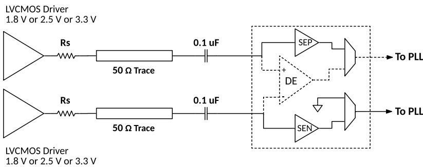
Figure 16. Interface Type II Single Ended Direct AC Coupled
