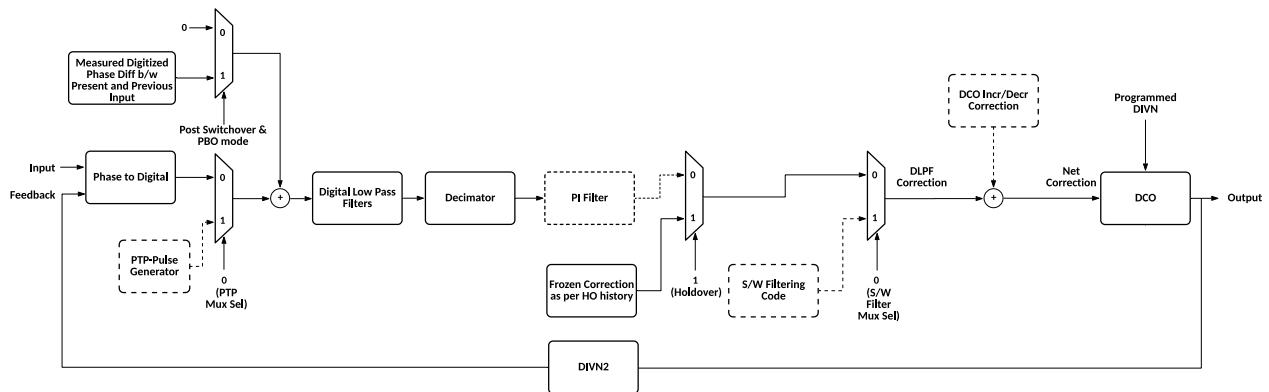
Figure 28. Holdover and Phase Build-Out Modes
