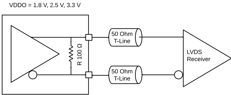
Figure 42. Output Driver used with traditional DC Coupled LVDS receiver
