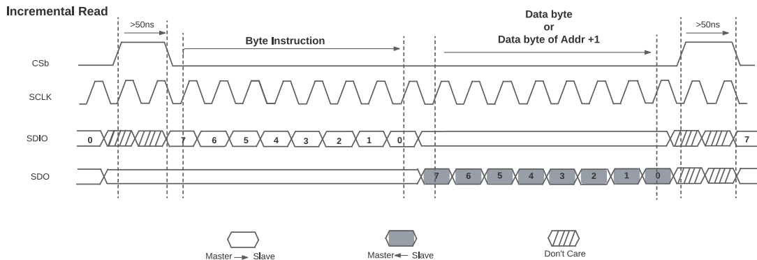
Figure 58. SPI Incremental Read
