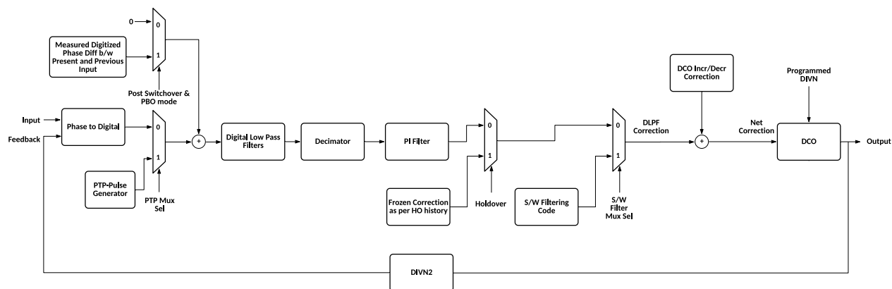
Figure 26. Basic DLPF Block Diagram
