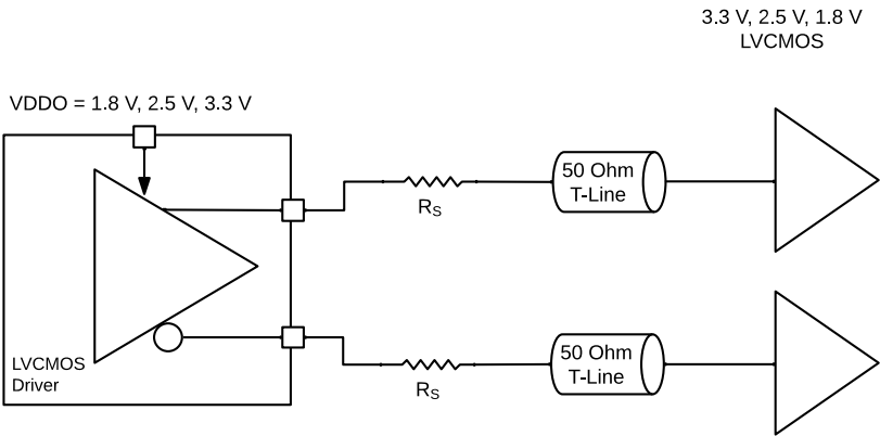
Figure 41. DC Coupled LVCMOS
