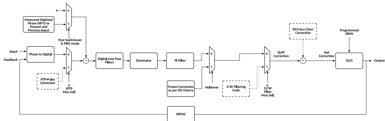
Figure 27. Basic Mode of Operation
