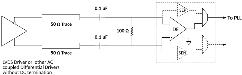
Figure 18. Interface Type IV Differential AC Coupled 4A
