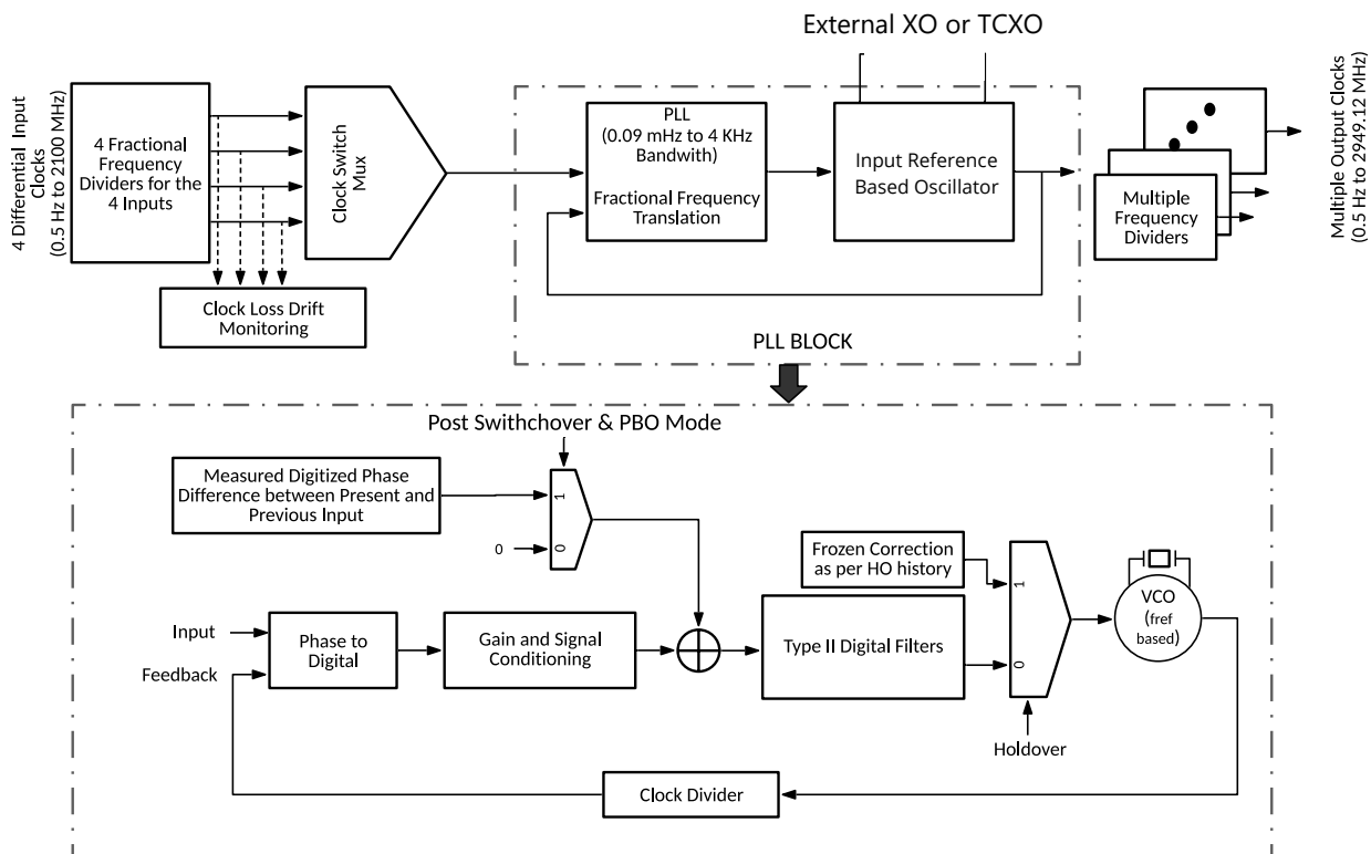
Figure 25. PLL Architecture
