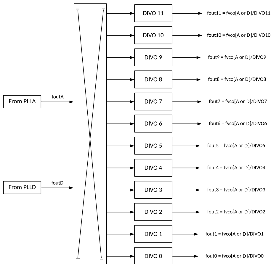
Figure 4. Bank1 / Bank2 Output Clock Distribution
