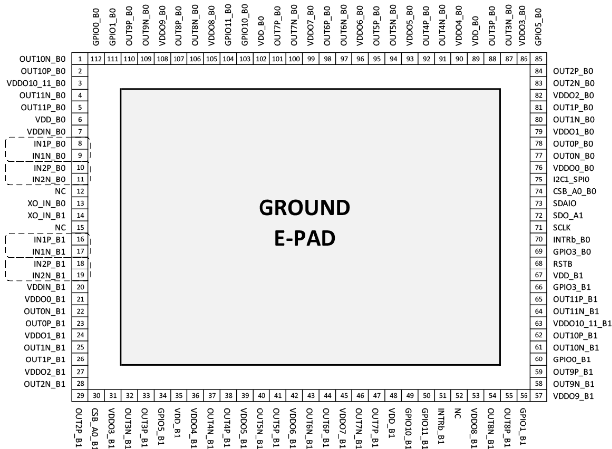
Figure 13. 4 Differential/ 8 Single Ended Inputs
