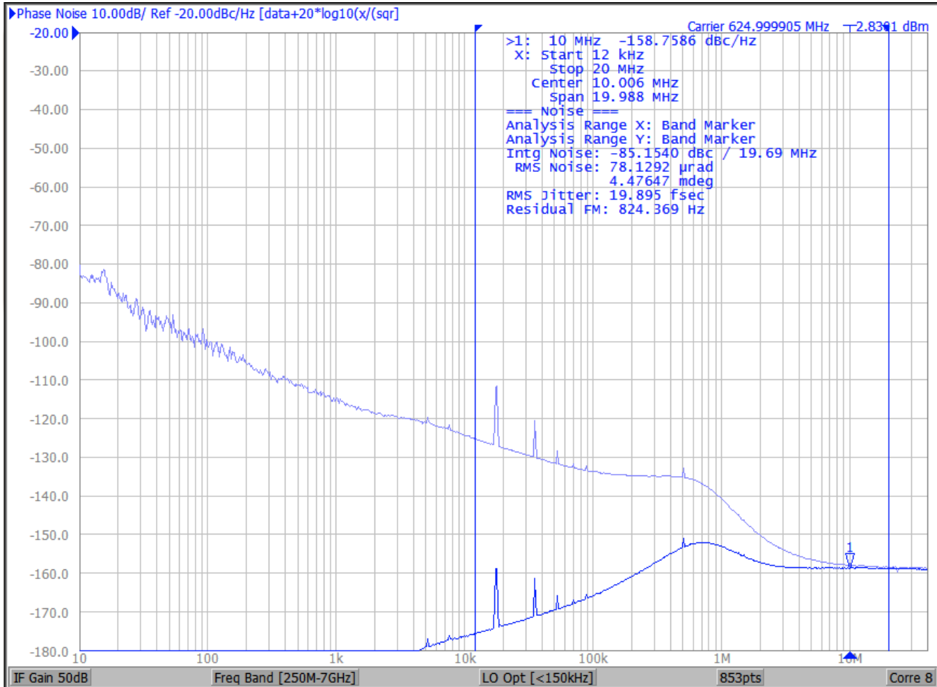
SiT95924: 625MHz Output (LVDS) with SiT5975AI-SE TCXO providing 86.2068696M XO reference.
