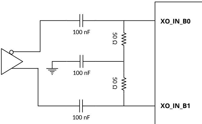
Figure 11. Differential XO Connections
