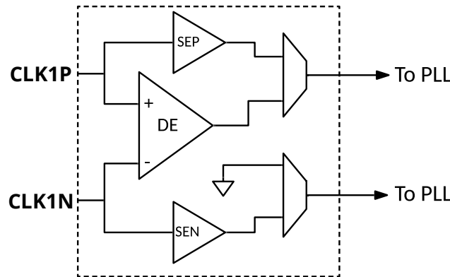
Figure 14. Input Buffer Structure
