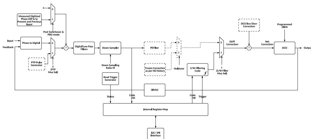
Figure 31. Closed-Loop S/W Filtering Mode
