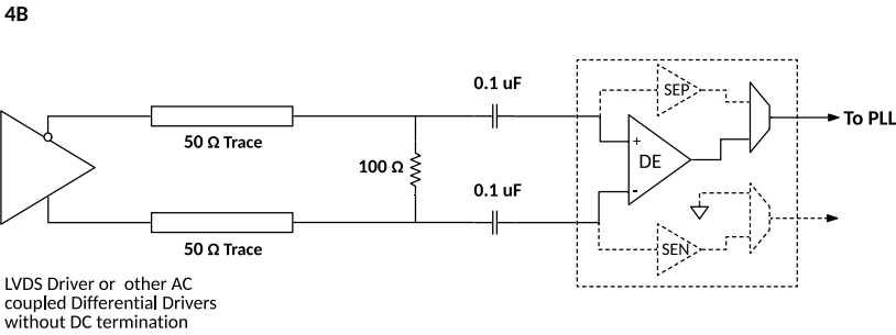
Figure 19. Interface Type IV Differential AC Coupled 4B
