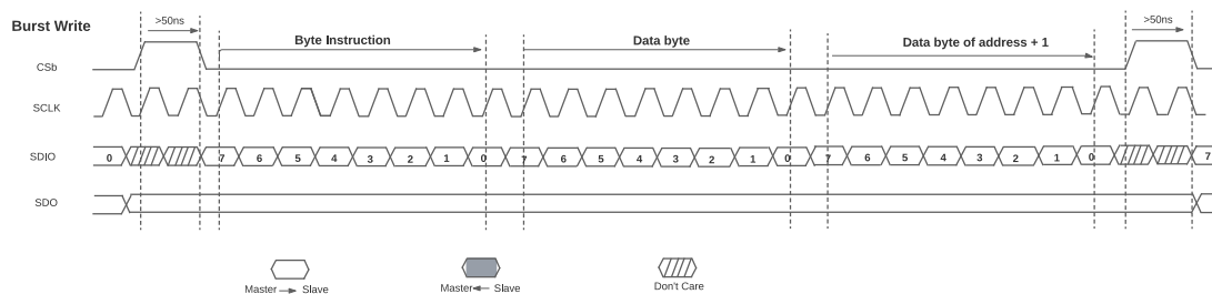
Figure 56. SPI Burst Write
