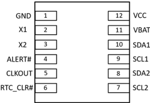
Figure 3. SiT95901 Pin Diagram
