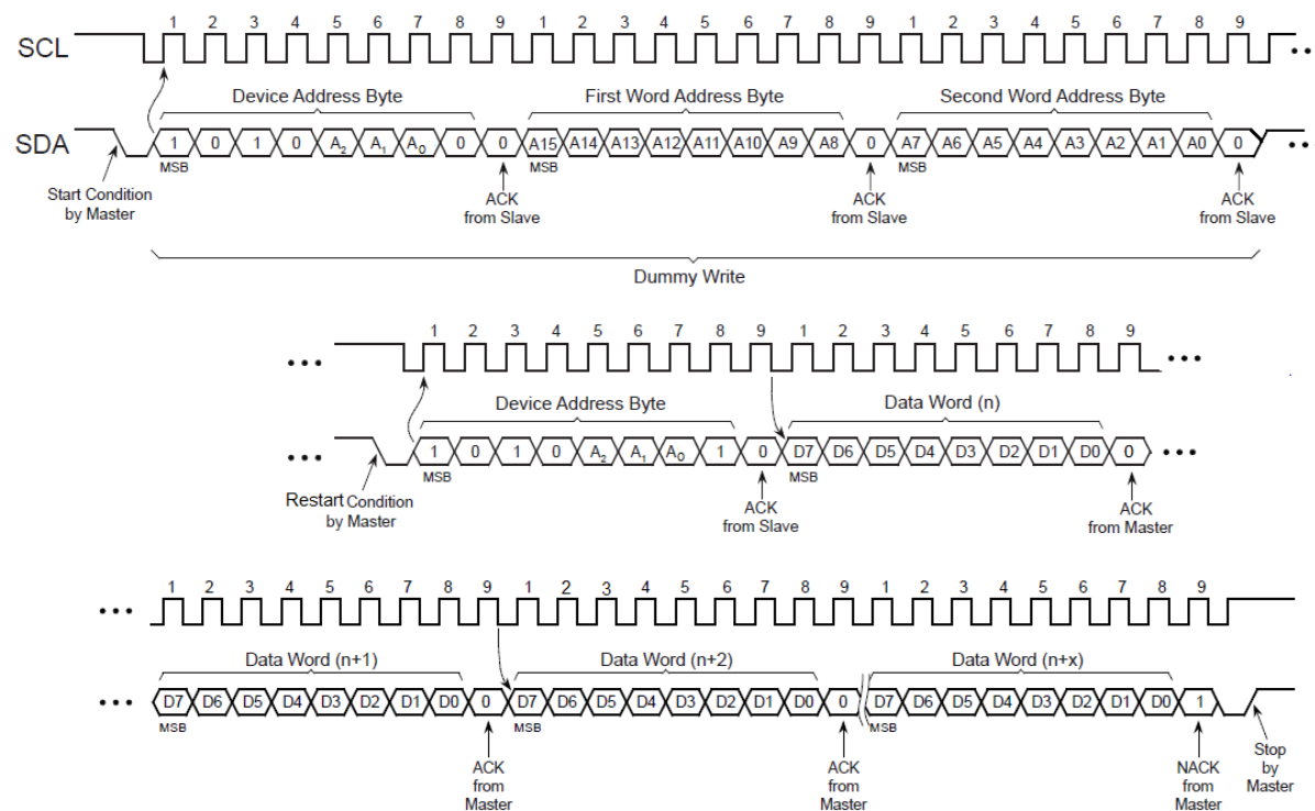
Figure 54. EEPROM read
