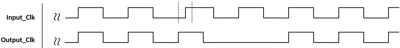
Figure 52. Case for Phase difference between 0 and 0.5\pi
