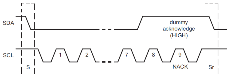
Figure 57. Start Byte Procedure
