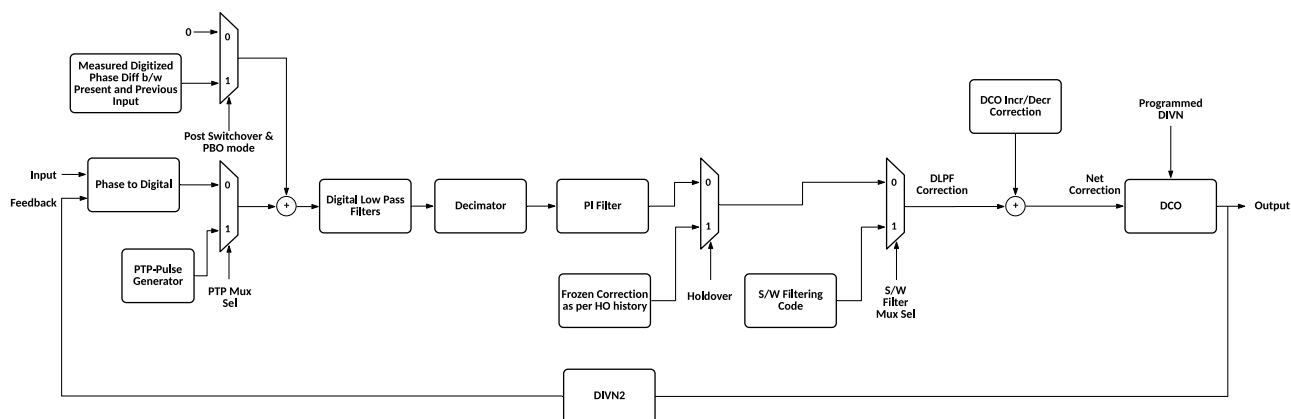
Figure 27. Basic DLPF Block Diagram
