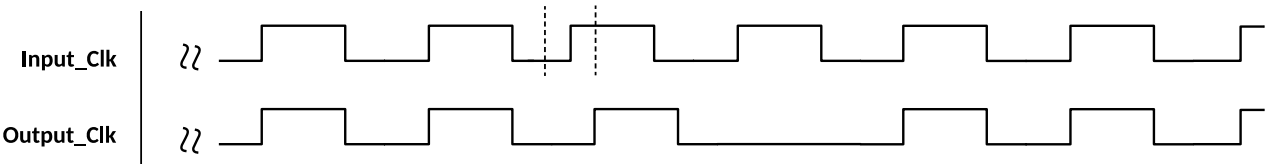
Figure 53. Case for Phase difference between -0.5\pi and 0
