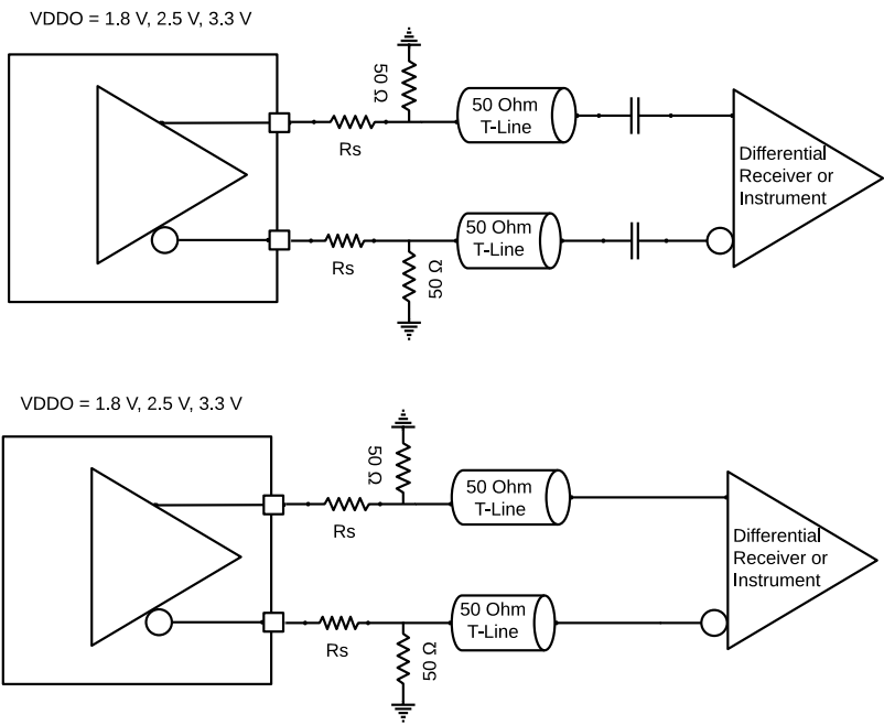
Figure 42. Output Driver used with traditional HCSL receiver.
