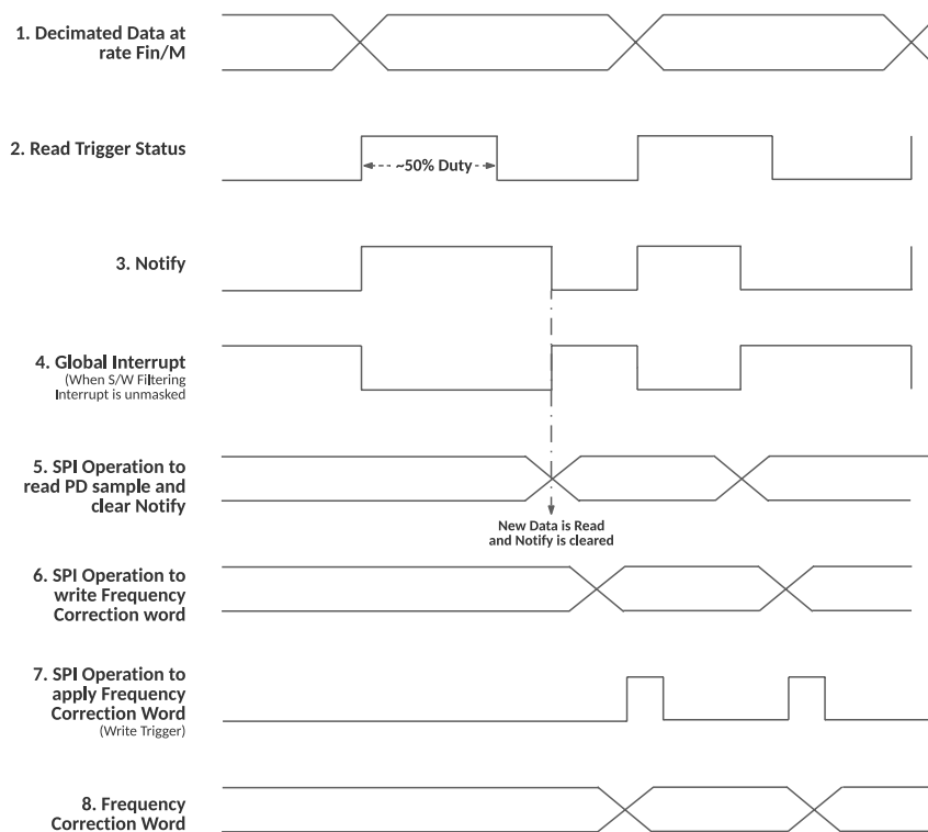
Figure 31. Timing Diagram Illustrating the Closed-Loop S/W Filtering Sequence
