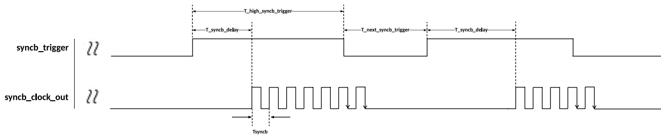
Figure 47. syncb_clock_out behavior with respect to syncb_trigger
