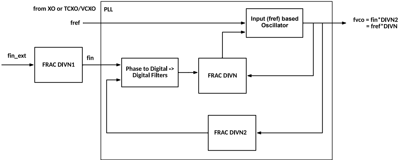
Figure 5. PLL Internals
