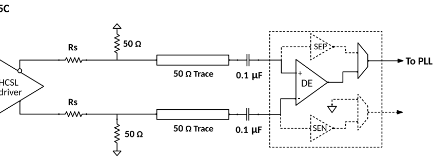
Figure 25. Interface Type V Differential AC Coupled 5C
