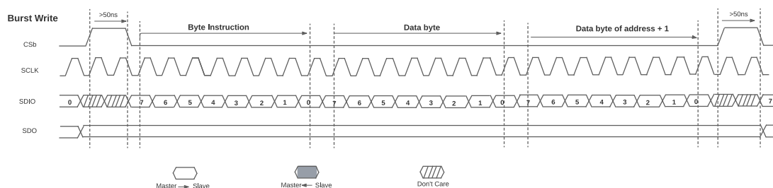
Figure 62. SPI Burst Write
