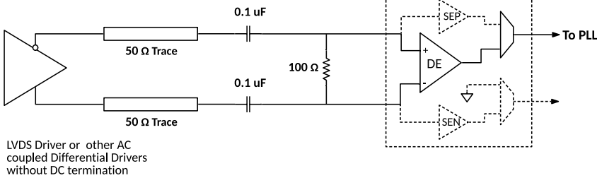
Figure 19. Interface Type IV Differential AC Coupled 4A
