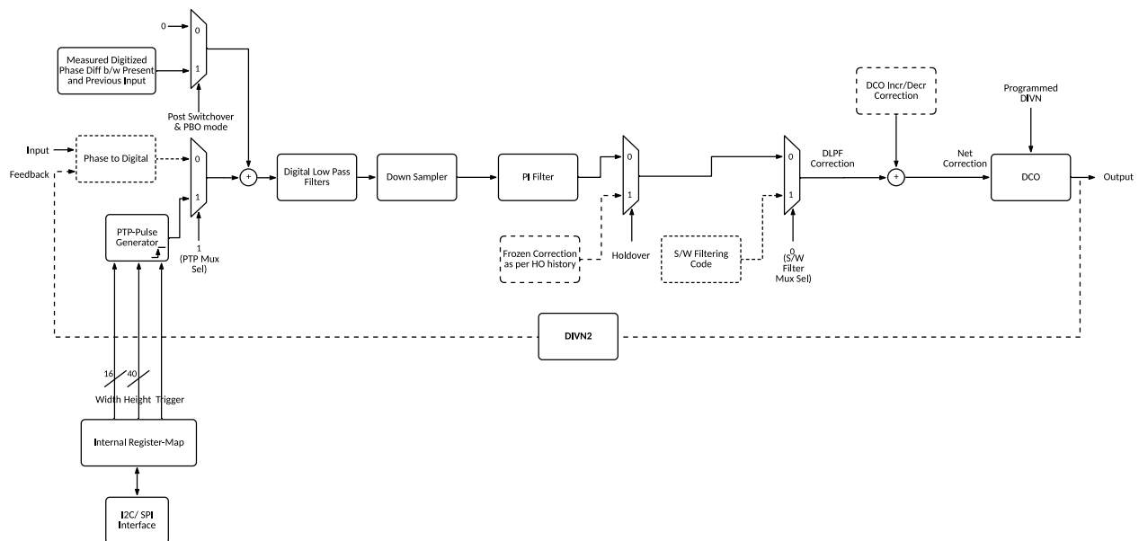
Figure 32. PTP Mode
