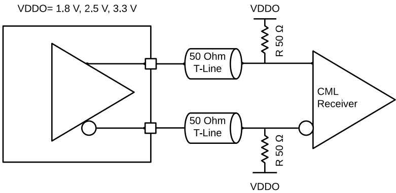
Figure 41. Output Driver used with traditional DC Coupled CML receiver.
