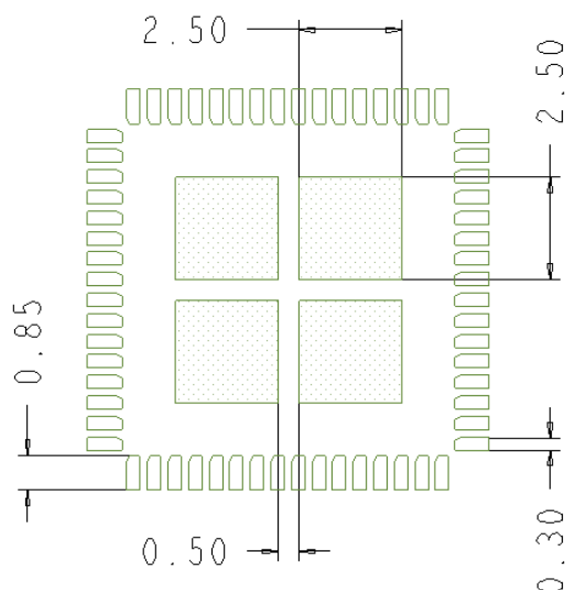
Figure 68. Solder Mask Design
