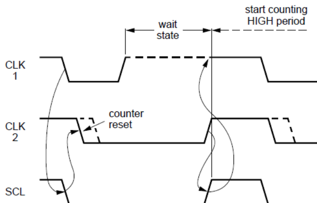
Figure 55. SCL Synchronization
