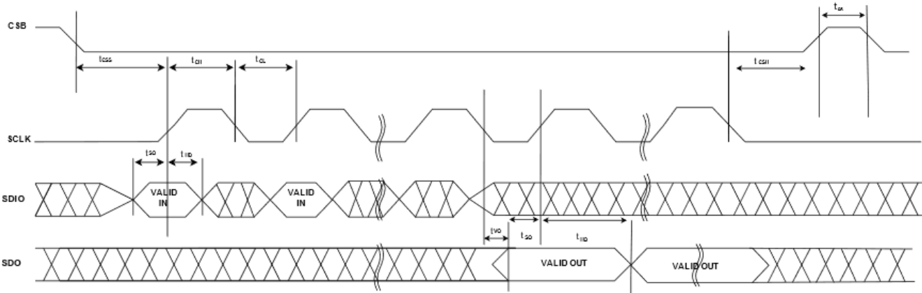
Figure 59. SPI Timing Diagram
