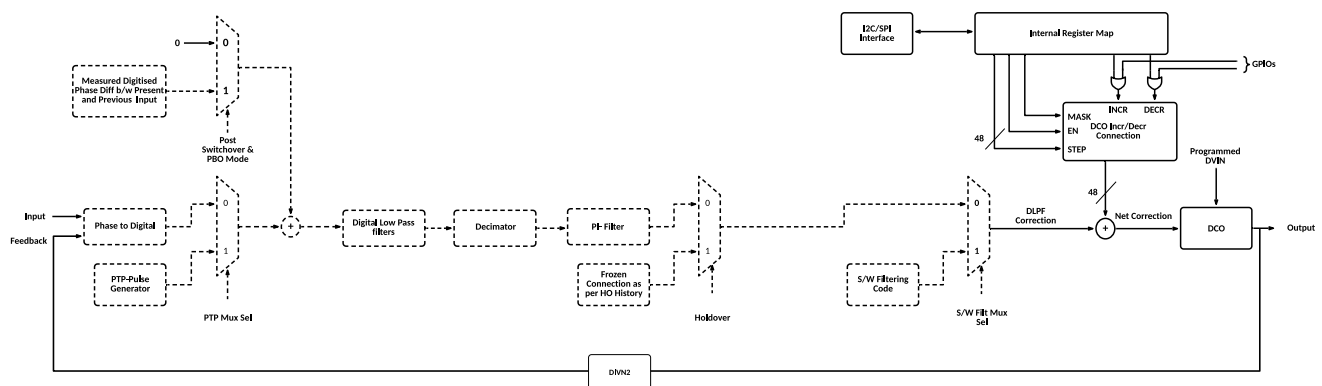
Figure 33. DCO Increment/Decrement path for Inner-Loop
