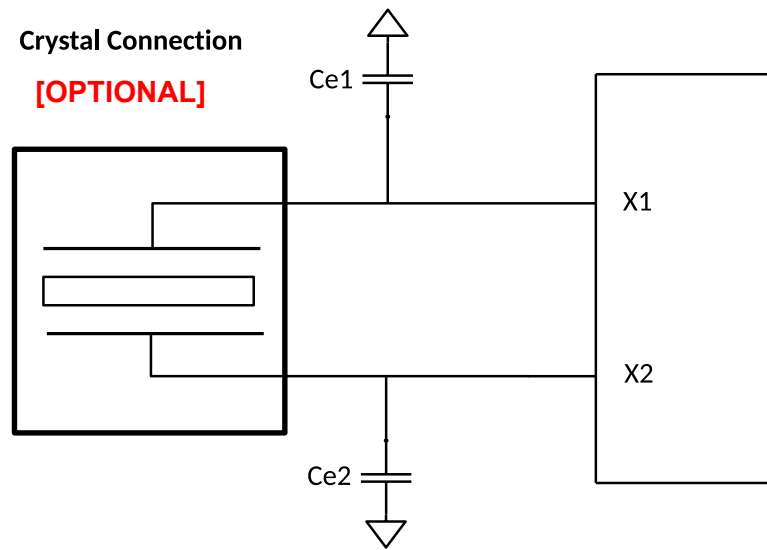
Figure 10. Crystal Connections
