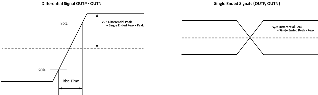
Figure 36. Waveform Convention
