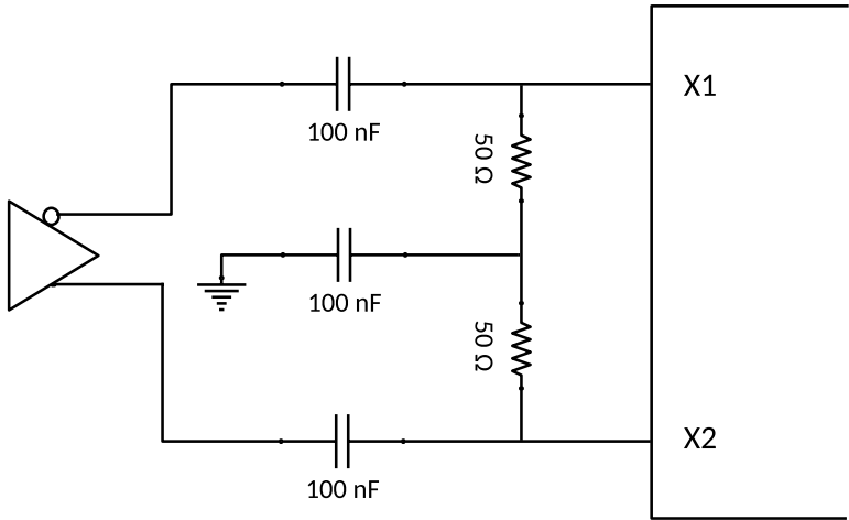
Figure 12. Differential XO Connections
