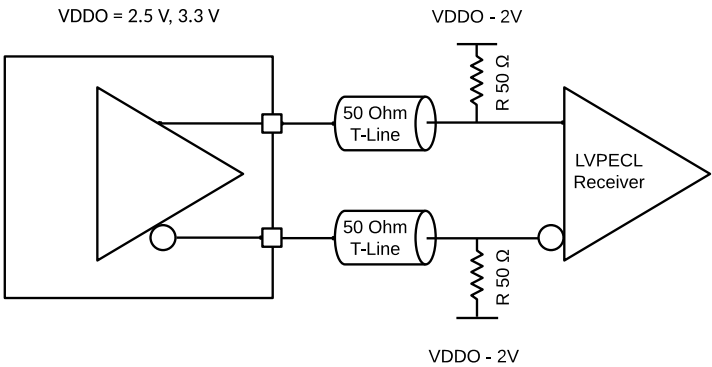
Figure 38. Output Driver used with traditional LVPECL DC Coupled receiver.
