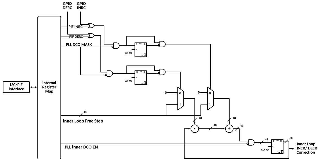
Figure 34. Architecture of the Inner-Loop Increment/Decrement path
