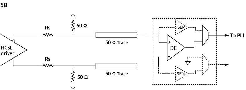
Figure 24. Interface Type V Differential DC Coupled 5B
