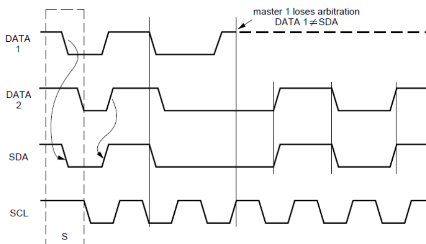
Figure 56. Arbitration
