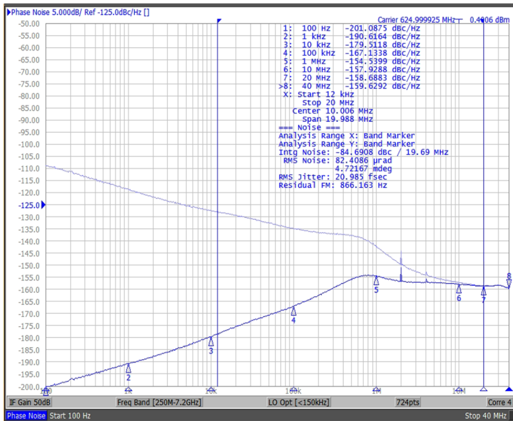
SiT95317: 625M Output (LVDS) with 96M SMA100B XO Source
