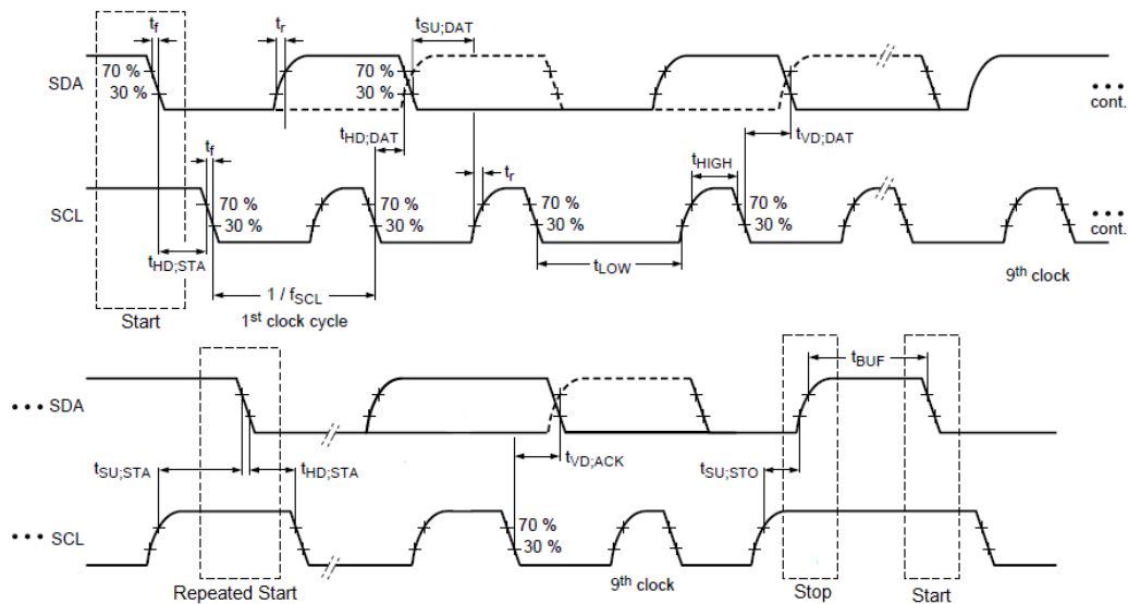
Figure 58. I2C Timing Waveform
