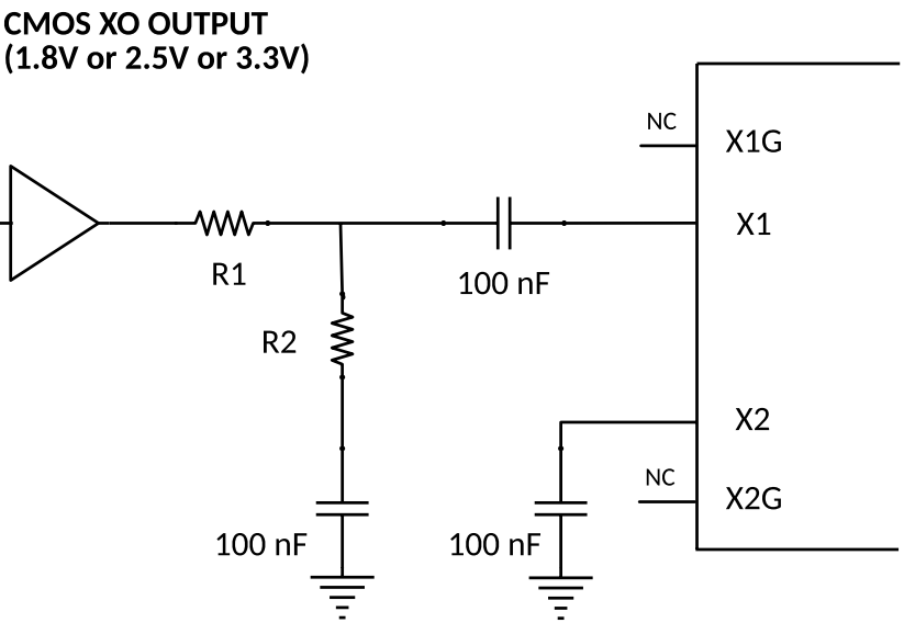
Figure 11. CMOS XO Connections
