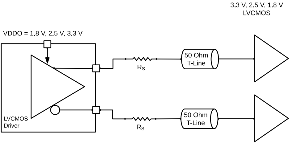
Figure 44. DC Coupled LVCMOS
