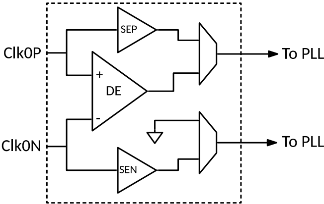
Figure 15. Input Buffer Structure
