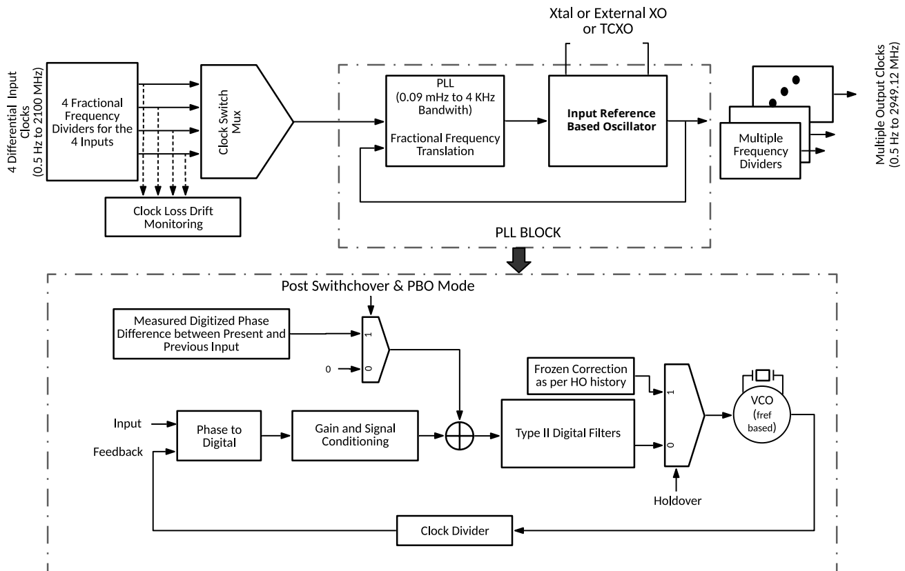
Figure 26. PLL Architecture
