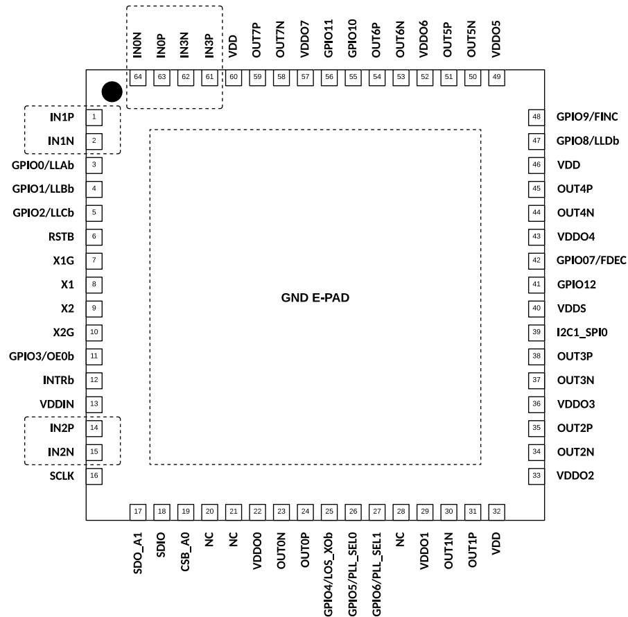
Figure 14. 4 Differential/ 8 Single Ended Inputs
