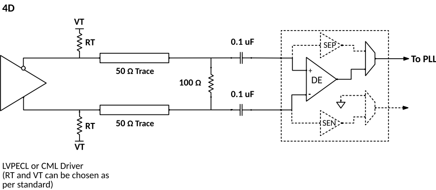
Figure 22. Interface Type IV Differential AC Coupled 4D
