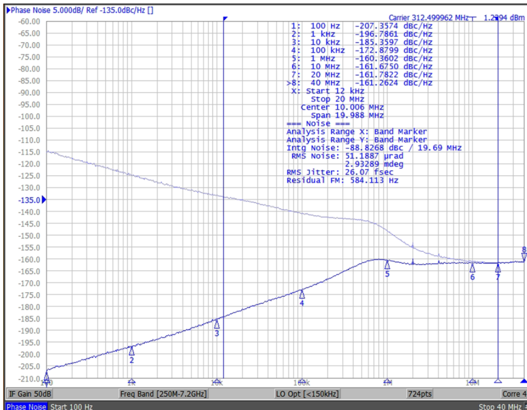
SiT95317: 312.5M Output (LVDS) with 96M SMA100B XO Source
