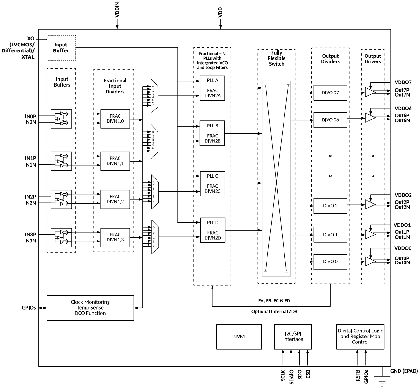
Figure 3. SiT95317 Functional Block Diagram
