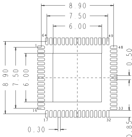
Figure 67. Land Pattern
