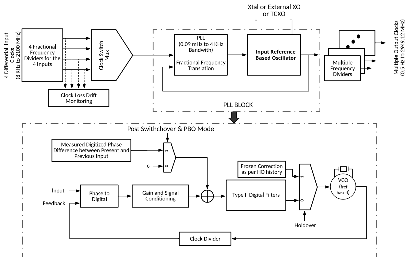
Figure 26. PLL Architecture
