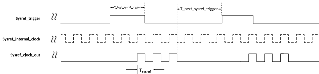
Figure 43. sysref_clock_out behaviour with respect to sysref_trigger in pulser mode
