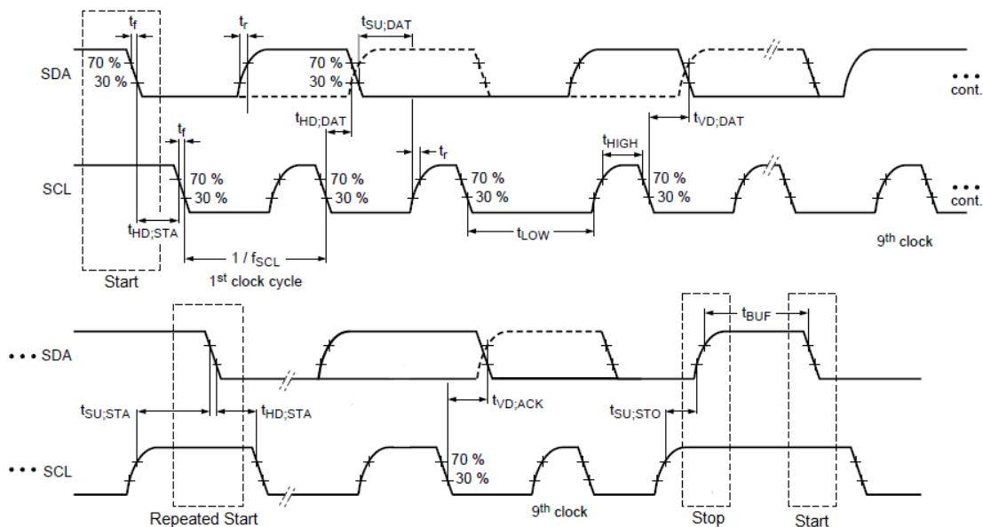
Figure 49. I2C Timing Waveform
