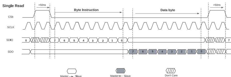
Figure 54. SPI Single Read
