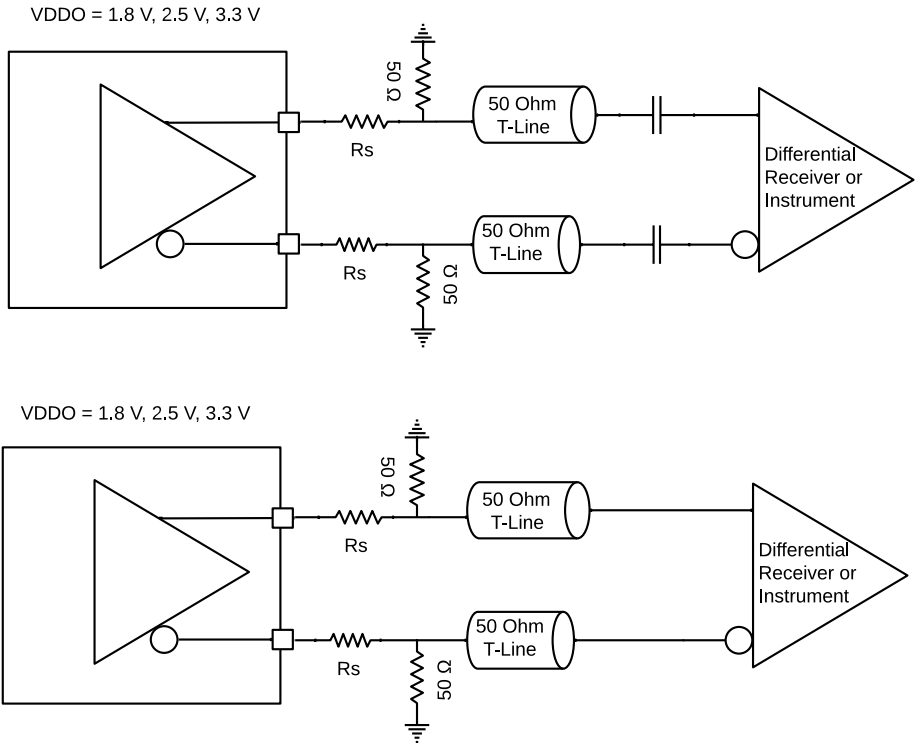
Figure 39. Output Driver used with traditional HCSL receiver
