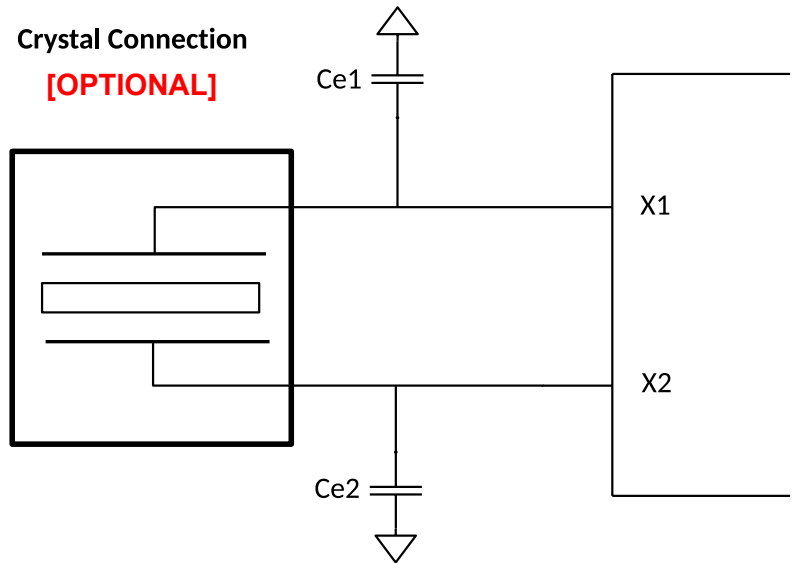
Figure 10. Crystal Connections
