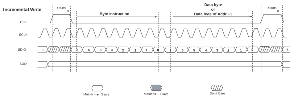
Figure 52. SPI Incremental Write
