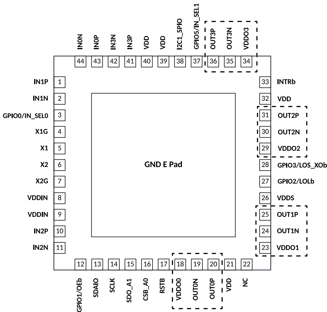
Figure 32. SiT95314 Output Drivers
