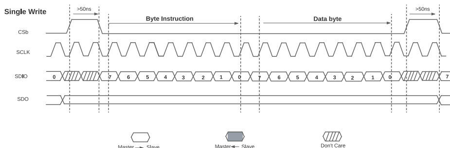
Figure 51. SPI Single Write
