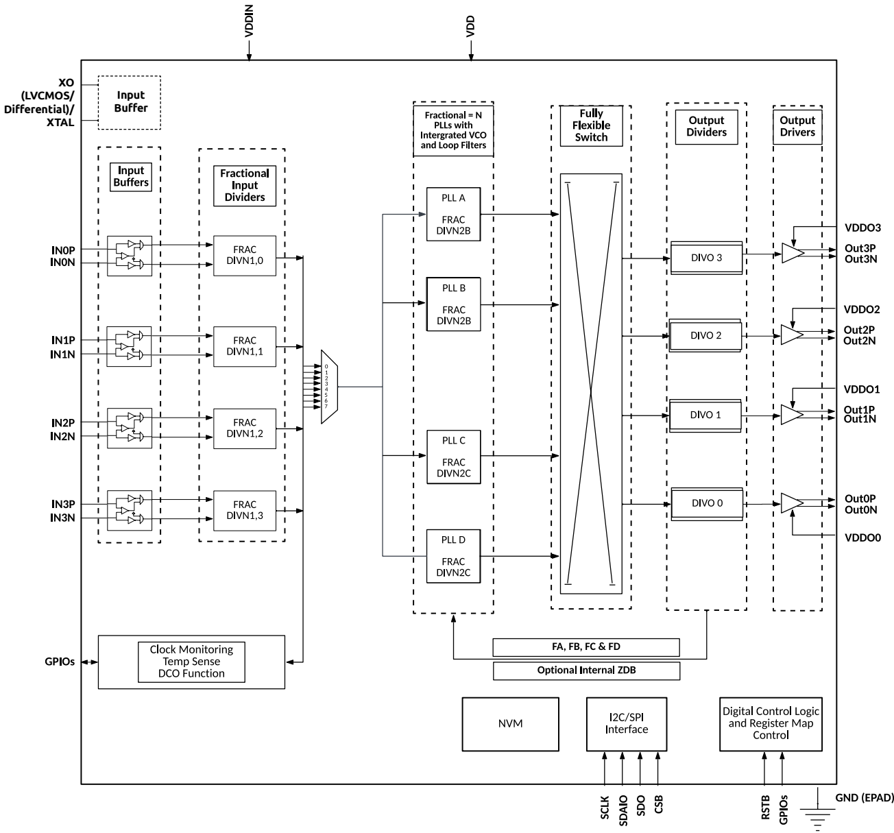
Figure 3. SiT95314 Functional Block Diagram
