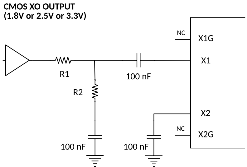
Figure 11. CMOS XO Connections
