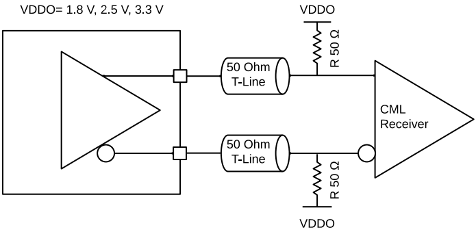
Figure 38. Output Driver used with traditional DC Coupled CML receiver
