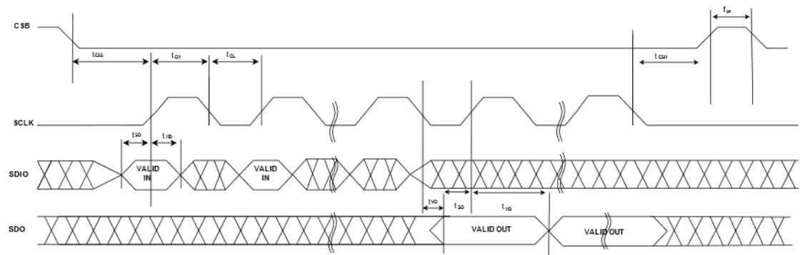
Figure 50. SPI Timing Diagram
