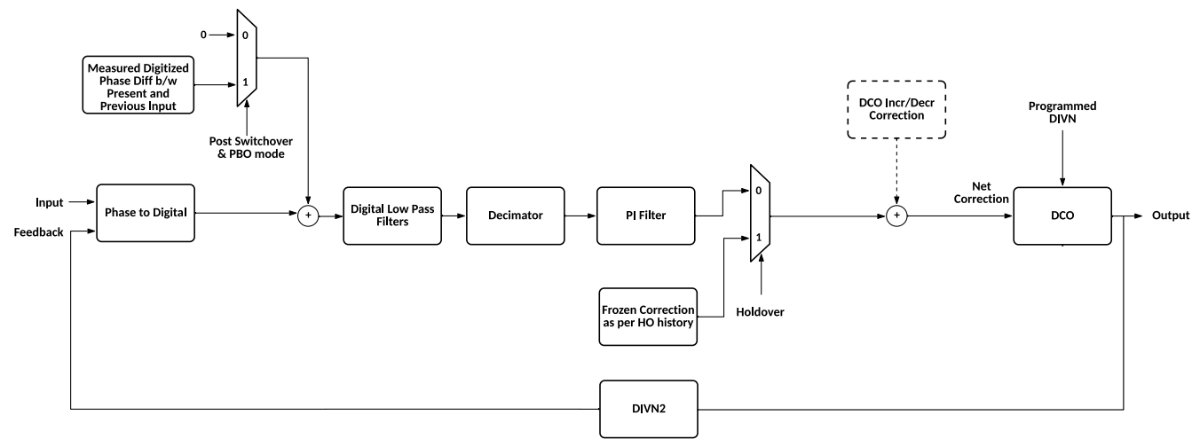
Figure 28. Basic Mode of Operation
