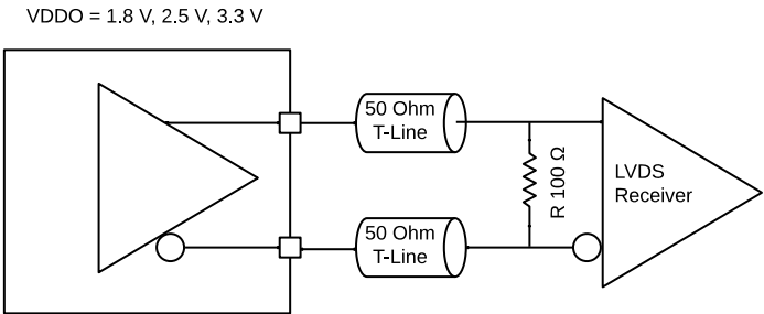
Figure 34. Output Driver used with traditional DC Coupled LVDS receiver
