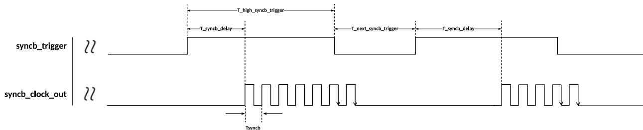
Figure 44. syncb_clock_out behavior with respect to syncb_trigger
