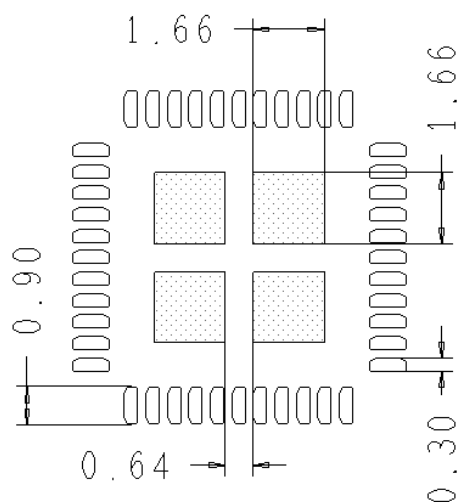
Figure 59. Solder Mask Design
