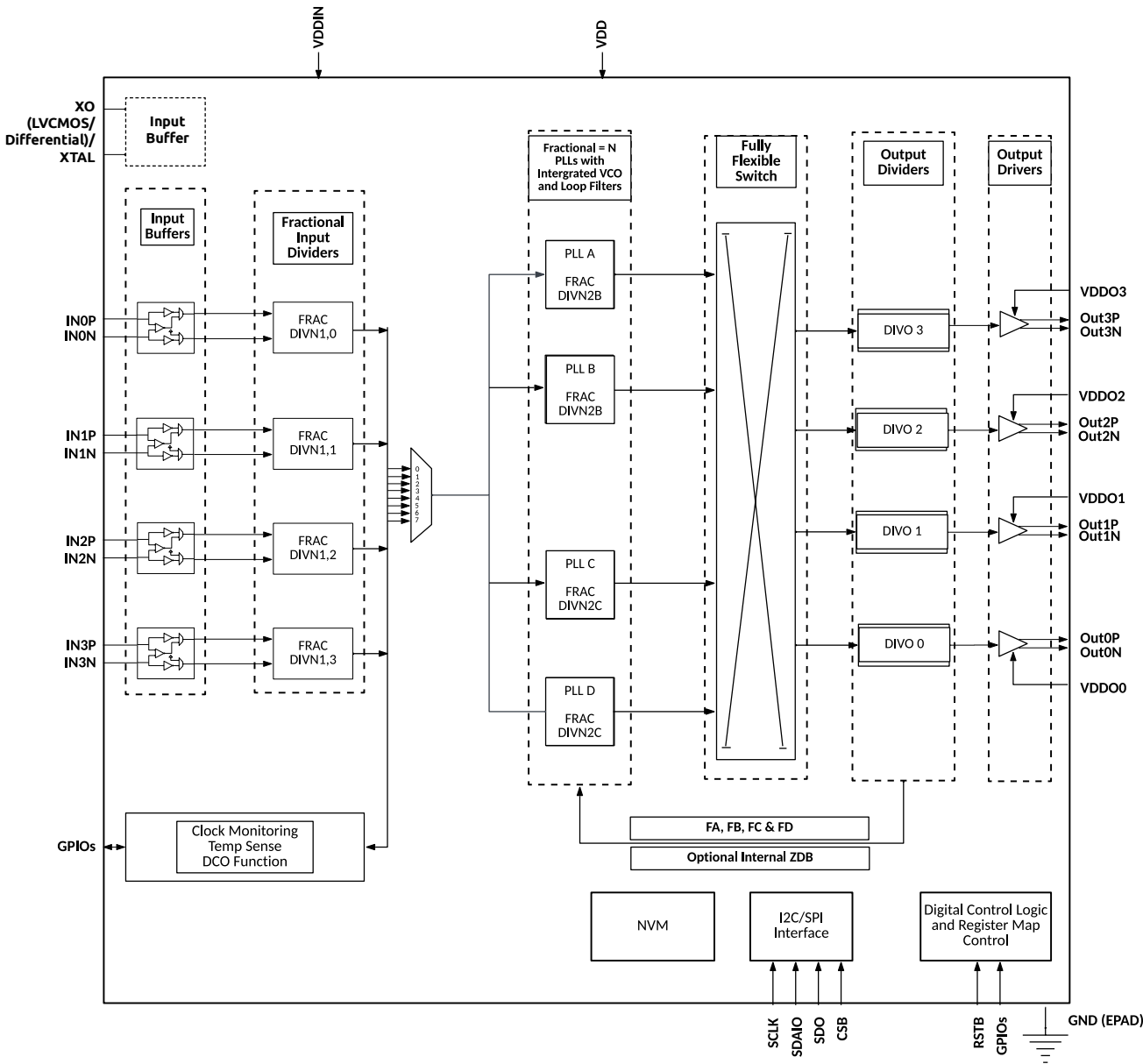
Figure 1. Functional Overview SiT95314
