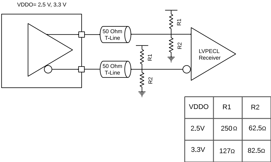
Figure 36. LVPECL Alternate DC termination: Thevenin
