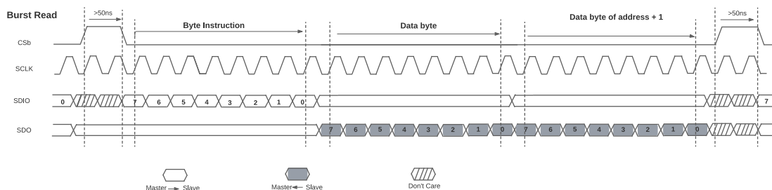
Figure 56. SPI Burst Read
