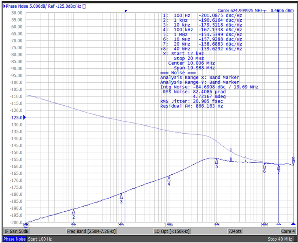
SiT95314: 625M Output (LVDS) with 96M SMA100B XO Source
