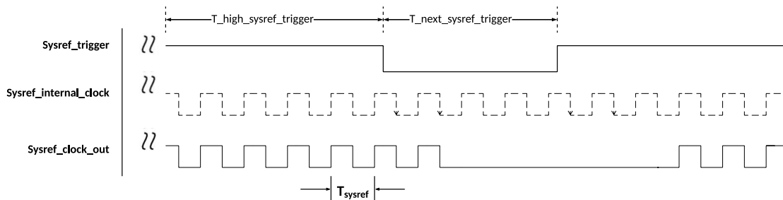
Figure 42. sysref_clock_out behavior with respect to sysref_trigger
