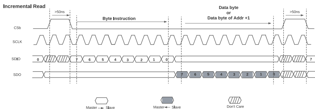
Figure 55. SPI Incremental Read
