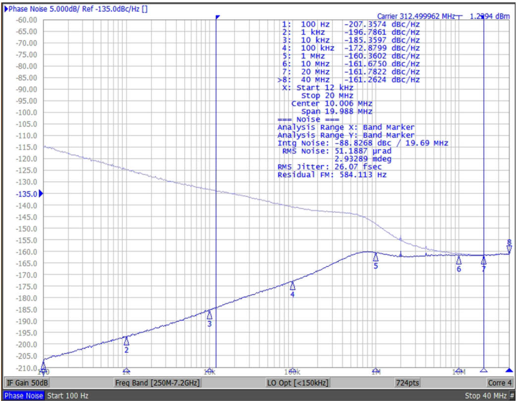
SiT95314: 312.5M Output (LVDS) with 96M SMA100B XO Source
