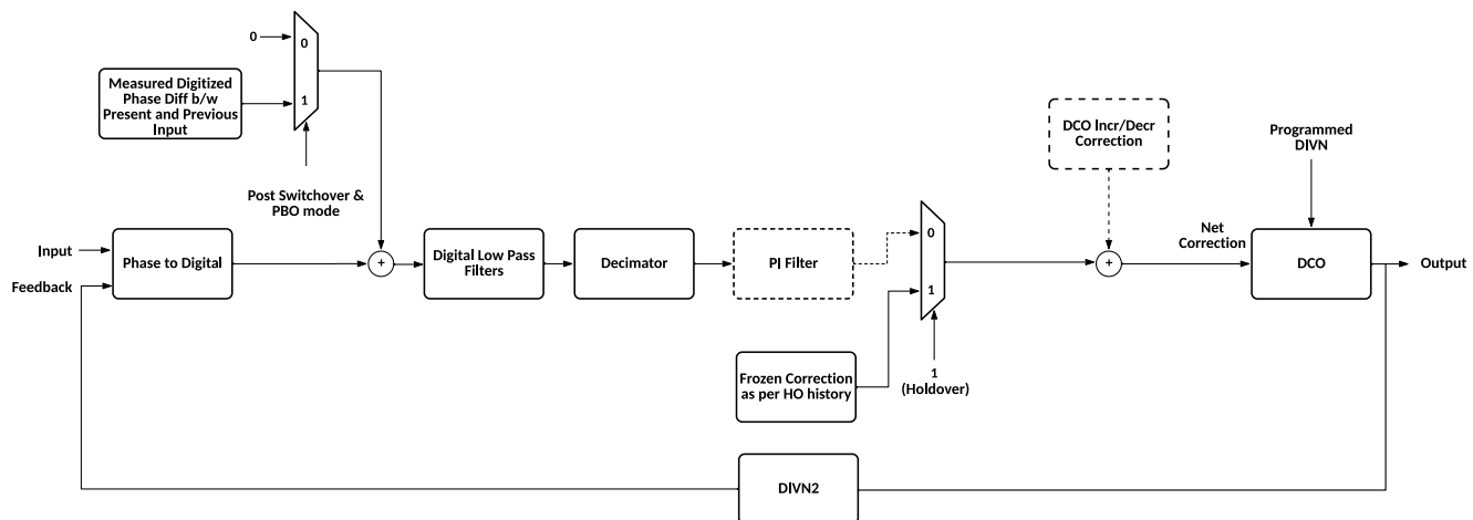
Figure 29. Holdover and Phase Build-Out Modes
