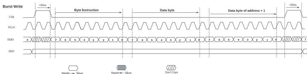
Figure 53. SPI Burst Write
