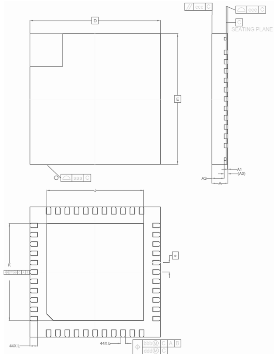
Figure 57. Package Diagram (44 QFN)
