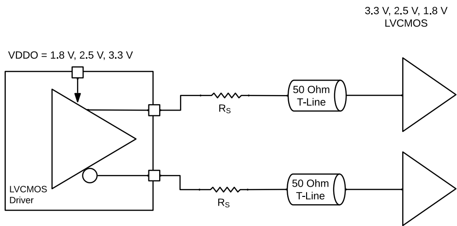
Figure 41. DC Coupled LVCMOS
