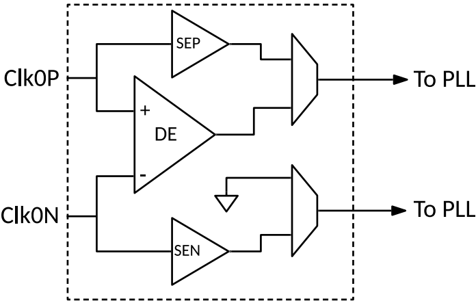
Figure 15. Input Buffer Structure
