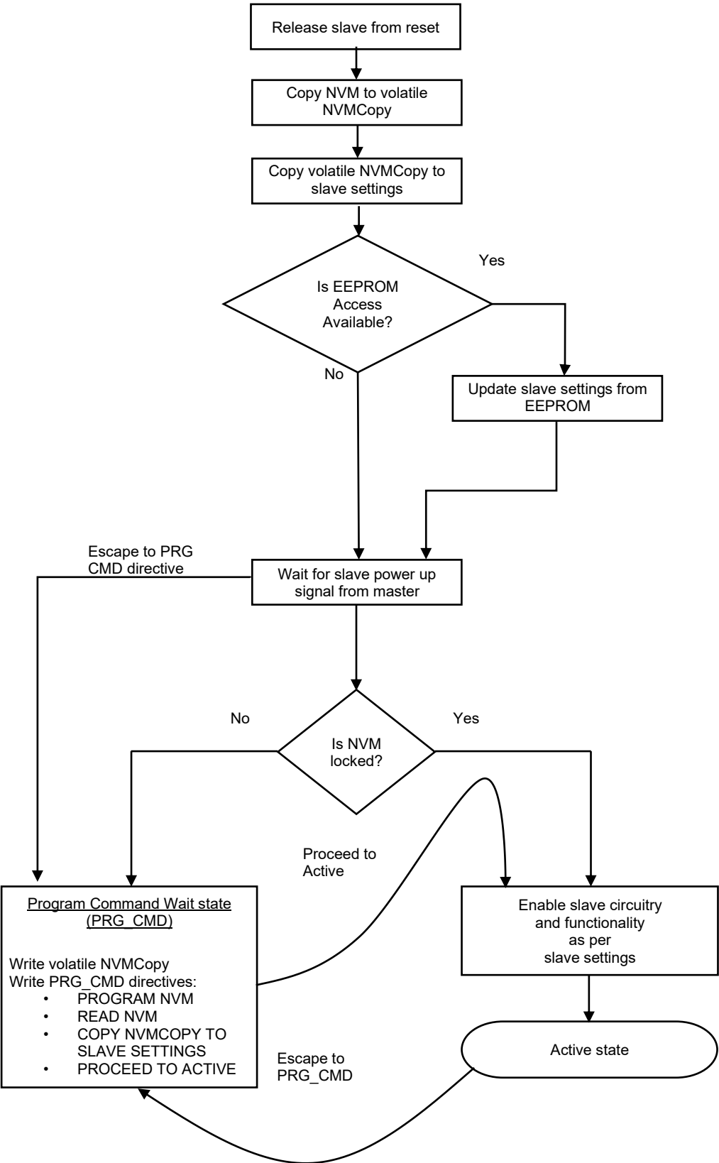
Figure 9. Slave Wake-Up Finite State Machine
