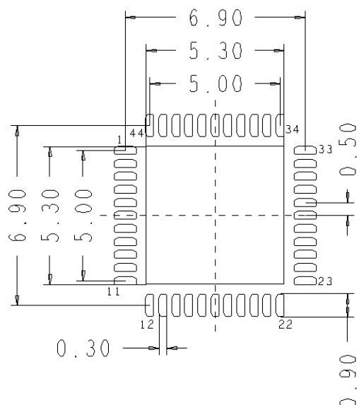
Figure 58. Land Pattern
