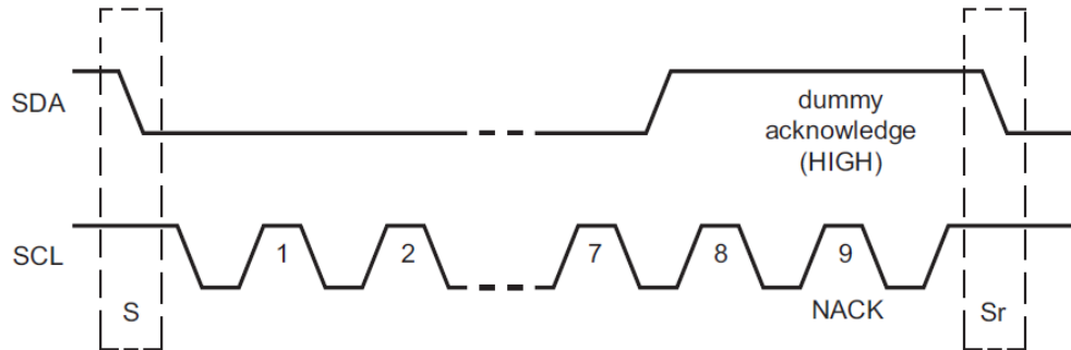
Figure 48. Start Byte Procedure
