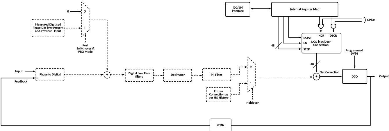
Figure 30. DCO Increment/Decrement path for inner-loop
