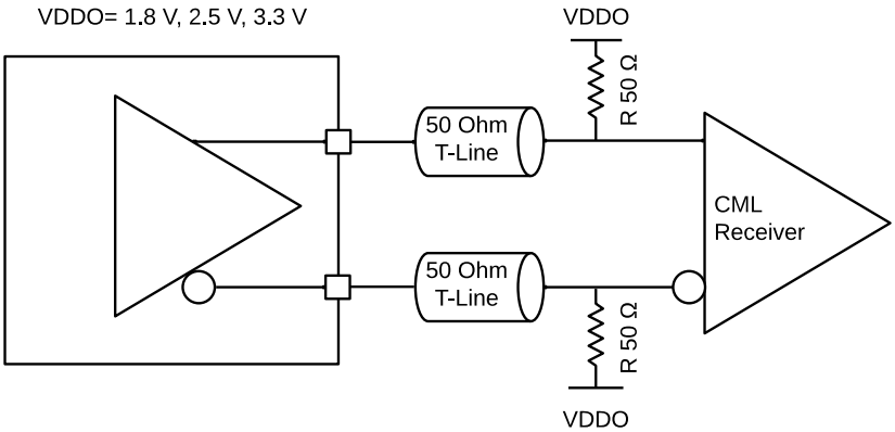
Figure 37. Output Driver used with traditional DC Coupled CML receiver
