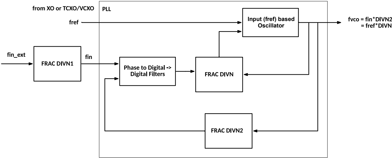
Figure 5. PLL Internals
