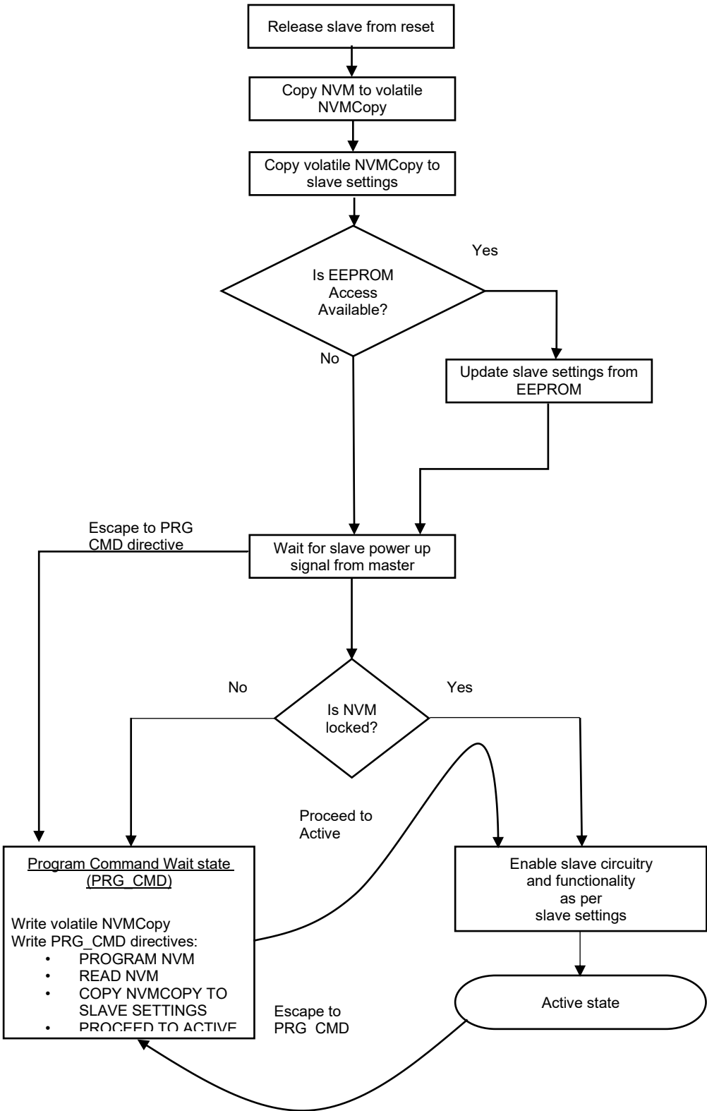
Figure 9. Slave Wake-Up Finite State Machine
