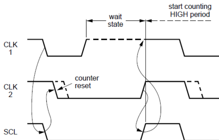
Figure 45. SCL Synchronization
