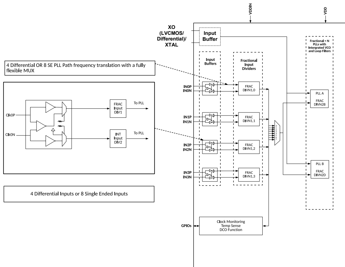
Figure 13. SiT95312 Input Slave Architecture
