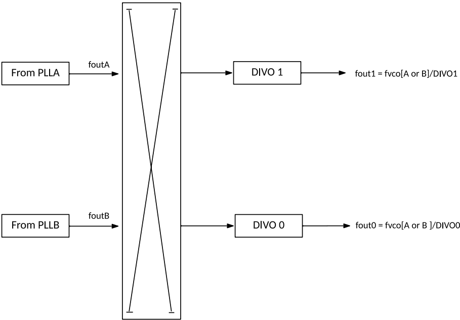
Figure 4. Output Clock Distribution
