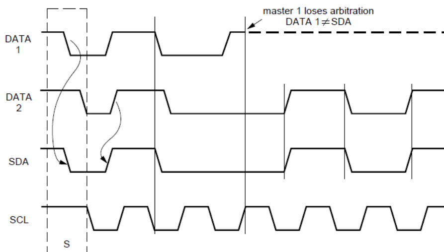
Figure 46. Arbitration
