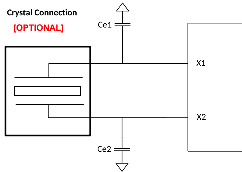
Figure 10. Crystal Connections
