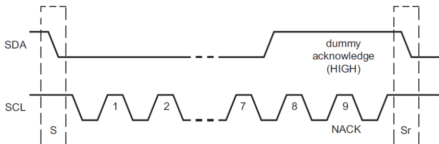
Figure 47. Start Byte Procedure
