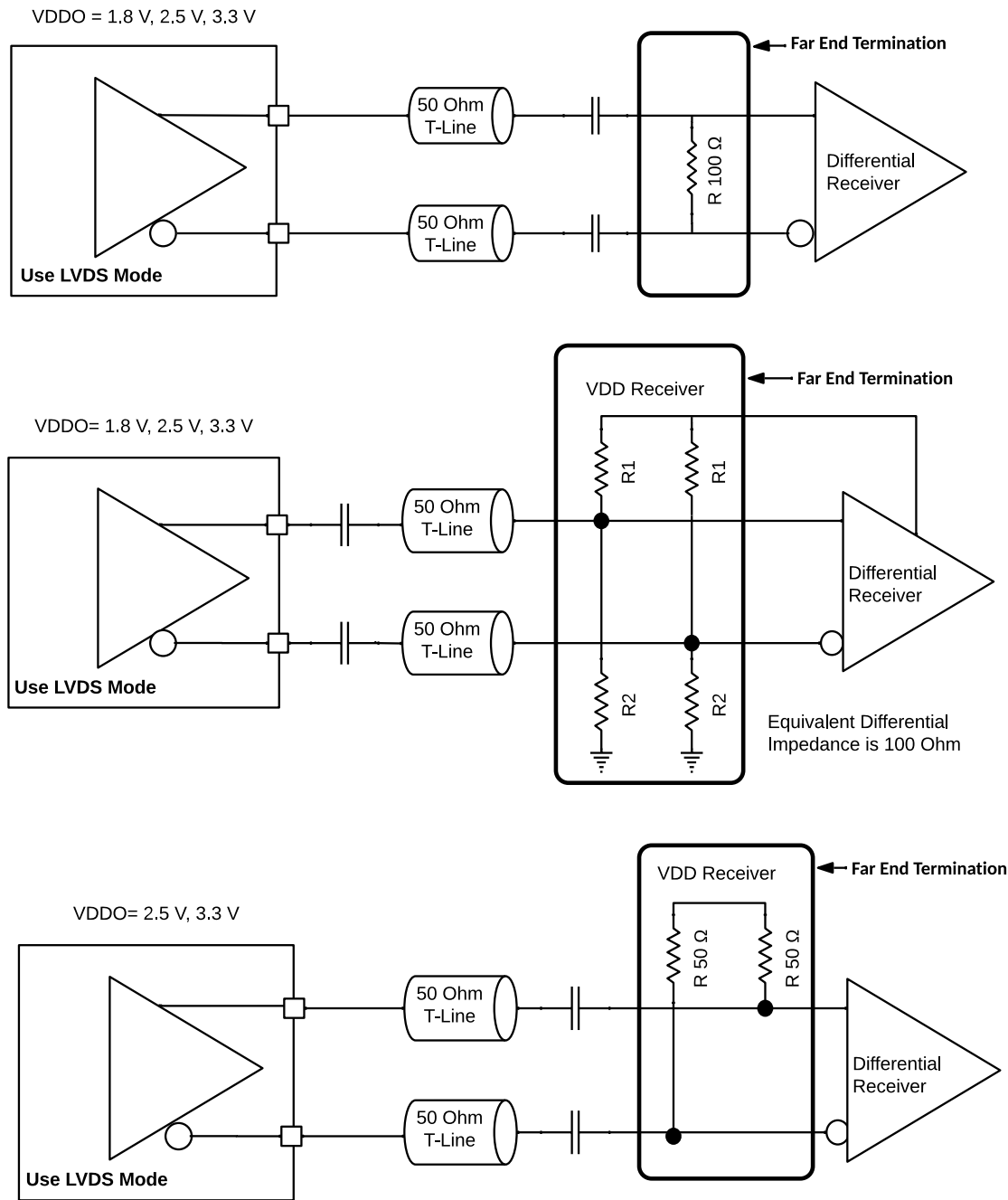
Figure 36. Output Driver used with AC Coupled terminations for various receivers
