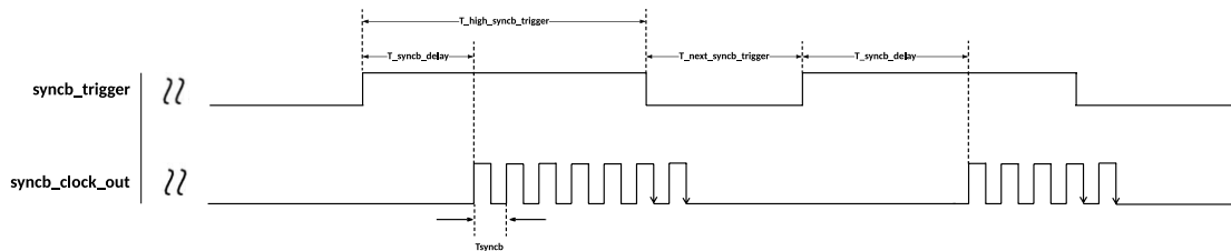
Figure 43. syncb_clock_out behavior with respect to syncb_trigger
