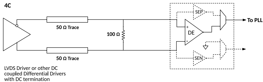
Figure 21. Interface Type IV Differential AC Coupled 4C
