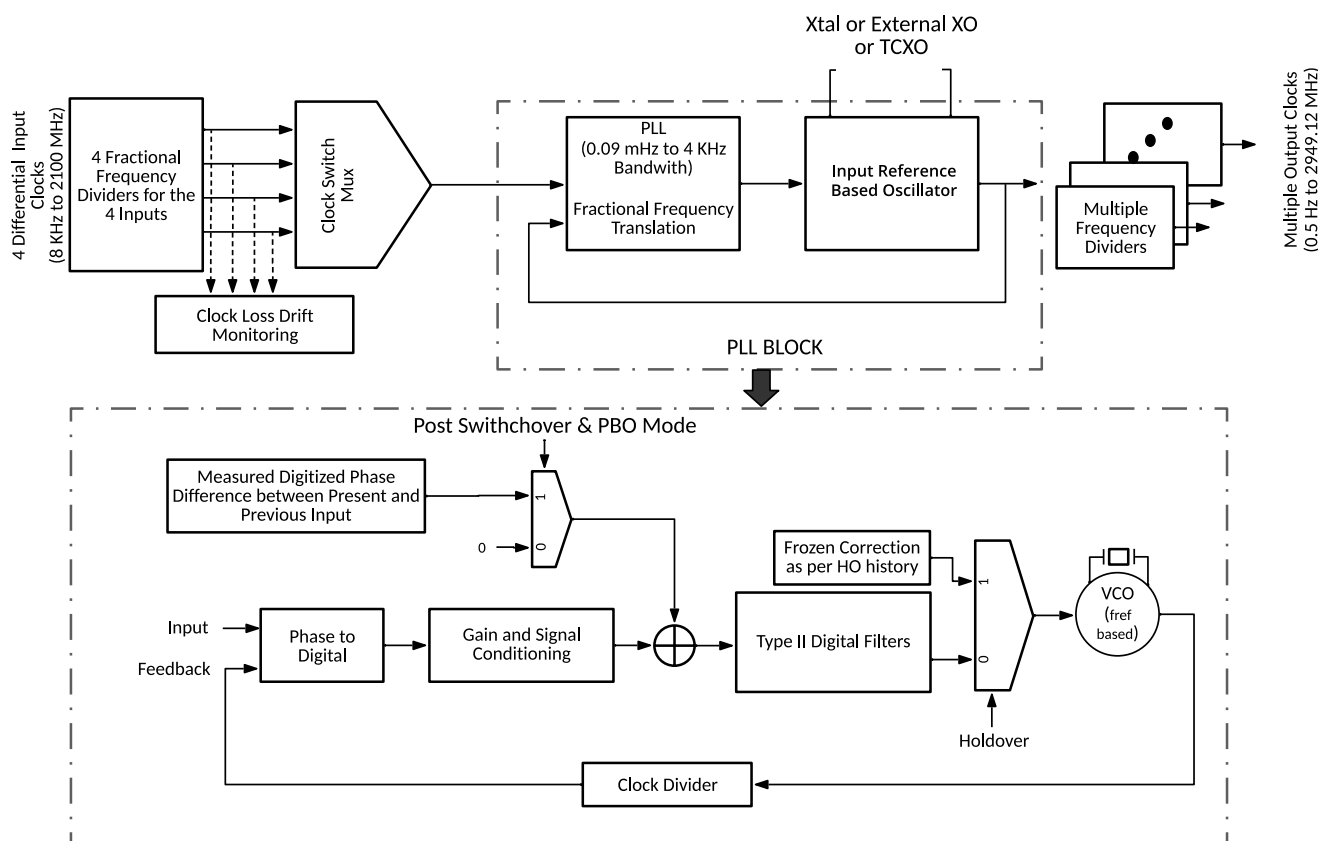
Figure 25. PLL Architecture
