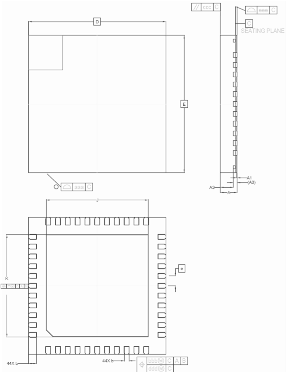
Figure 56. Package Diagram (44 QFN)
