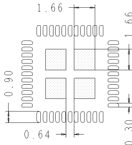
Figure 58. Solder Mask Design
