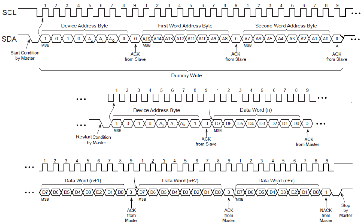
Figure 44. EEPROM read
