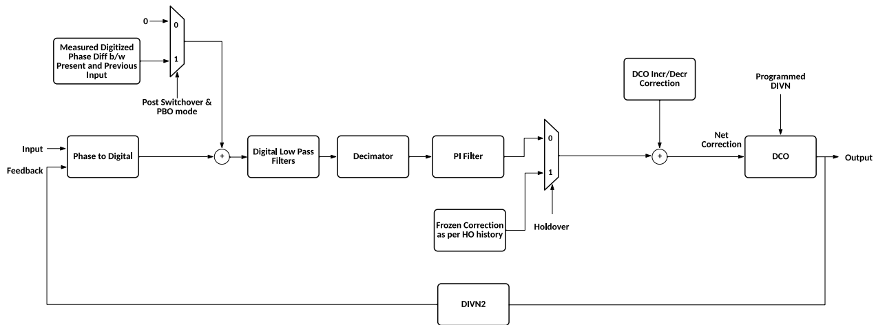
Figure 26. Basic DLPF Block Diagram
