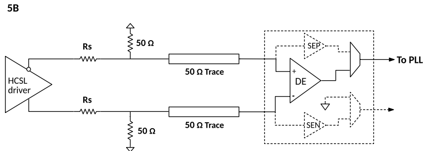
Figure 24. Interface Type V Differential DC Coupled 5B
