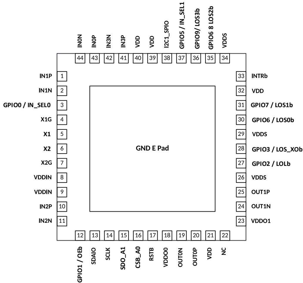
Figure 2. SiT95312 Pin Configuration
