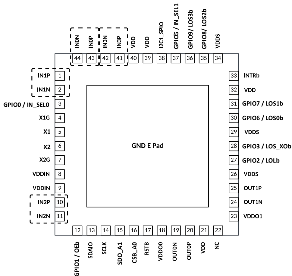
Figure 14. SiT95312 4 Diff/8 SE Input Drivers
