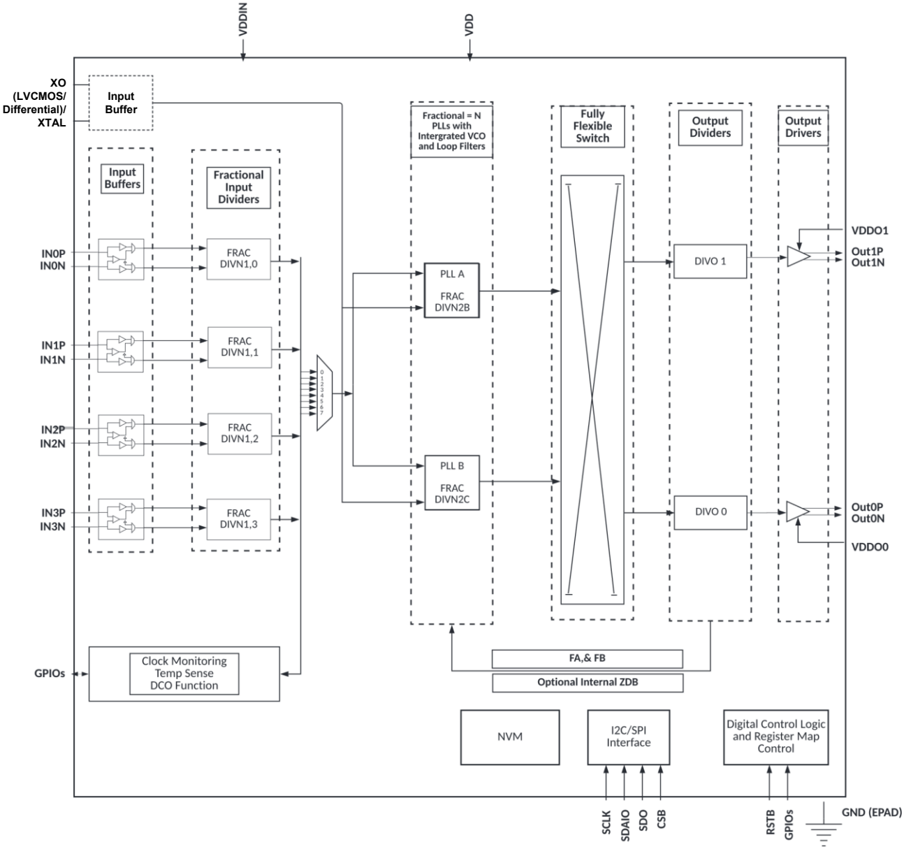
Figure 3. SiT95312 Functional Block Diagram
