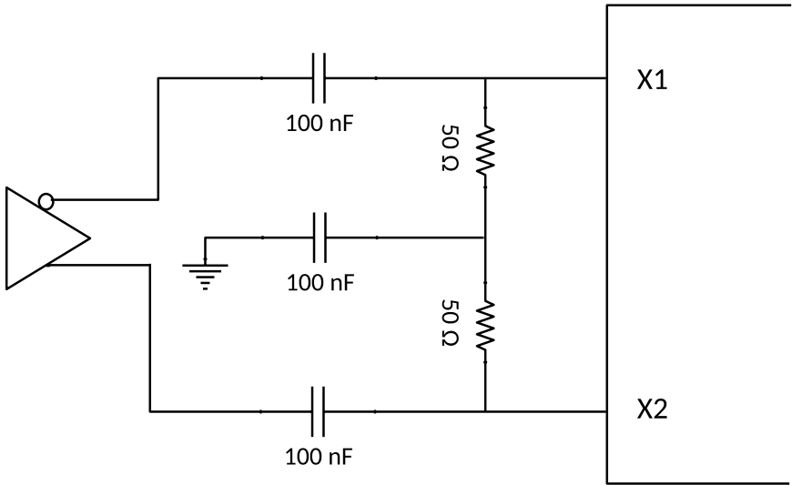
Figure 12. Differential XO Connections
