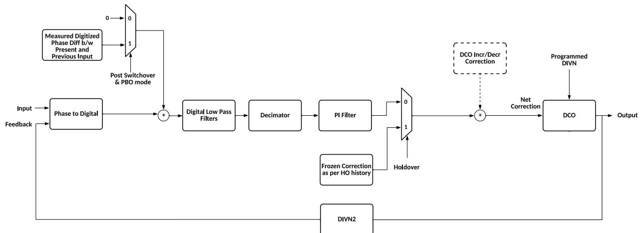
Figure 27. Basic Mode of Operation
