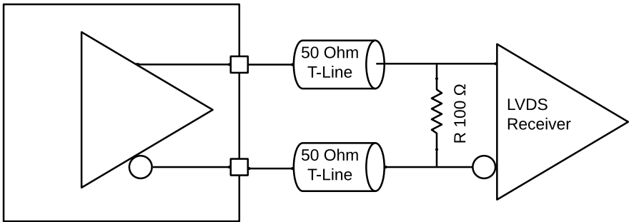
Figure 33. Output Driver used with traditional DC Coupled LVDS receiver
