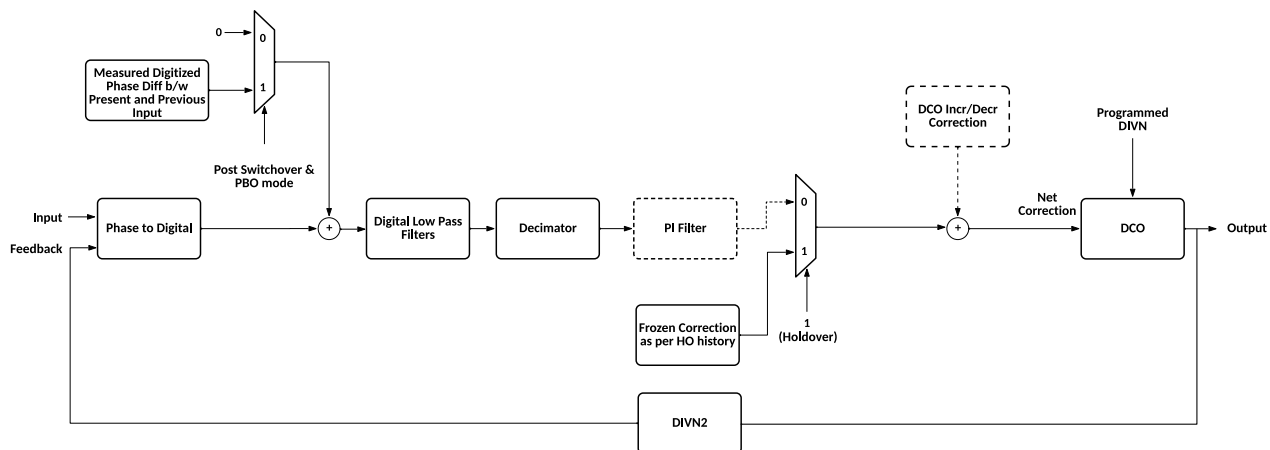
Figure 28. Holdover and Phase Build-Out Modes
