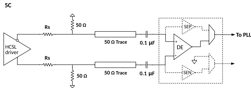
Figure 25. Interface Type V Differential AC Coupled 5C
