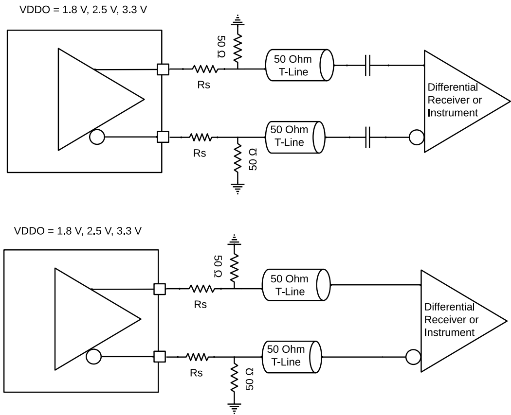
Figure 38. Output Driver used with traditional HCSL receiver
