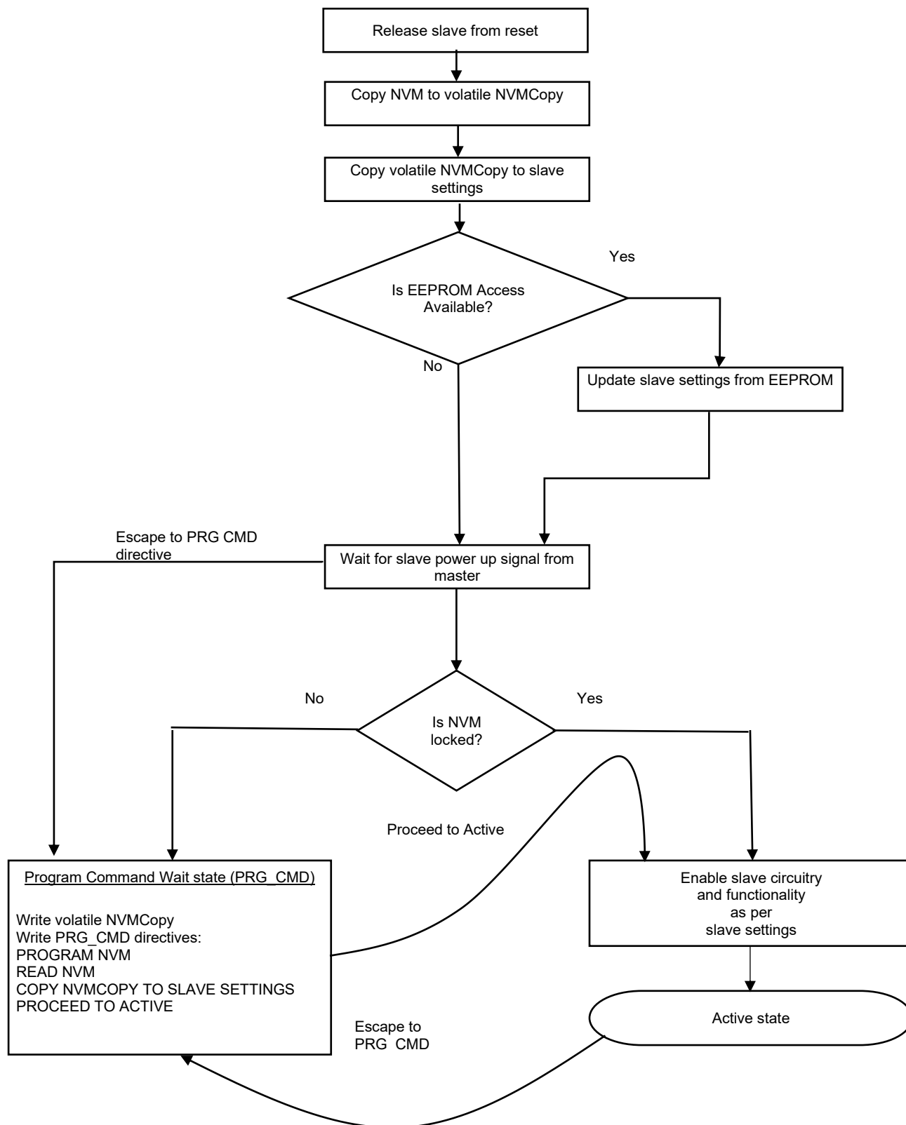
Figure 9. Slave Wake-Up Finite State Machine
