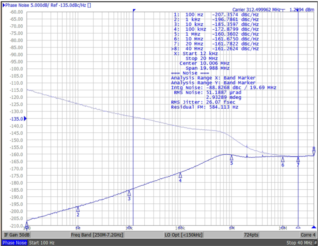
SiT95211: 312.5M Output (LVDS) with 96M SMA100B XO Source
