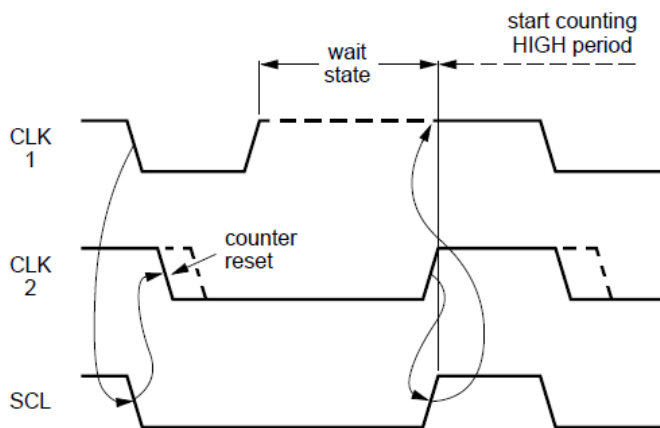
Figure 45. SCL Synchronization
