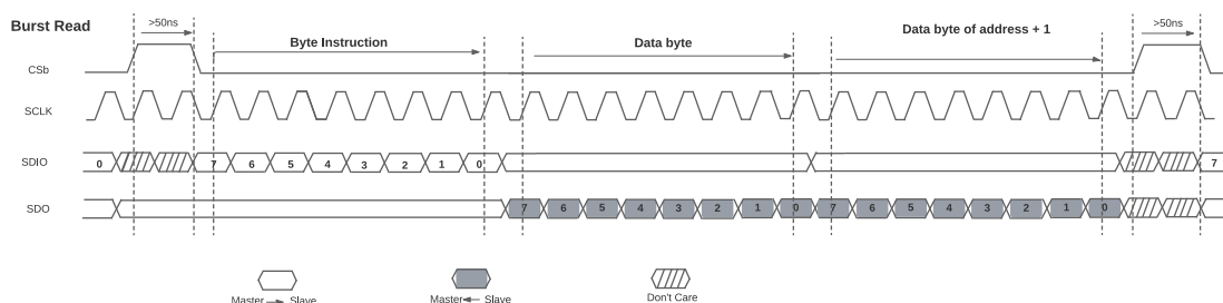
Figure 55. SPI Burst Read
