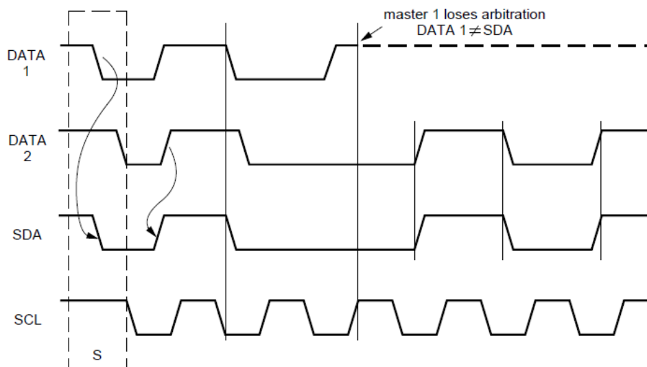
Figure 46. Arbitration
