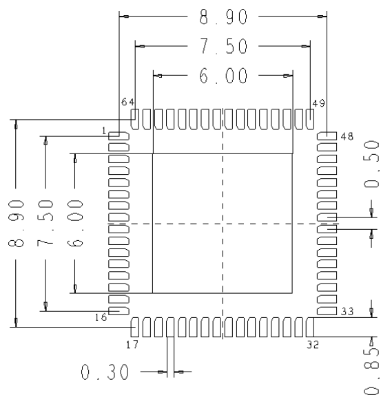
Figure 57. Land Pattern
