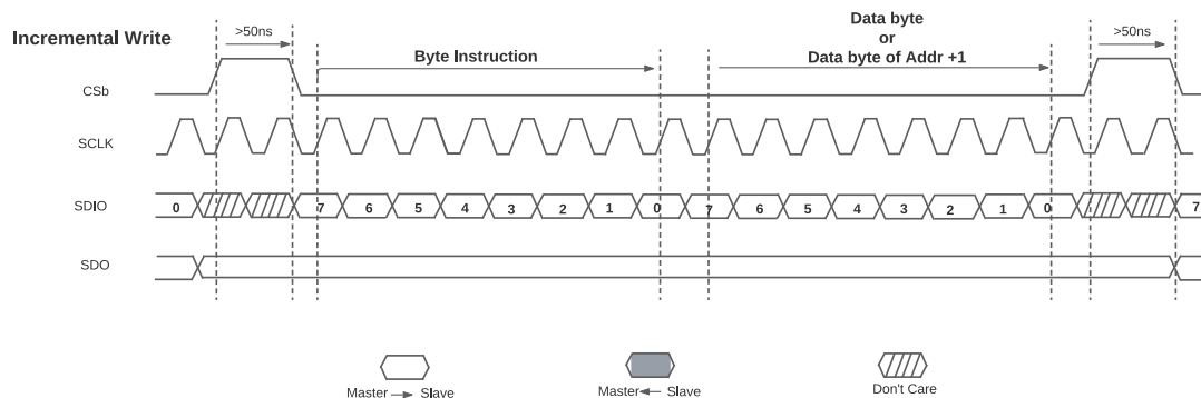
Figure 51. SPI Incremental Write
