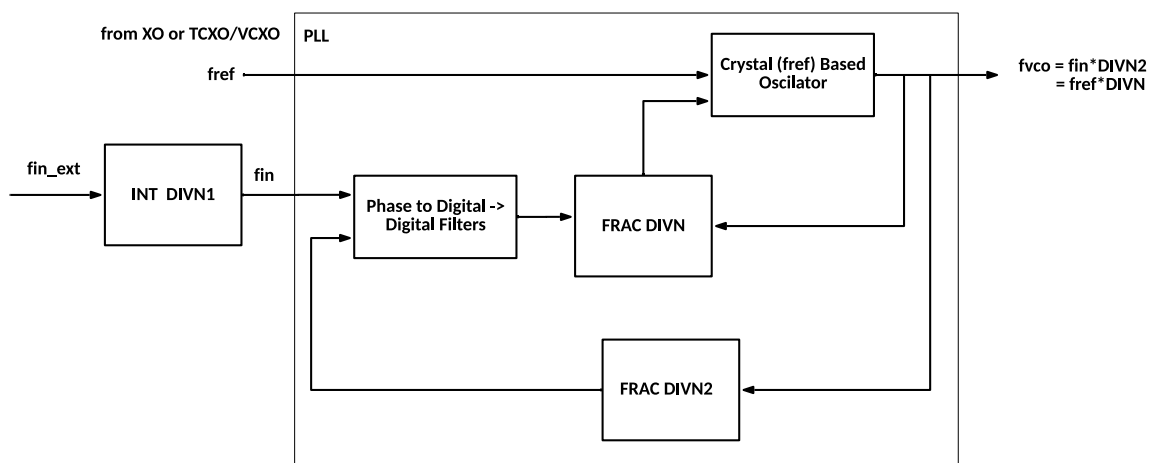
Figure 5. PLL Internals
