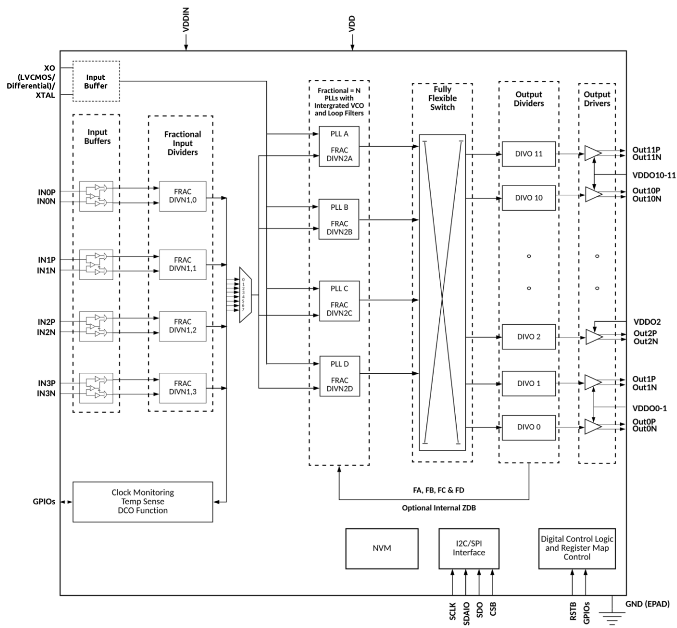
Figure 1. Functional Overview
