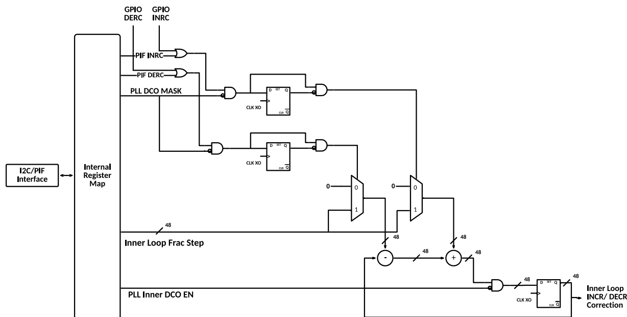
Figure 30. Architecture of the Inner-Loop Increment/Decrement path
