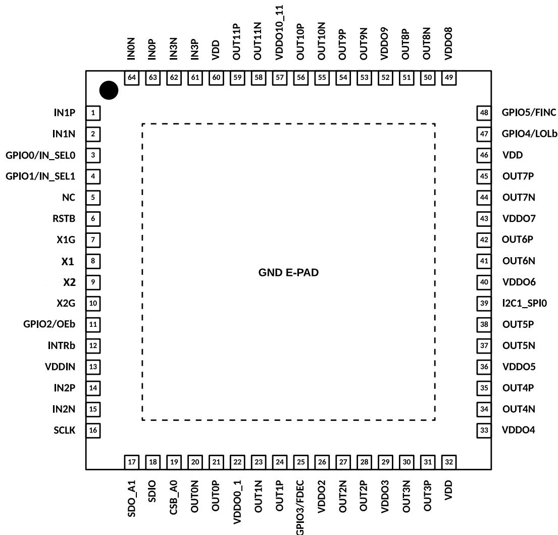
Figure 2. SiT95211 Pin Configuration
