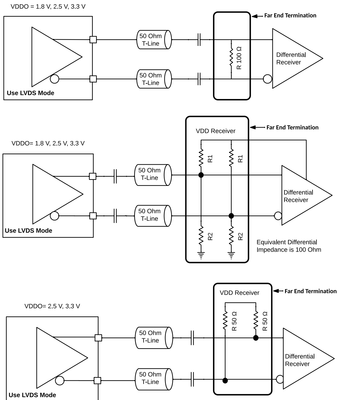
Figure 36. LVDS Output Driver used with AC Coupled terminations for various receivers
