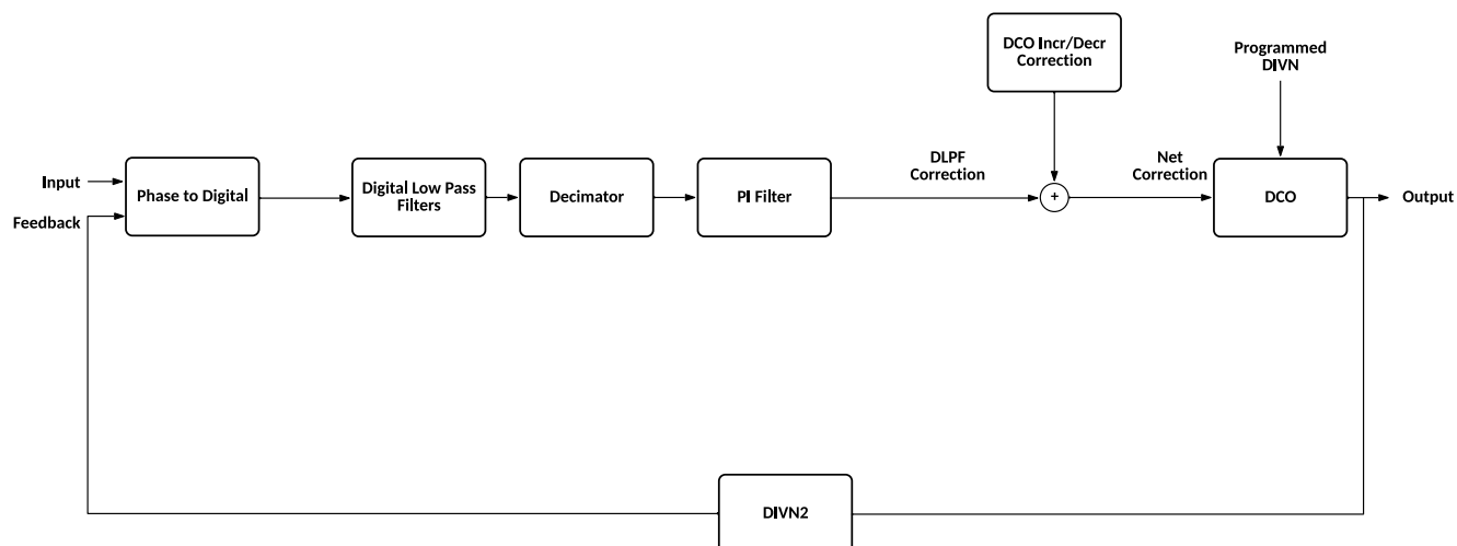
Figure 27. Basic DLPF Block Diagram
