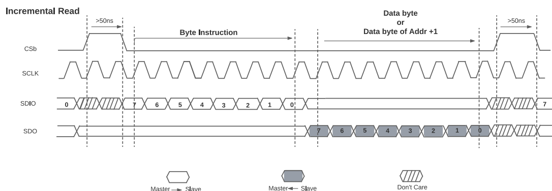
Figure 54. SPI Incremental Read
