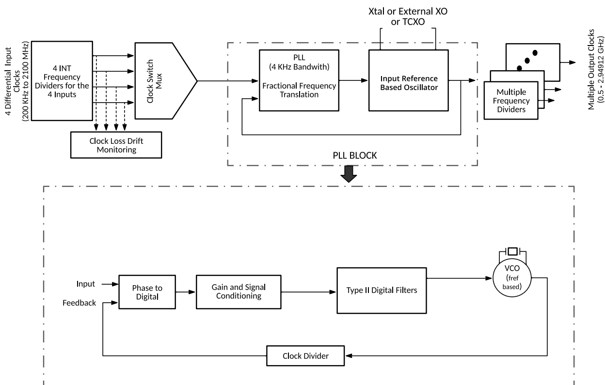
Figure 26. PLL Architecture
