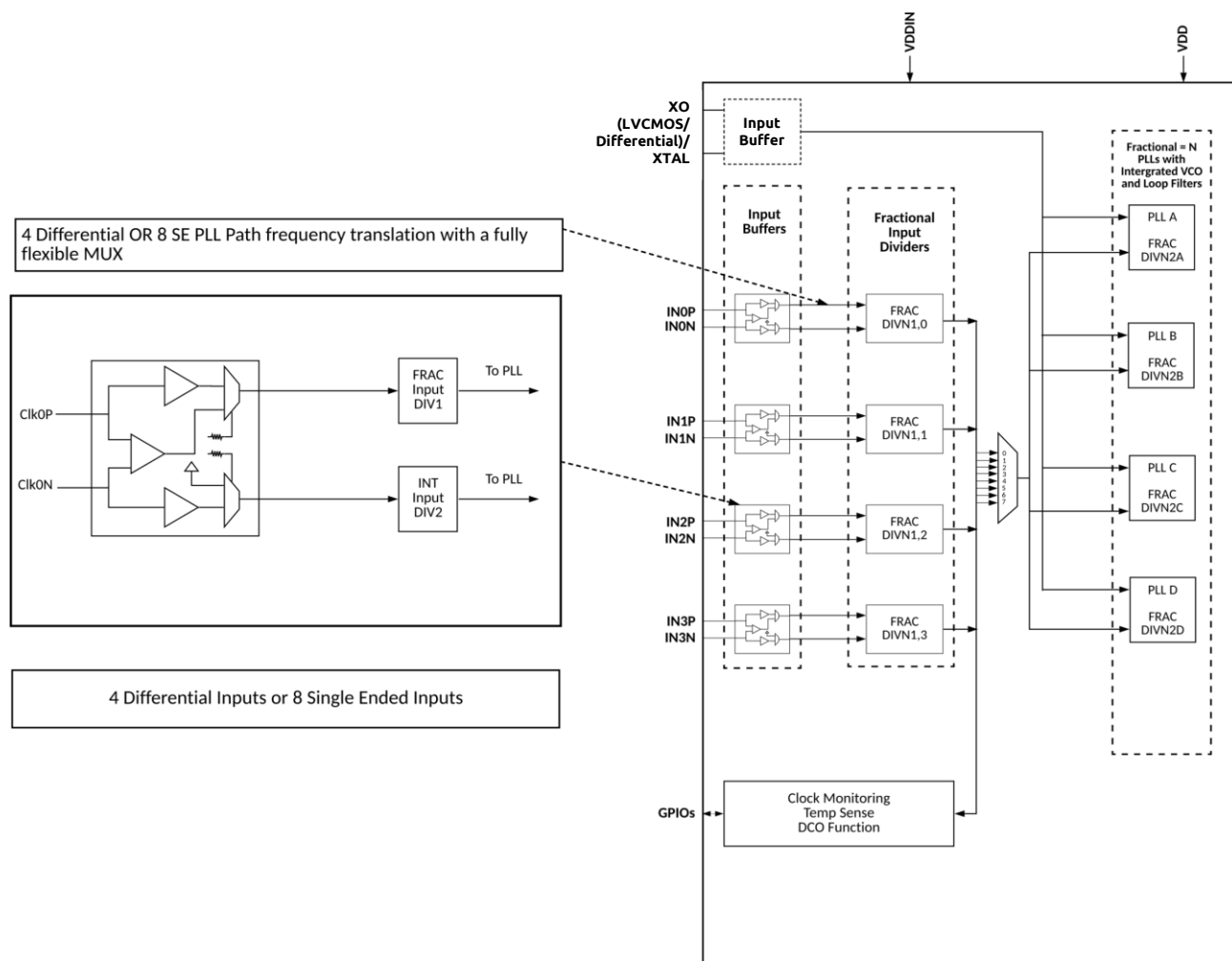
Figure 13. SiT95211 Input Slave Architecture
