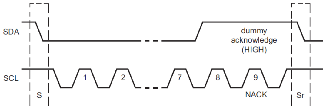
Figure 47. Start Byte Procedure
