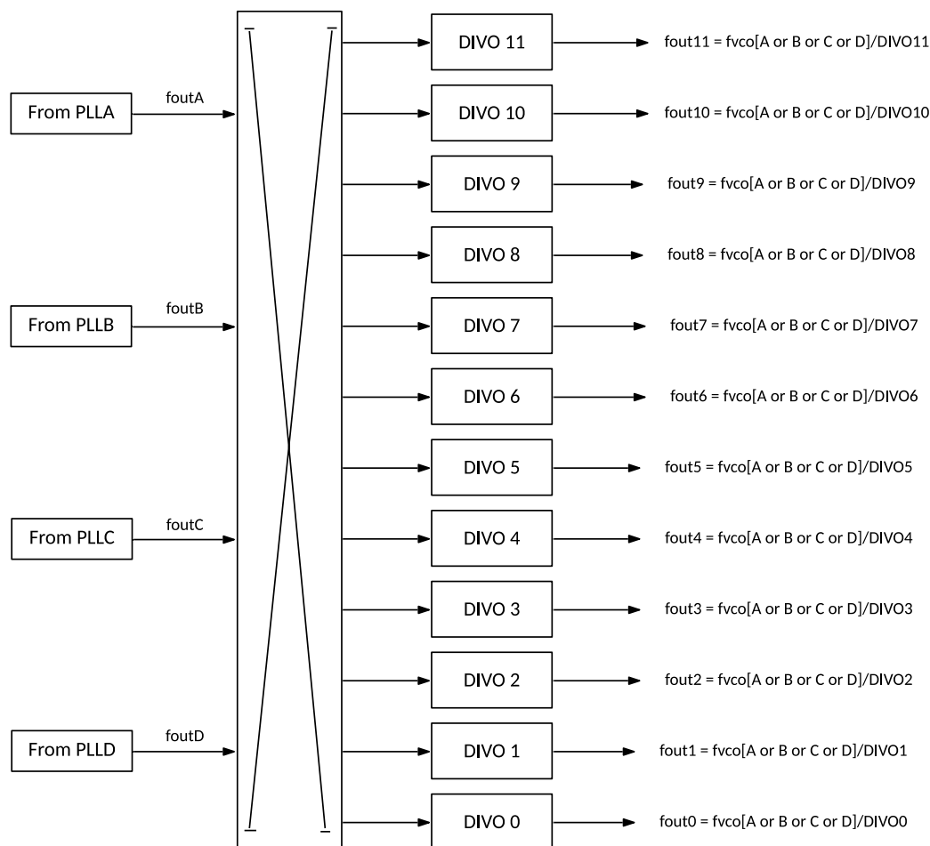
Figure 4. Output Clock Distribution
