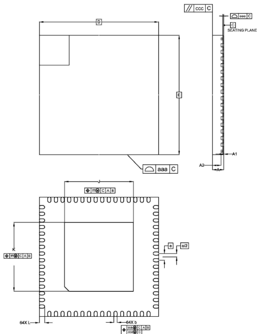
Figure 56. Package Diagram – 64 pin QFN
