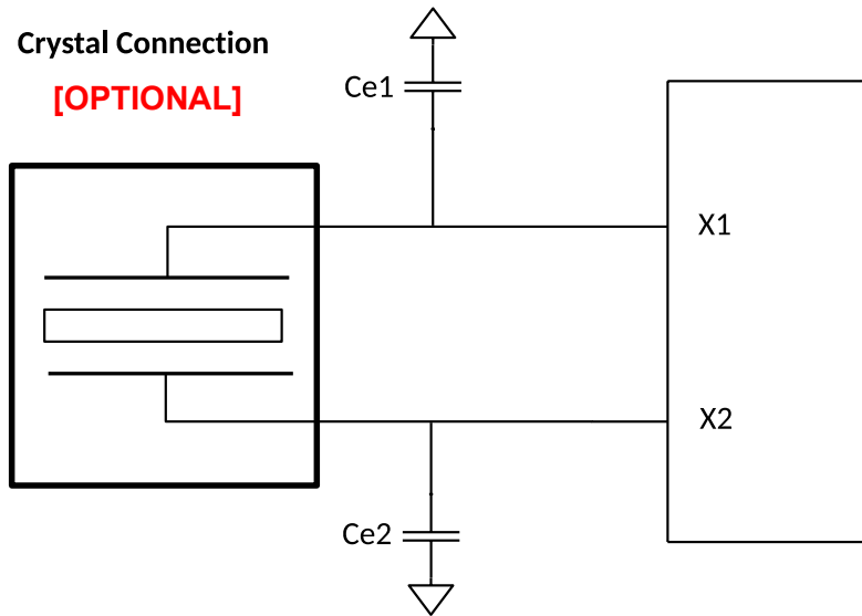
Figure 10. Crystal Connections
