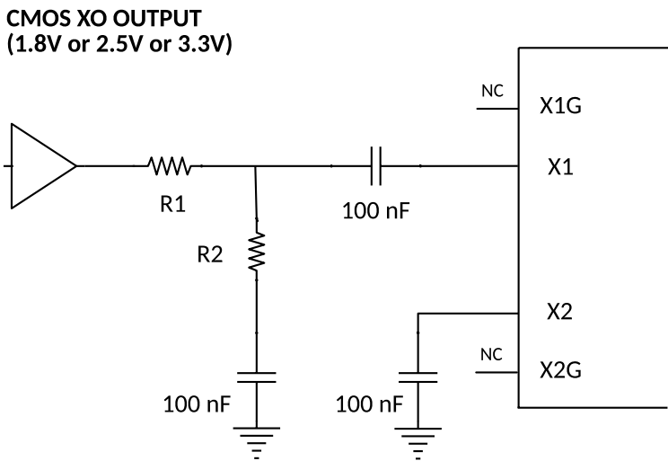
Figure 11. CMOS XO Connections
