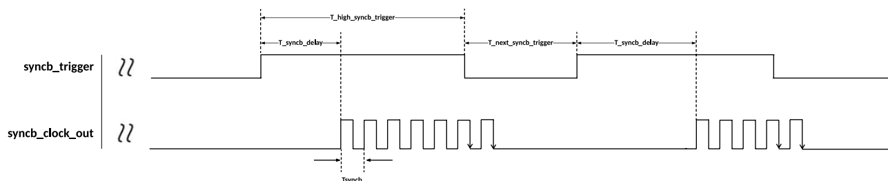
Figure 43. syncb_clock_out behavior with respect to syncb_trigger
