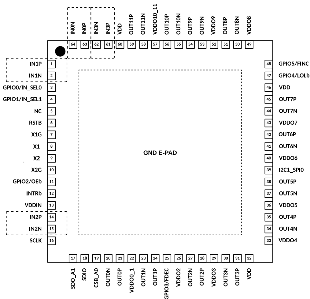
Figure 14. 4 Differential/ 8 Single Ended Inputs
