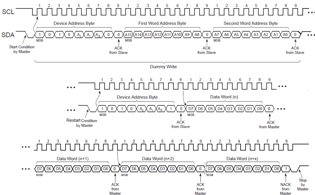
Figure 44. EEPROM read
