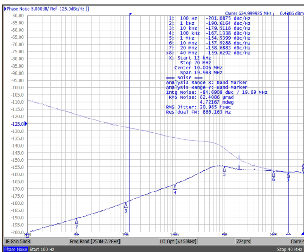
SiT95211: 625M Output (LVDS) with 96M SMA100B XO Source
