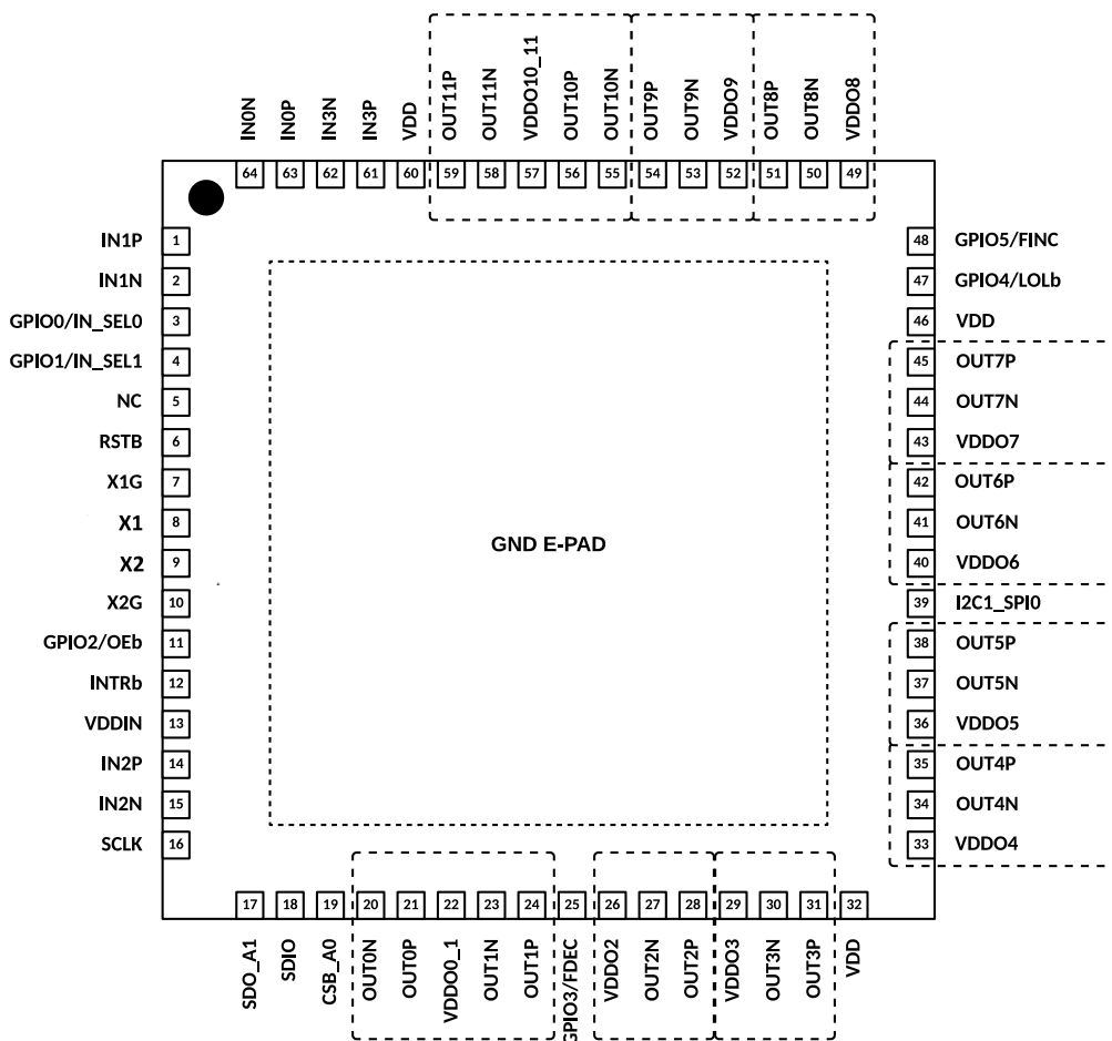
Figure 31. SiT95211 Output Driver
