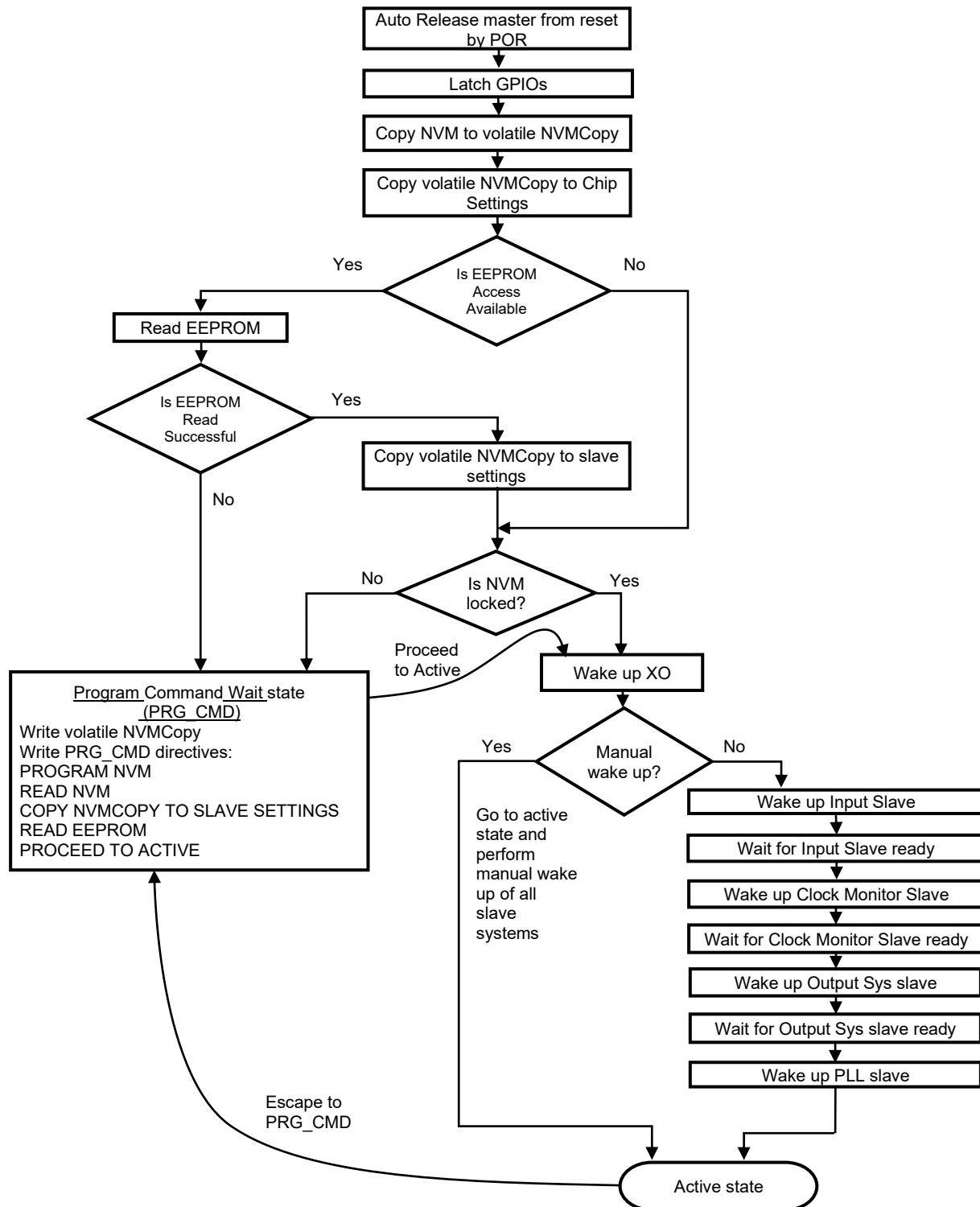
Figure 8. Master Wake-Up Finite State Machine
