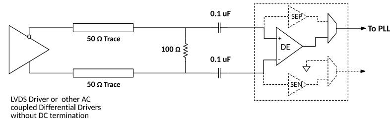
Figure 20. Interface Type IV Differential AC Coupled 4B
