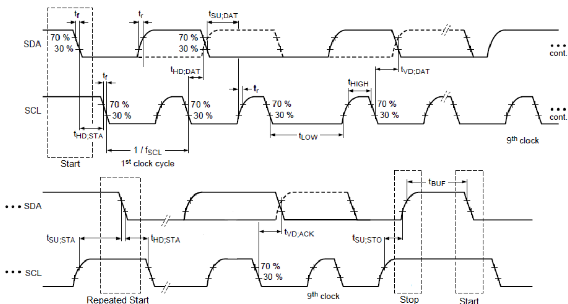
Figure 48. I2C Timing Waveform
