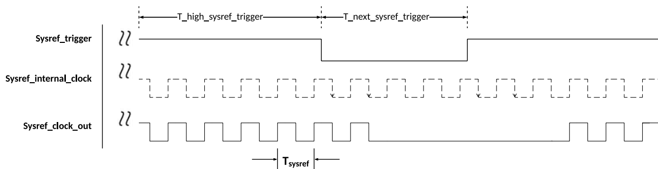
Figure 41. sysref_clock_out behaviour with respect to sysref_trigger
