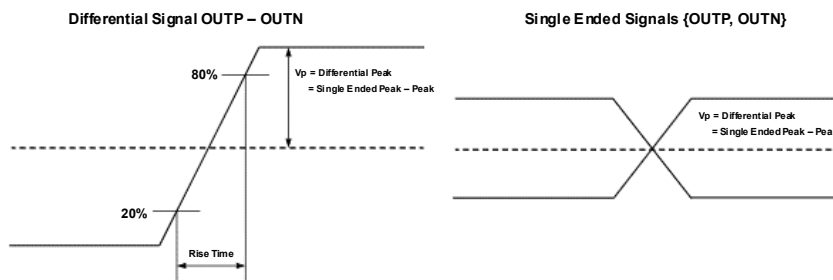
Figure 32. Waveform Convention
