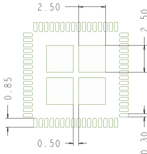
Figure 58. Solder Mask Design
