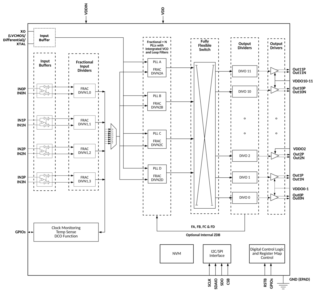
Figure 3. SiT95211 Functional Block Diagram
