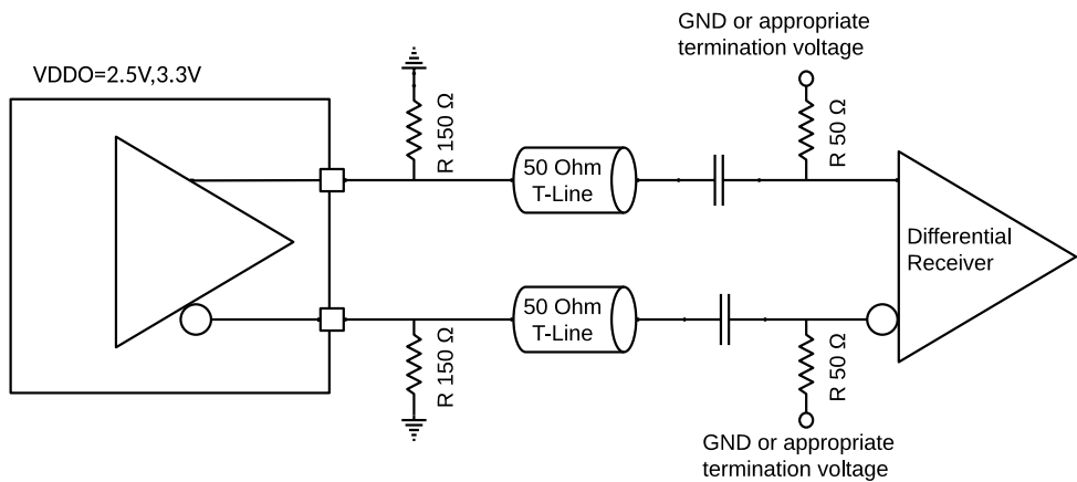
Figure 39. Alternate AC Coupled HCSL with DC Coupled resistors on Chip side
