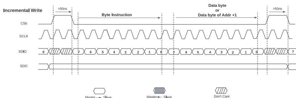
Figure 51. SPI Incremental Write
