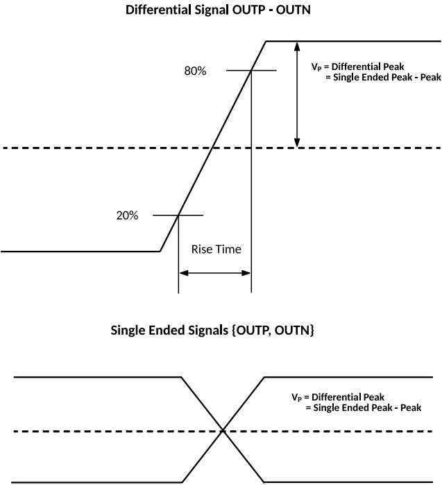
Figure 32. Waveform Convention
