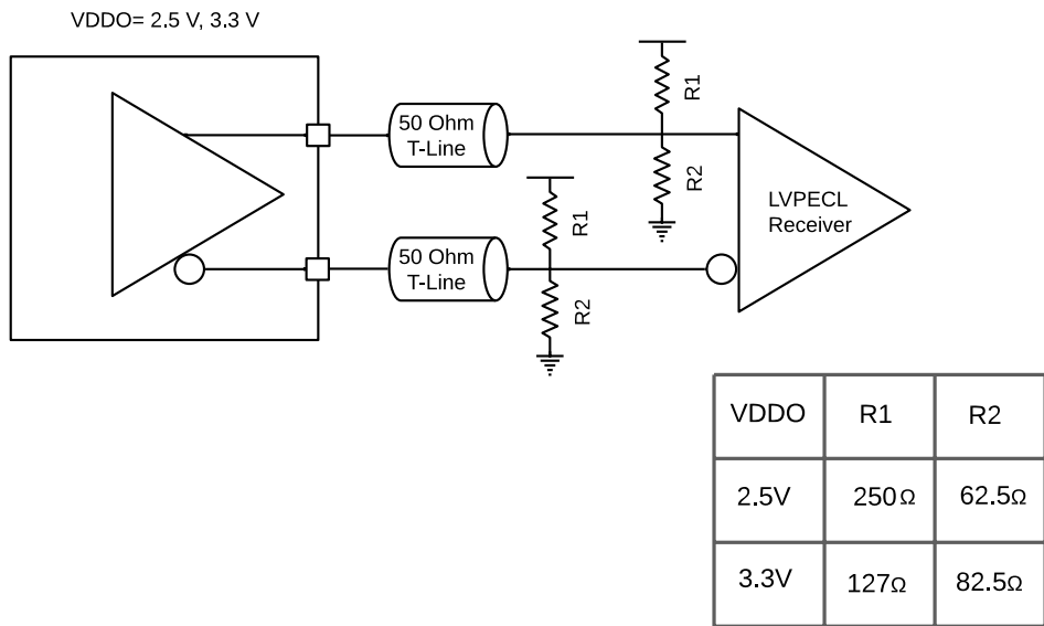
Figure 35. LVPECL Alternate DC termination: Thevenin
