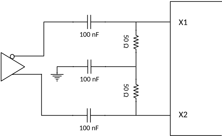
Figure 12. Differential XO Connections
