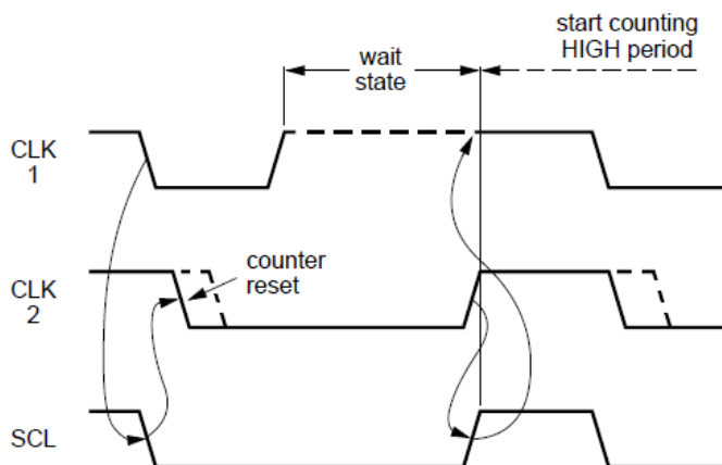
Figure 45. SCL Synchronization
