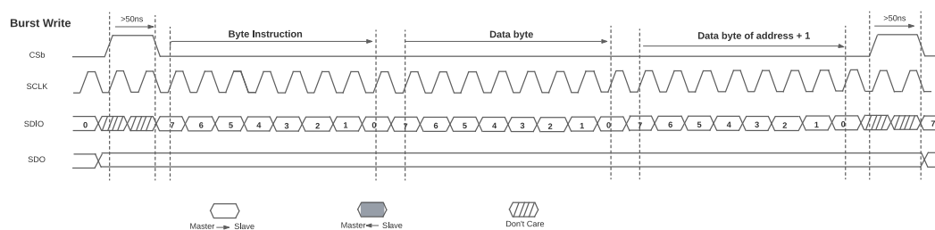
Figure 52. SPI Burst Write
