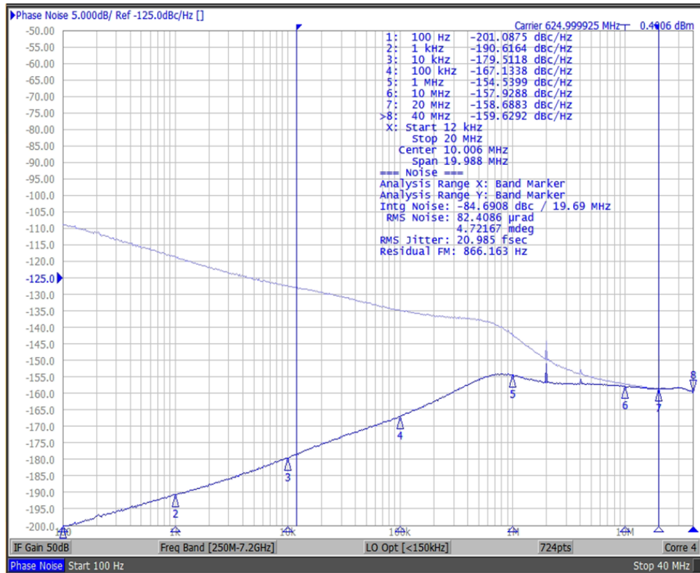
SiT95210: 625M Output (LVDS) with 96M SMA100B XO Source
