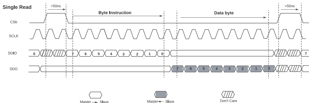
Figure 53. SPI Single Read
