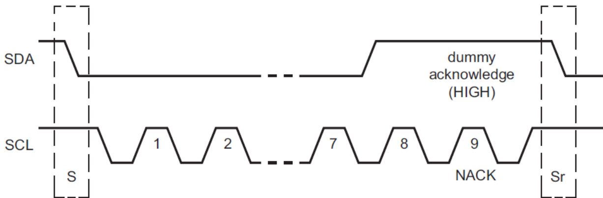
Figure 47. Start Byte Procedure
