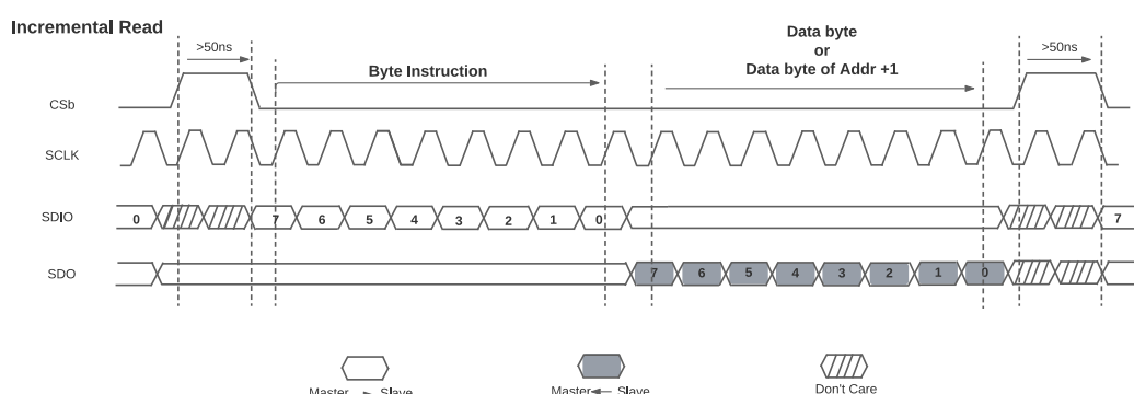
Figure 54. SPI Incremental Read
