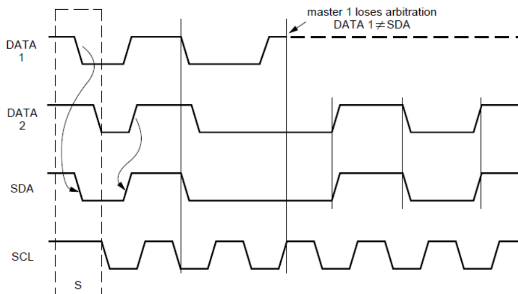
Figure 46. Arbitration
