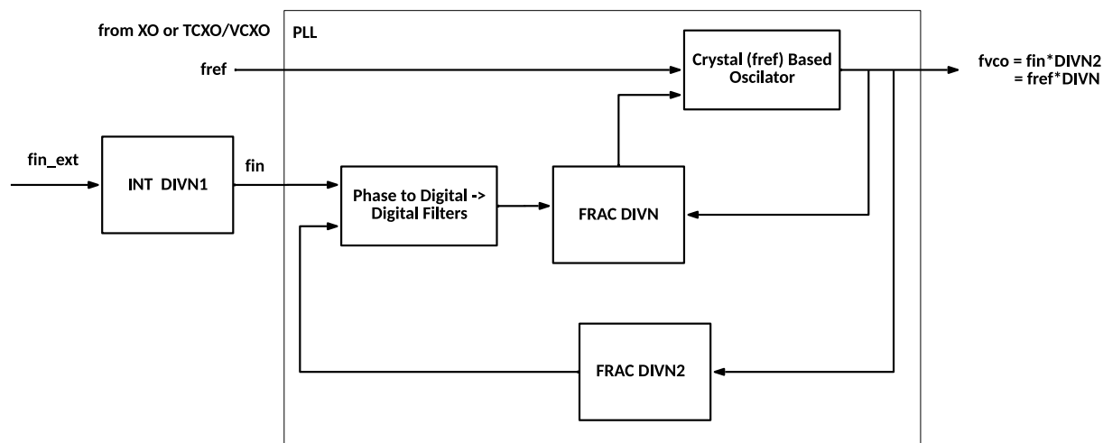
Figure 5. PLL Internals
