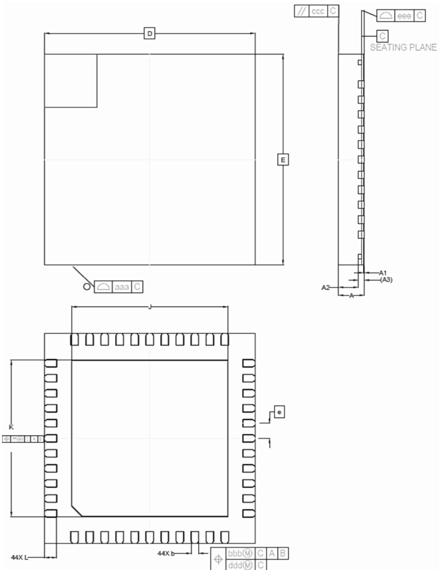
Figure 56. Package Diagram (44 QFN)
