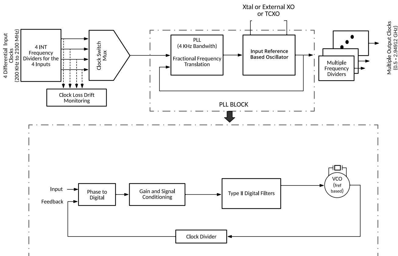
Figure 26. PLL Architecture
