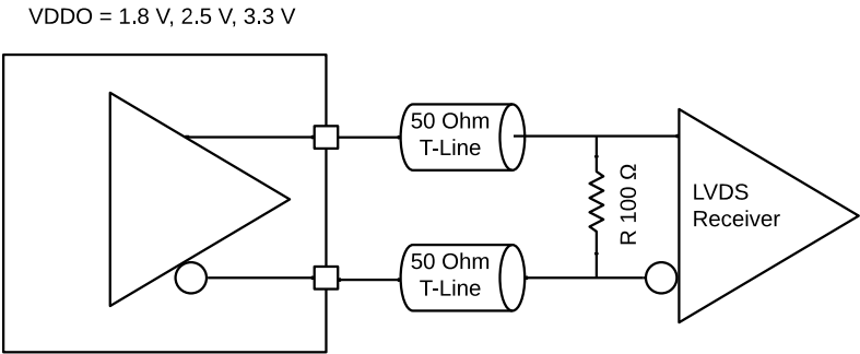
Figure 33. Output Driver used with traditional DC Coupled LVDS receiver
