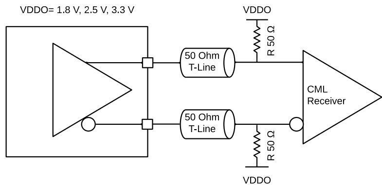
Figure 37. Output Driver used with traditional DC Coupled CML receiver
