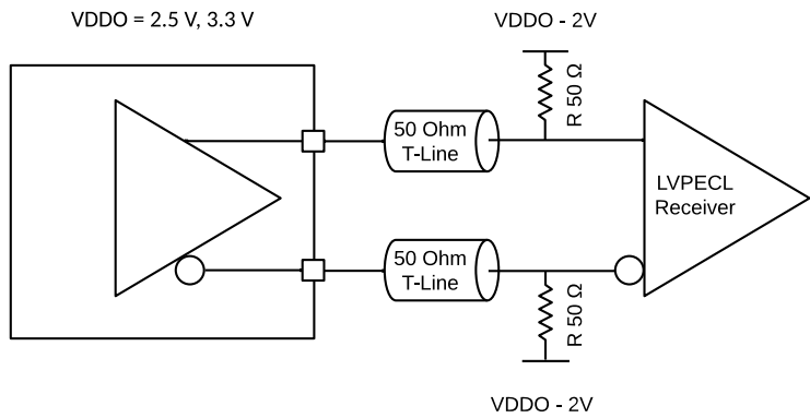
Figure 34. Output Driver used with traditional LVPECL DC Coupled receiver (DC Termination to VDDO - 2V)
