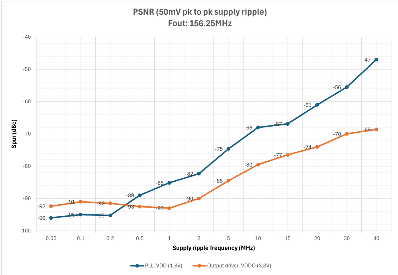
SiT95210 156.25 MHz
