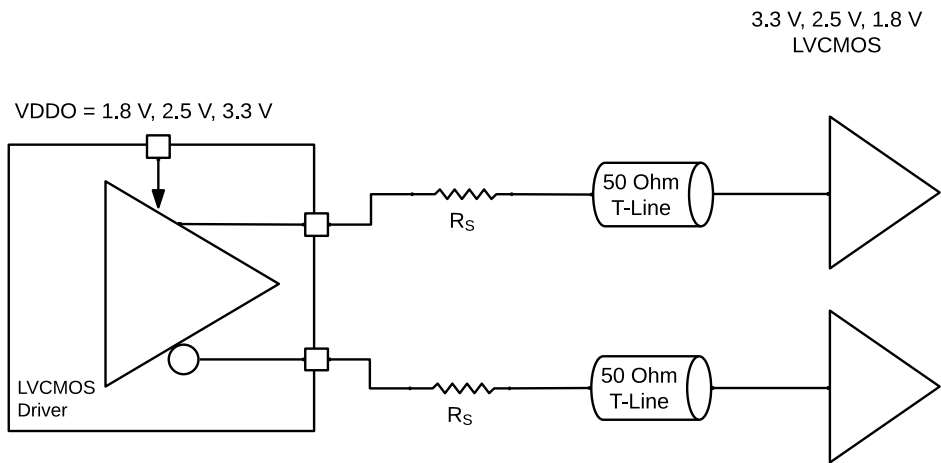
Figure 40. DC Coupled LVCMOS
