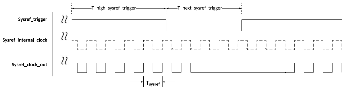
Figure 41. sysref_clock_out behavior with respect to sysref_trigger
