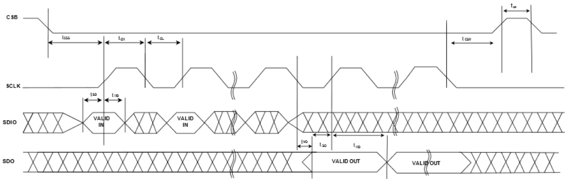
Figure 49. SPI Timing Diagram
