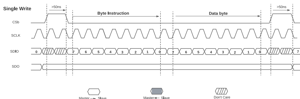
Figure 50. SPI Single Write
