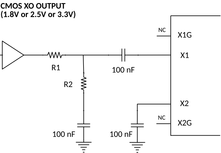
Figure 11. CMOS XO Connections
