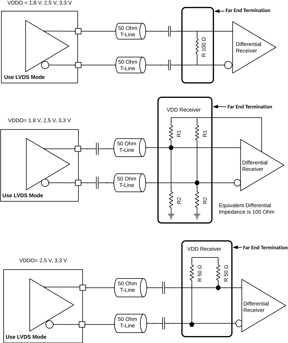
Figure 36. LVDS Output Driver used with AC Coupled terminations for various receivers
