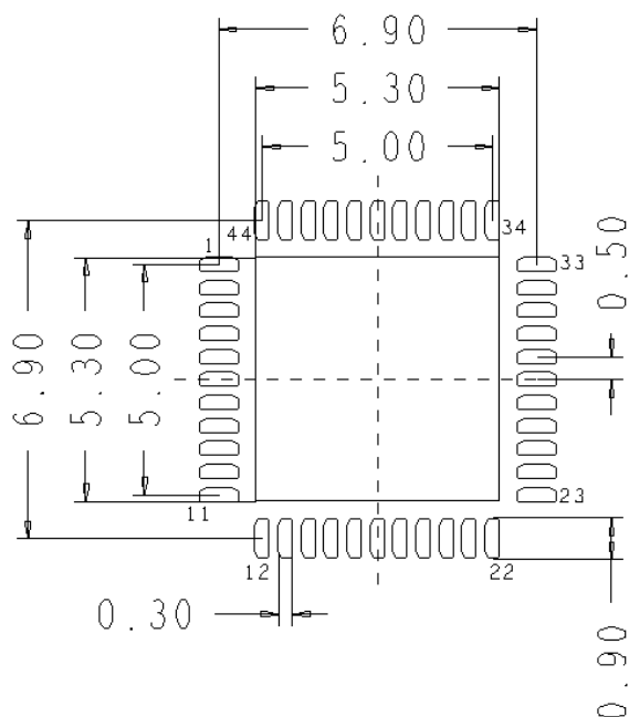
Figure 57. Land Pattern
