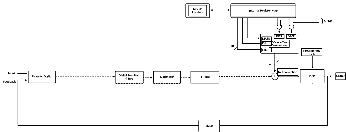
Figure 29. DCO Increment/Decrement path for Inner-Loop
