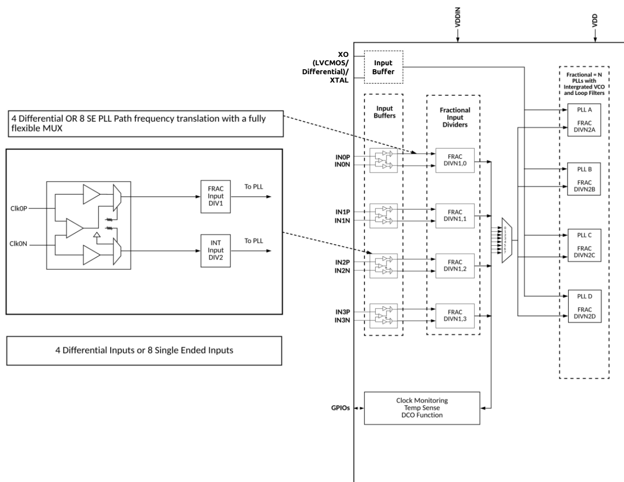
Figure 13. SiT95210 Input Slave Architecture
