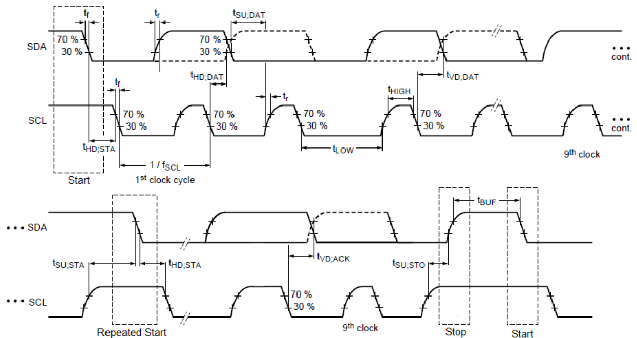
Figure 48. I2C Timing Waveform
