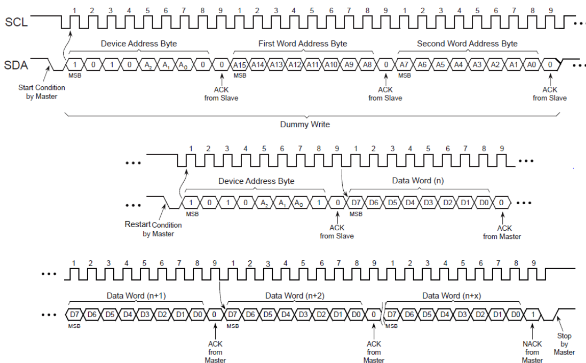
Figure 44. EEPROM read
