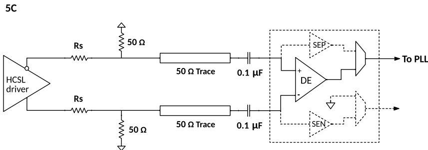
Figure 25. Interface Type V Differential AC Coupled 5C
