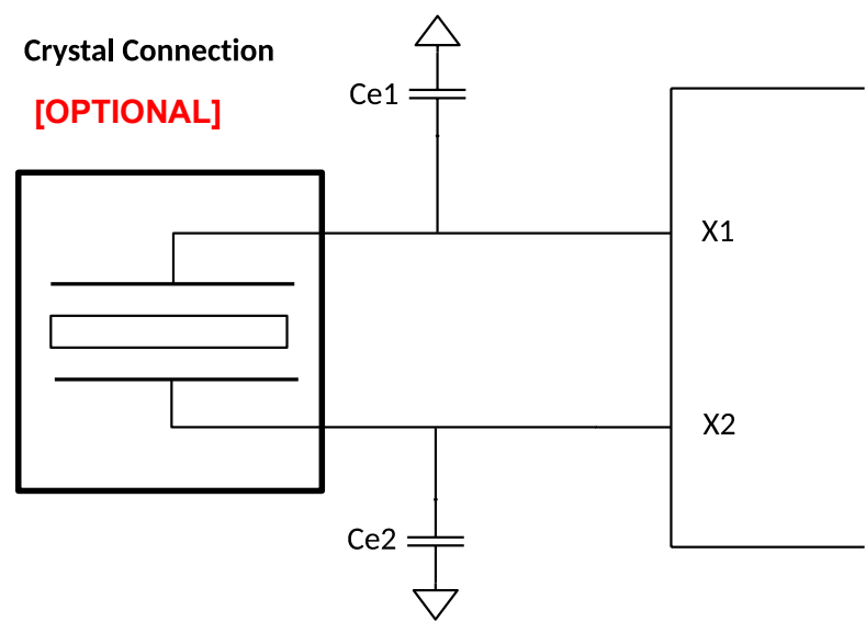
Figure 10. Crystal Connections
