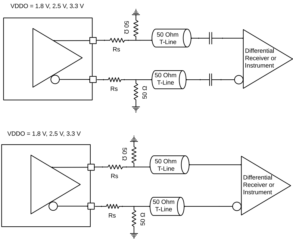
Figure 38. Output Driver used with traditional HCSL receiver
