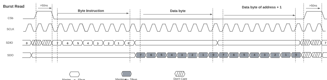
Figure 55. SPI Burst Read
