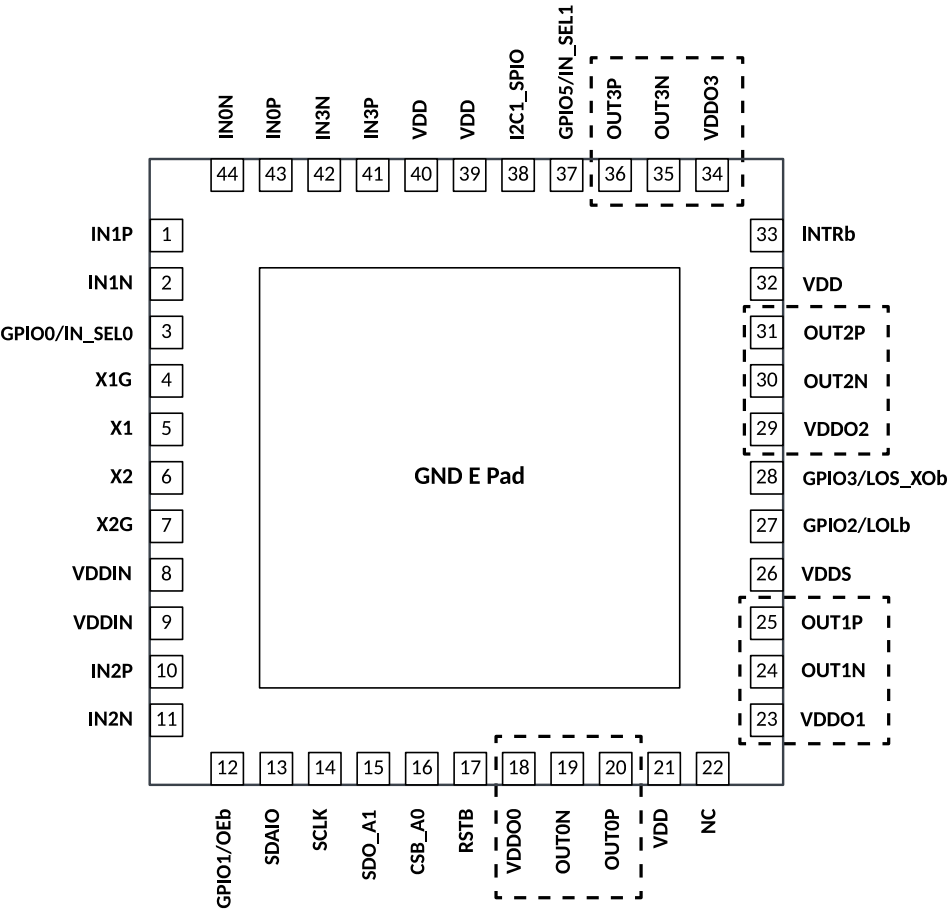
Figure 31. SiT95210 Output Drivers
