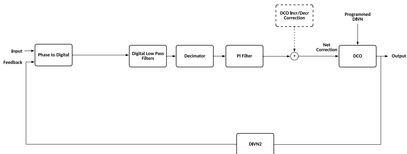
Figure 28. Basic Mode of Operation
