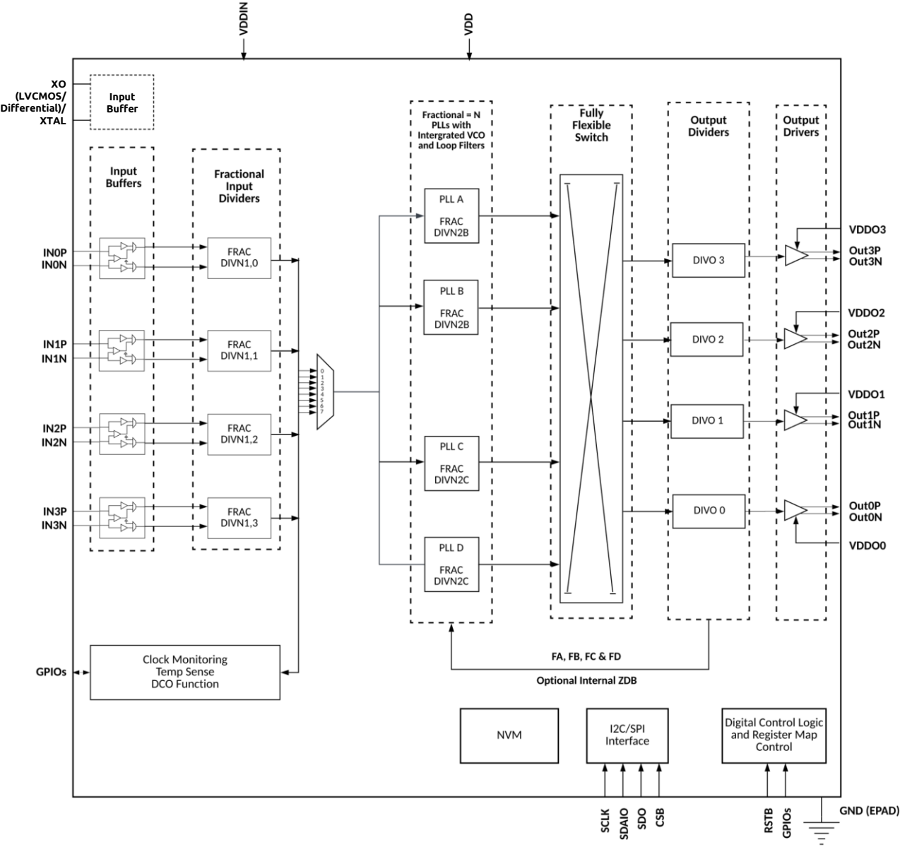
Figure 1. Functional Overview
