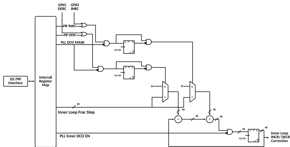
Figure 30. Architecture of the Inner-Loop Increment/Decrement path
