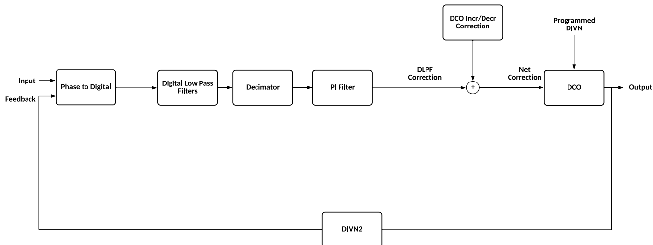
Figure 27. Basic DLPF Block Diagram
