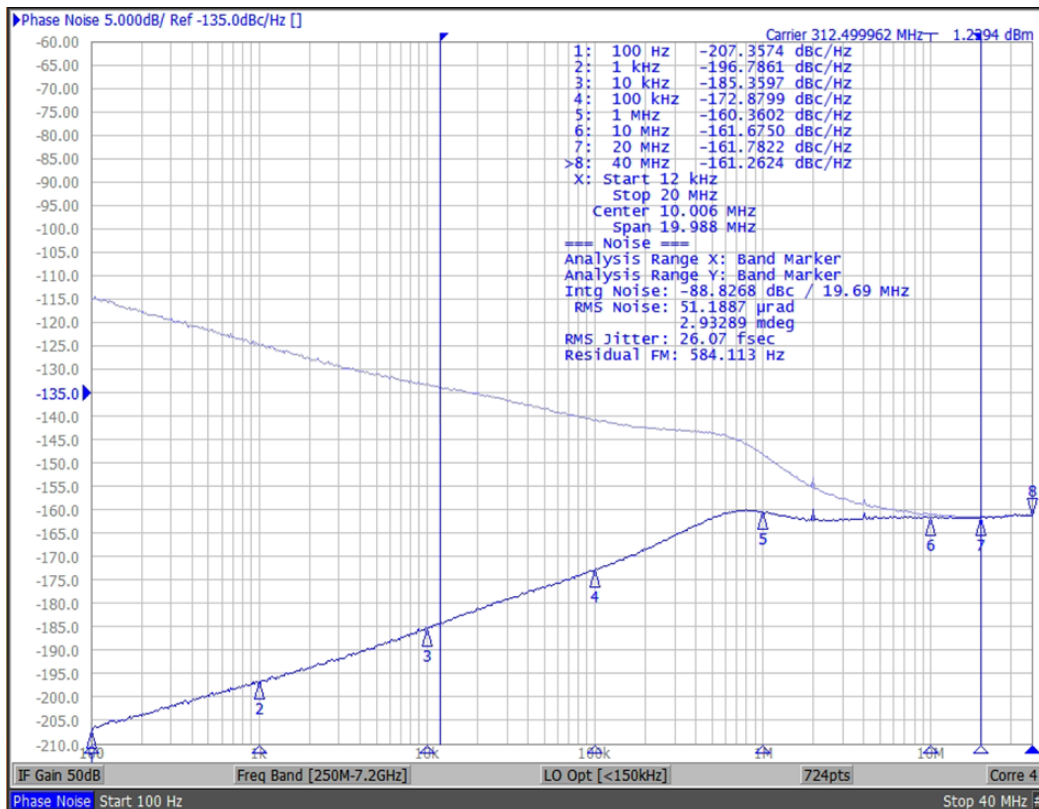
SiT95210: 312.5M Output (LVDS) with 96M SMA100B XO Source
