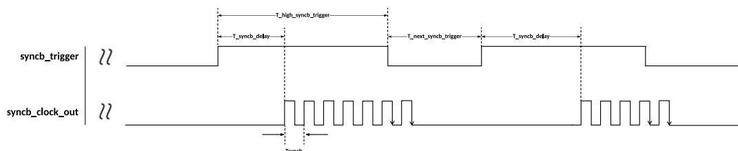
Figure 43. syncb_clock_out behavior with respect to syncb_trigger
