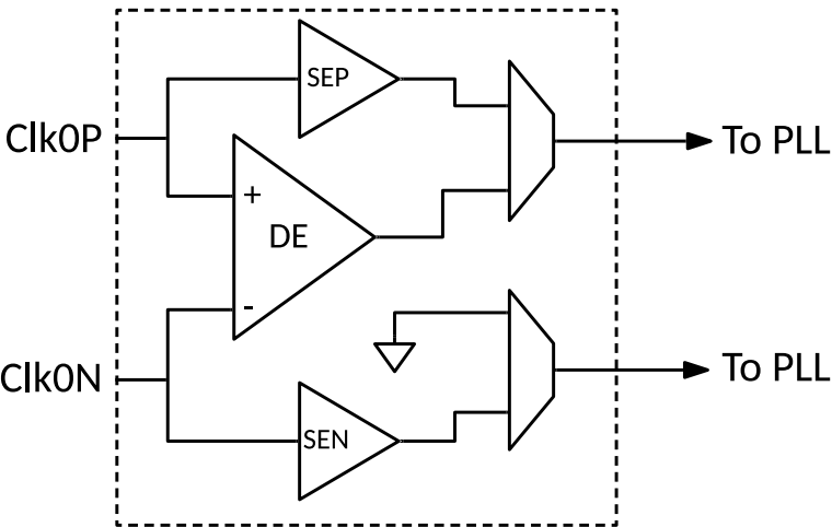
Figure 15. Input Buffer Structure
