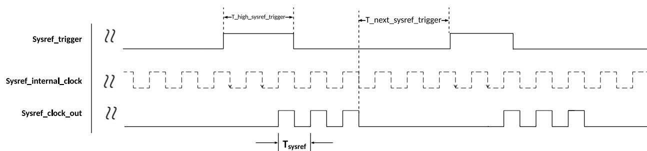
Figure 42. sysref_clock_out behaviour with respect to sysref_trigger in pulser mode
