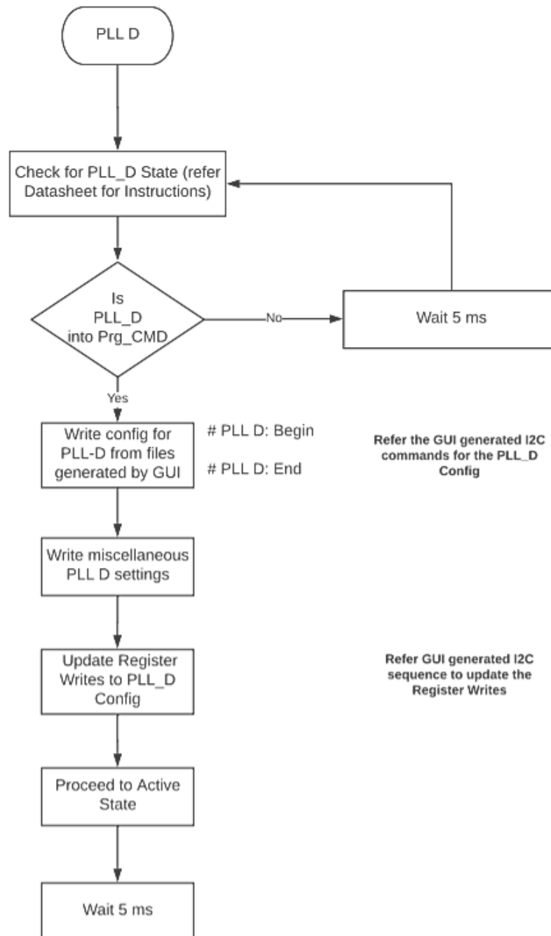
Figure 49. STEP 8: Initialize the PLL D System Page – Page D
