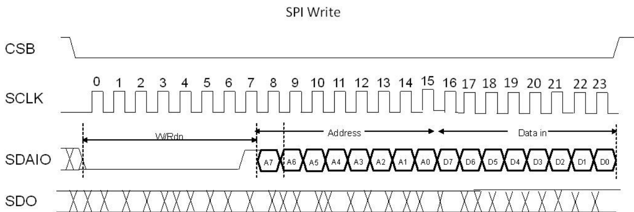
Figure 41. SPI Write Operation
