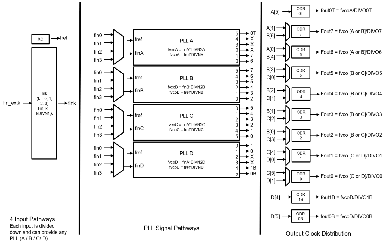
Figure 11. Overall Hierarchy of Clocks
