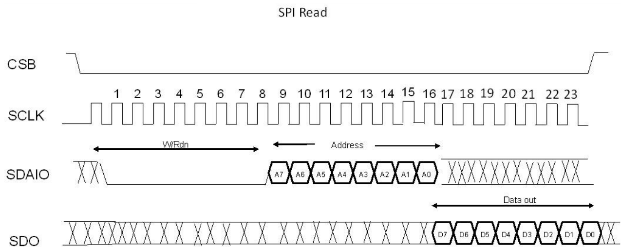
Figure 40. SPI Read Operation
