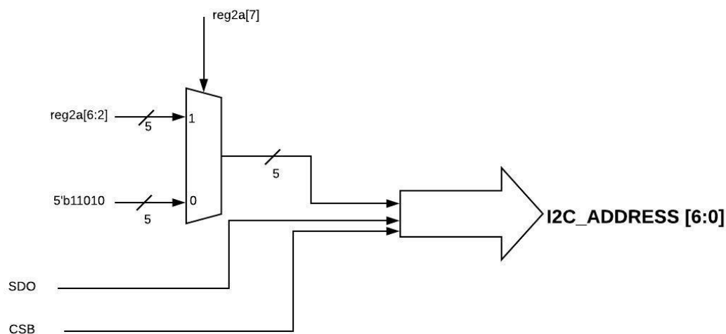
Figure 36. I 2 C Addressing Scheme for Cascade
