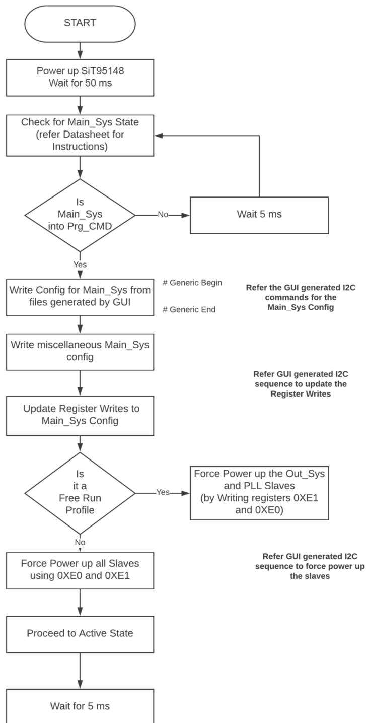
Figure 42. Step 1: Initialize the Main Page – Page 0
