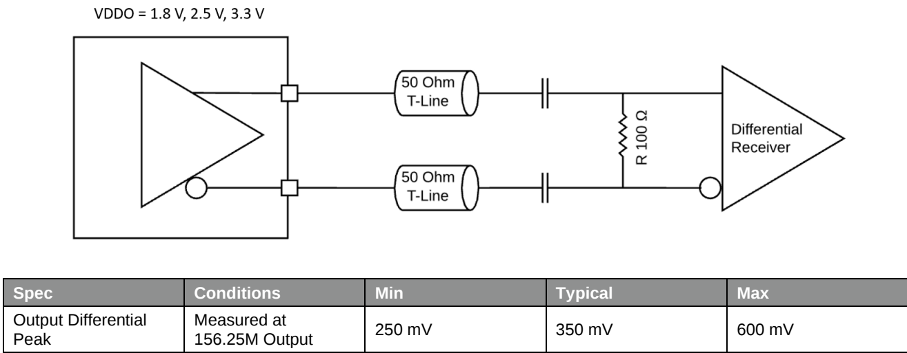
Figure 28. LVDS AC Termination at the Load
