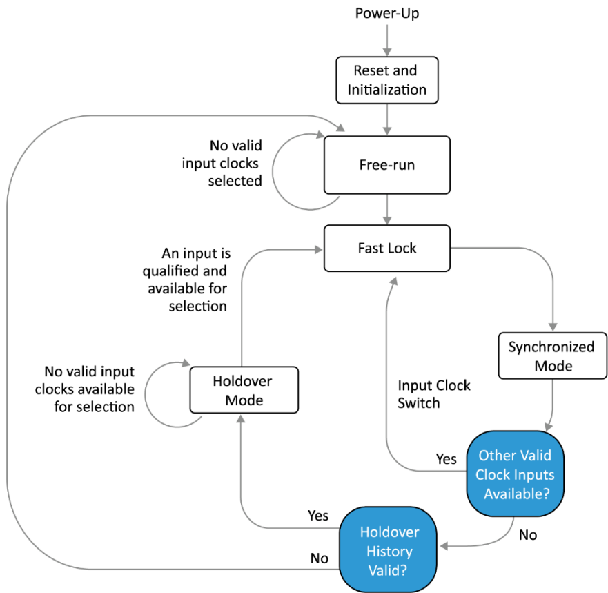
Figure 18. Operation Modes
