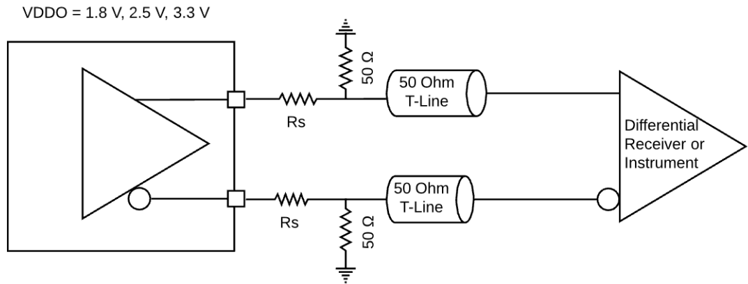
Figure 30. HCSL Interface Termination [51]
