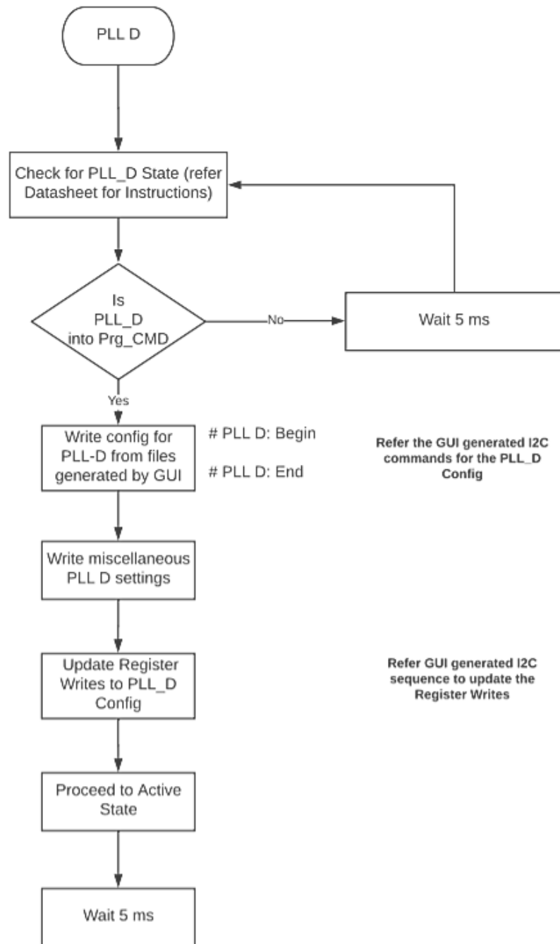
Figure 49. STEP 8: Initialize the PLL D System Page – Page D
