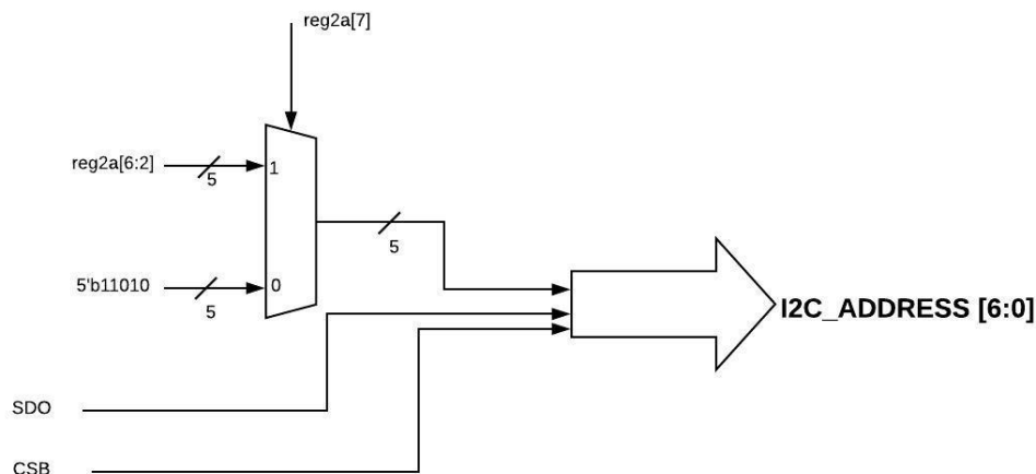
Figure 36. I 2 C Addressing Scheme for Cascade
