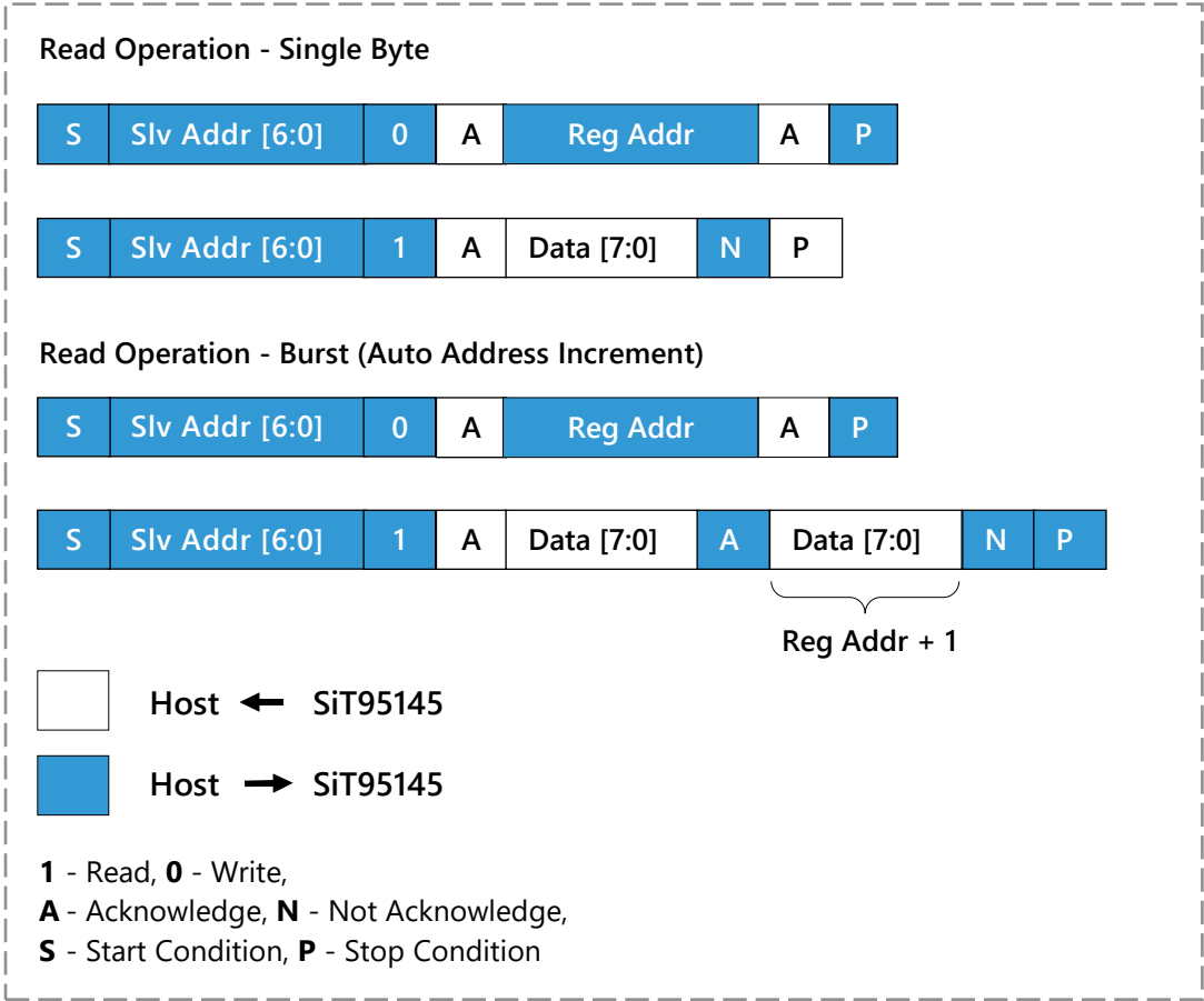
Figure 37. Read Block
