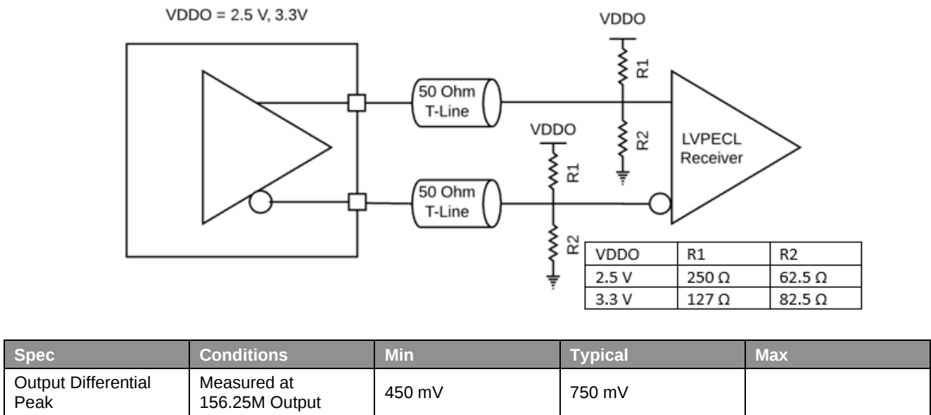
Figure 25. LVPECL DC-coupled Load Termination with Thevenin Equivalent Network
