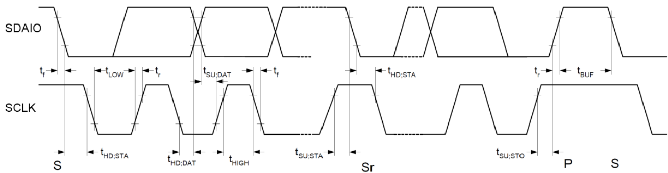
Figure 5. I 2 C Timing Waveform
