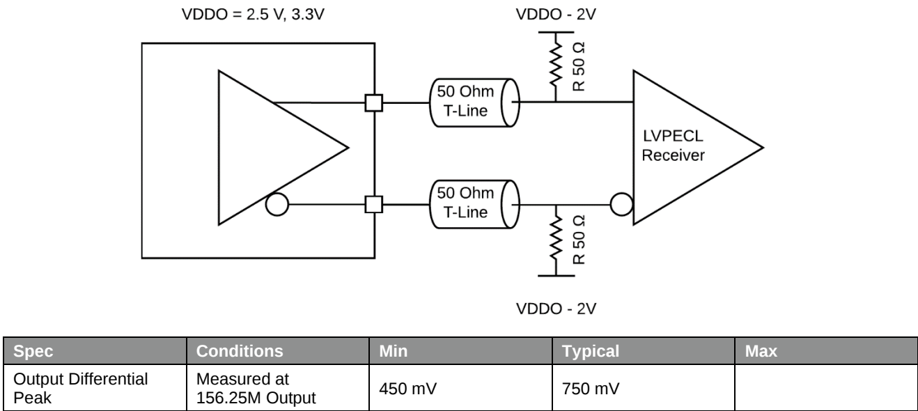
Figure 24. LVPECL with DC-coupled Termination
