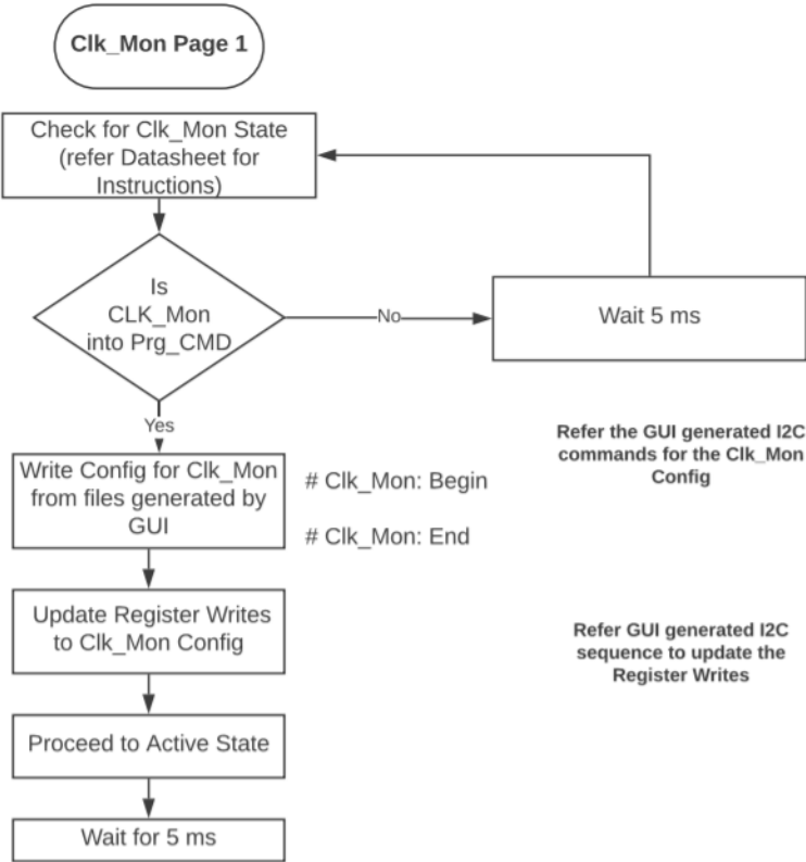
Figure 44. STEP 3: Initialize the Clock Monitor System Page – Page 1
