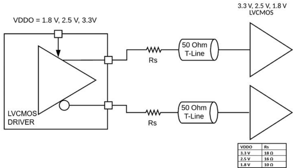
Figure 32. LVC MOS output Termination
