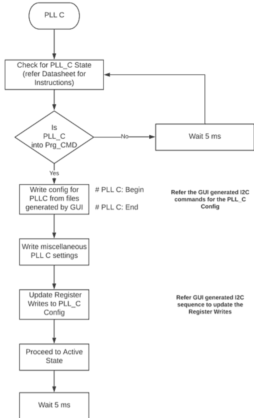
Figure 48. STEP 7: Initialize the PLL C System Page – Page C
