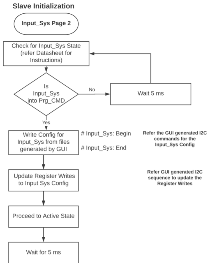
Figure 43. STEP 2: Initialize the Input System Page – Page 2
