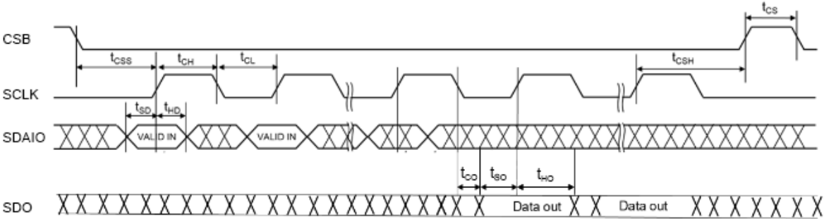
Figure 6. SPI Timing Waveform
