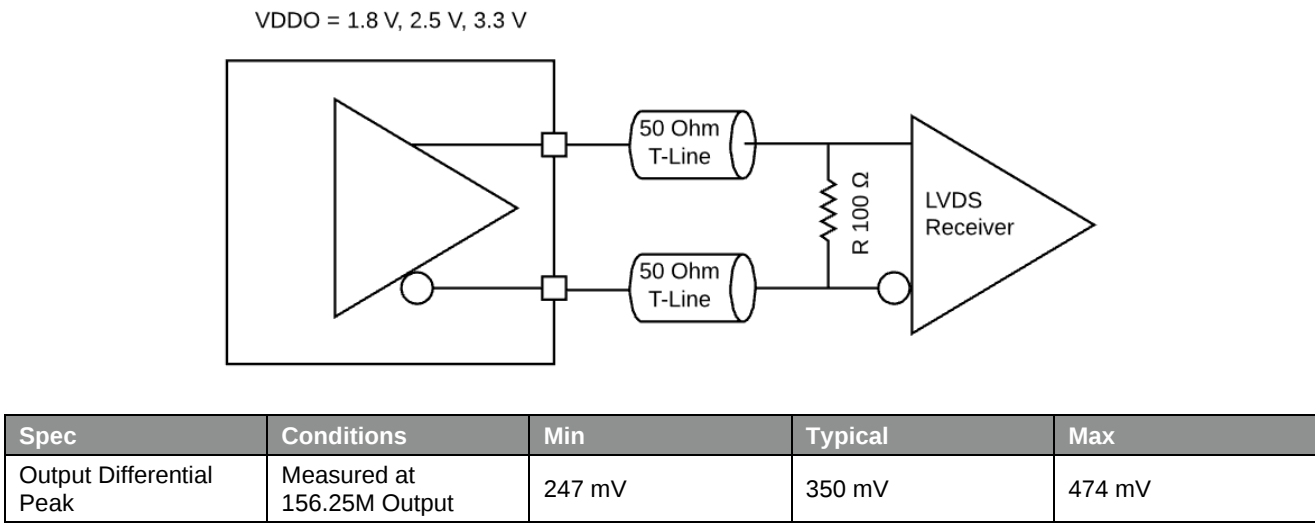
Figure 27. LVDS DC Termination at the Load
