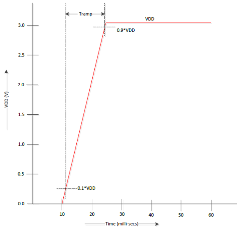
Figure 2. Supply Voltage Ramp
