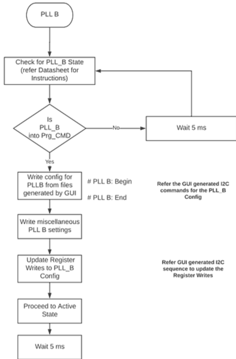
Figure 47. STEP 6: Initialize the PLL B System Page – Page B
