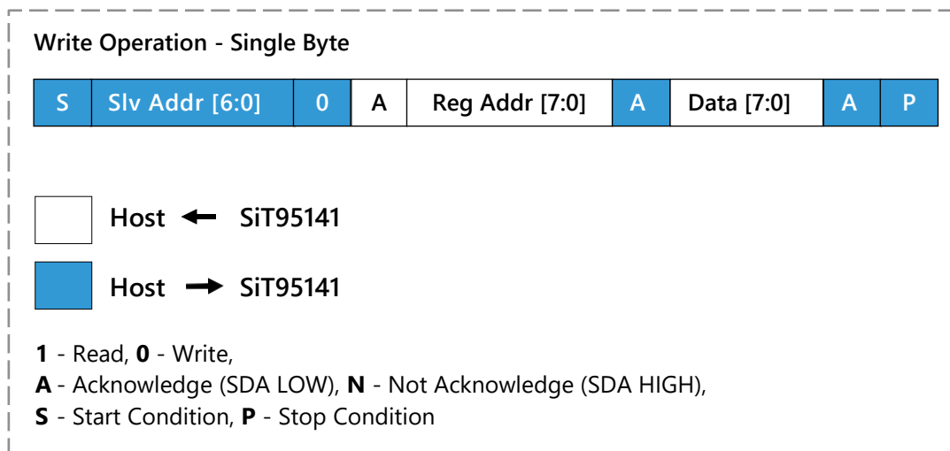
Figure 35. Write Block
