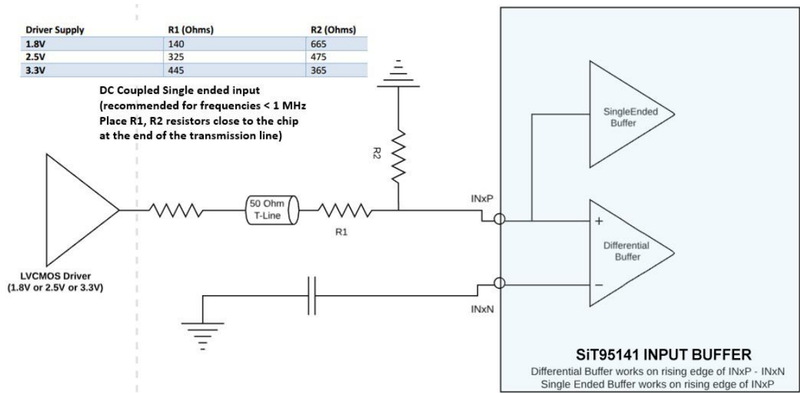
Figure 20. DC Coupled Single Ended Driver – Uses Single Ended Buffer Pathway [43]
