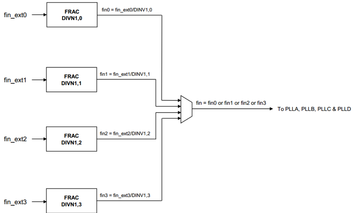
Figure 12. Input Clock Distribution
