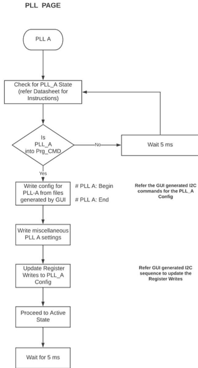
Figure 43. STEP 5: Initialize the PLL A System Page – Page A
