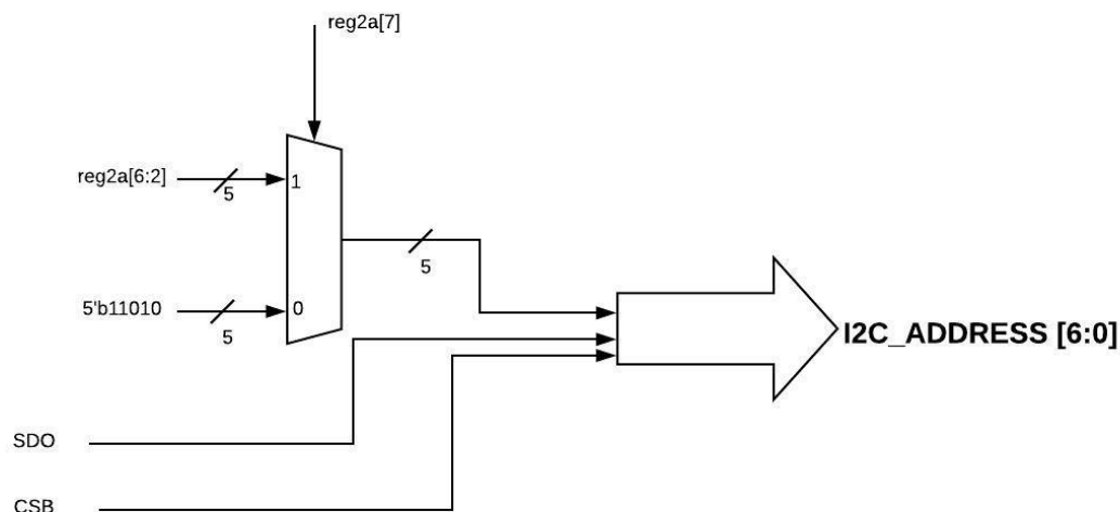
Figure 33. I 2 C Addressing Scheme for Cascade
