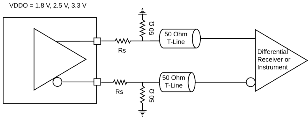
Figure 29. HCSL Interface Termination [44]
