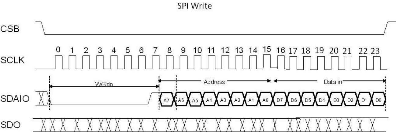
Figure 38. SPI Write Operation
