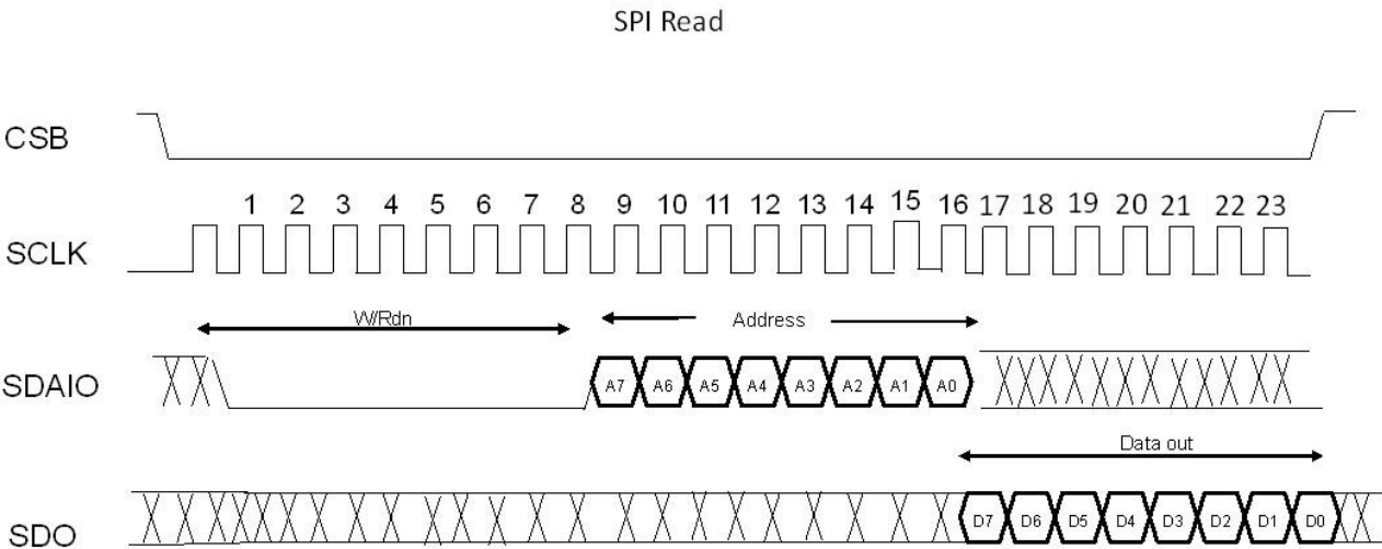
Figure 37. SPI Read Operation
