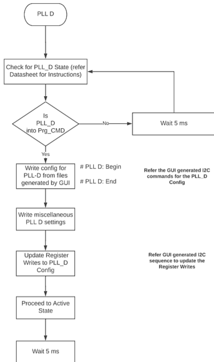
Figure 46. STEP 8: Initialize the PLL D System Page – Page D
