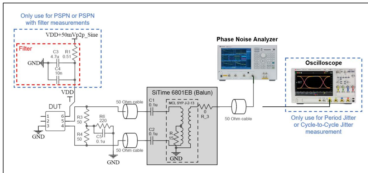
Figure 10. Test setup to measure FlexSwing Phase Noise, Period Jitter, Cycle-to-Cycle Jitter, and Power Supply-Induced Phase Noise (PSIPN) with and without filter added [19]
