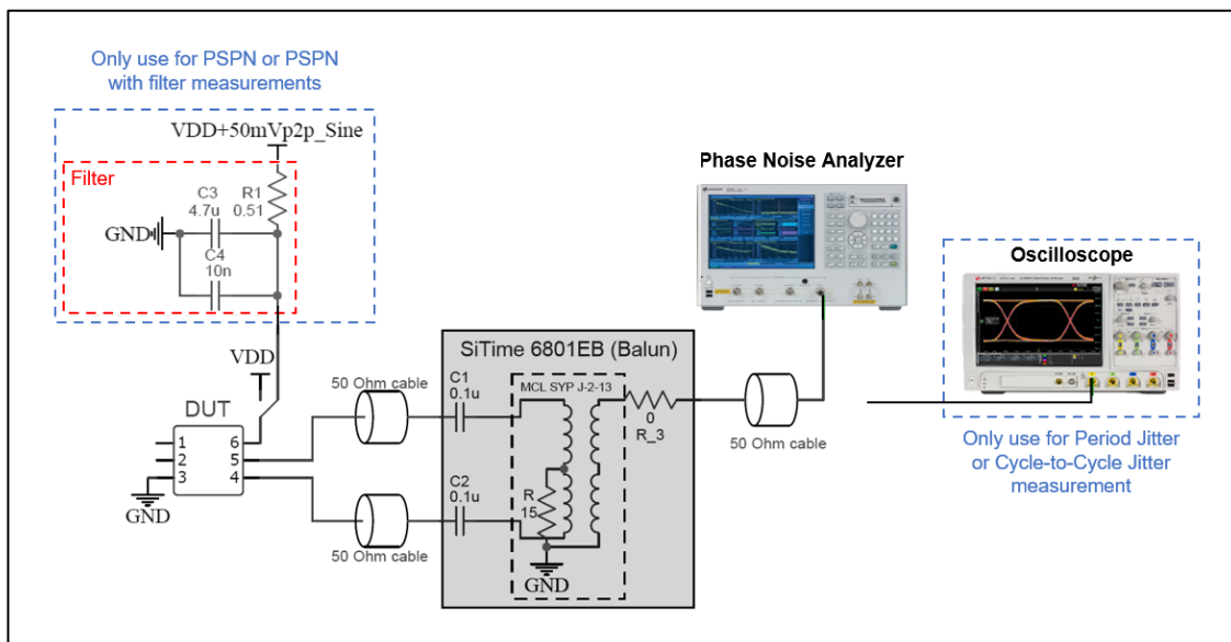
Figure 12. Test setup to measure LVDS Phase Noise, Period Jitter, Cycle-to-Cycle Jitter, and Power Supply-Induced Phase Noise (PSIPN) with and without filter added
