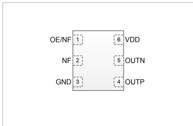
Figure 2. Pin Assignments (Top view) (Refer to Table 15 for Pin Descriptions)
