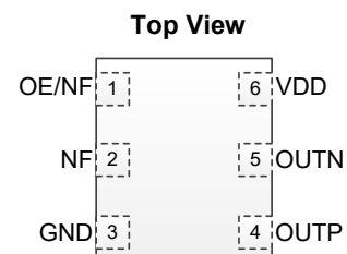
Figure 3. Pin Assignments
