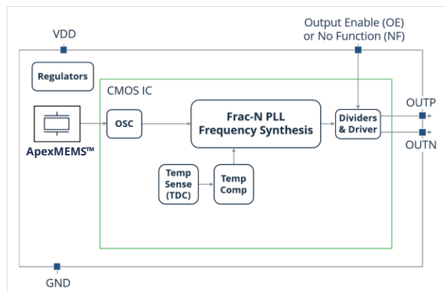
Figure 1. SiT9377 Block Diagram
