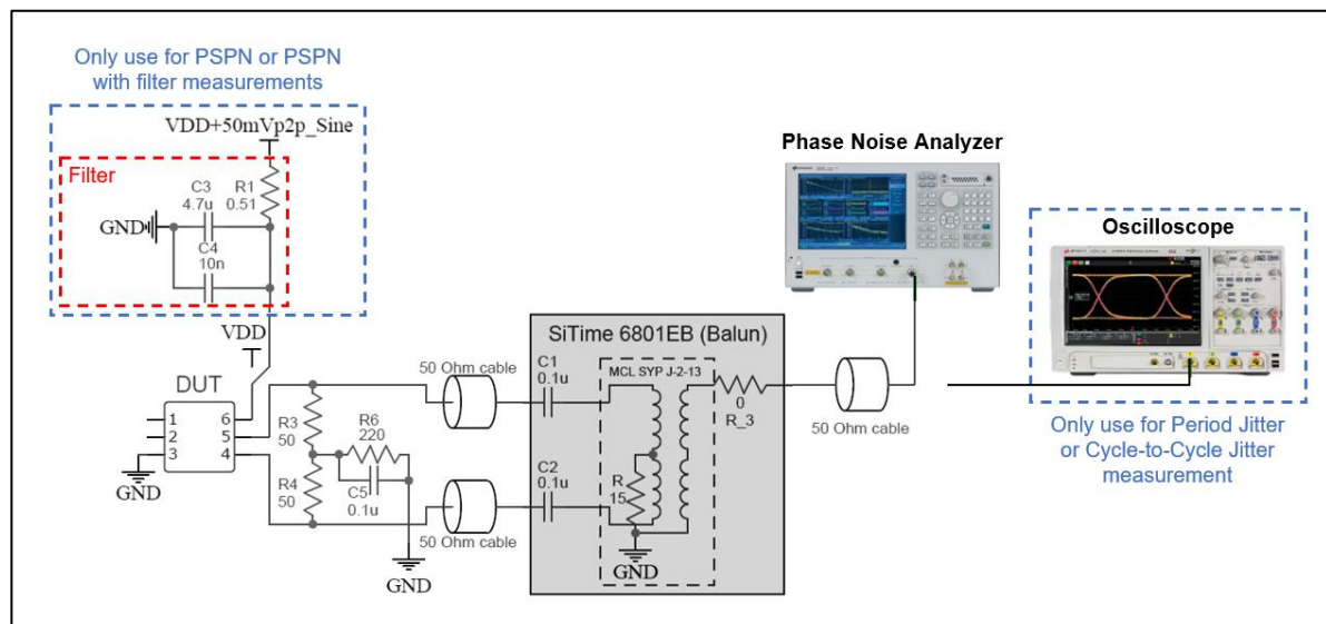
Figure 6. Test setup to measure FlexSwing Phase Noise, Period Jitter, Cycle-to-Cycle Jitter, and Power Supply-Induced Phase Noise (PSIPN) with and without filter added [15]
