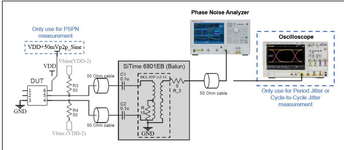
Figure 4. Test setup to measure LVPECL Phase Noise, Period Jitter, Cycle-to-Cycle Jitter, and Power Supply-Induced Phase Noise (PSIPN) without filter added [12]
