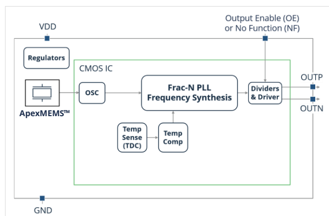
Figure 1. SiT9376 Block Diagram
