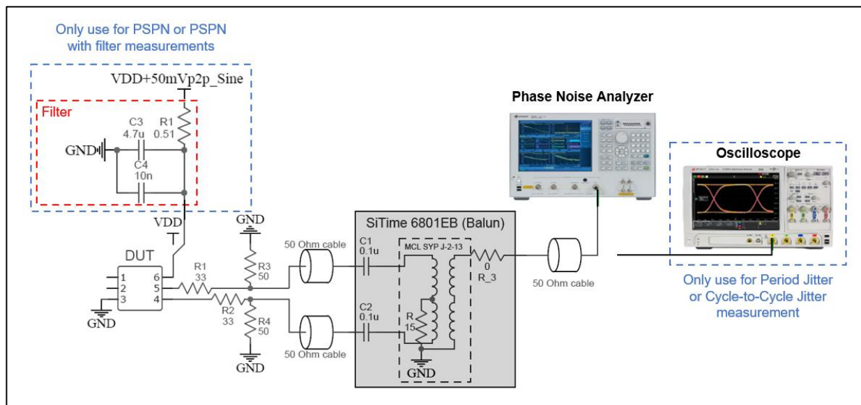
Figure 10. Test setup to measure HCSL Phase Noise, Period Jitter, Cycle-to-Cycle Jitter, and Power Supply-Induced Phase Noise (PSIPN) with and without filter added
