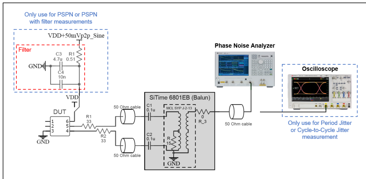
Figure 12. Test setup to measure Low-Power HCSL Phase Noise, Period Jitter, Cycle-to-Cycle Jitter, and Power Supply-Induced Phase Noise (PSPIN) with and without filter added
