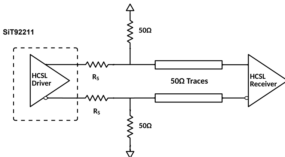
Figure 27. Termination scheme for DC coupled HCSL
