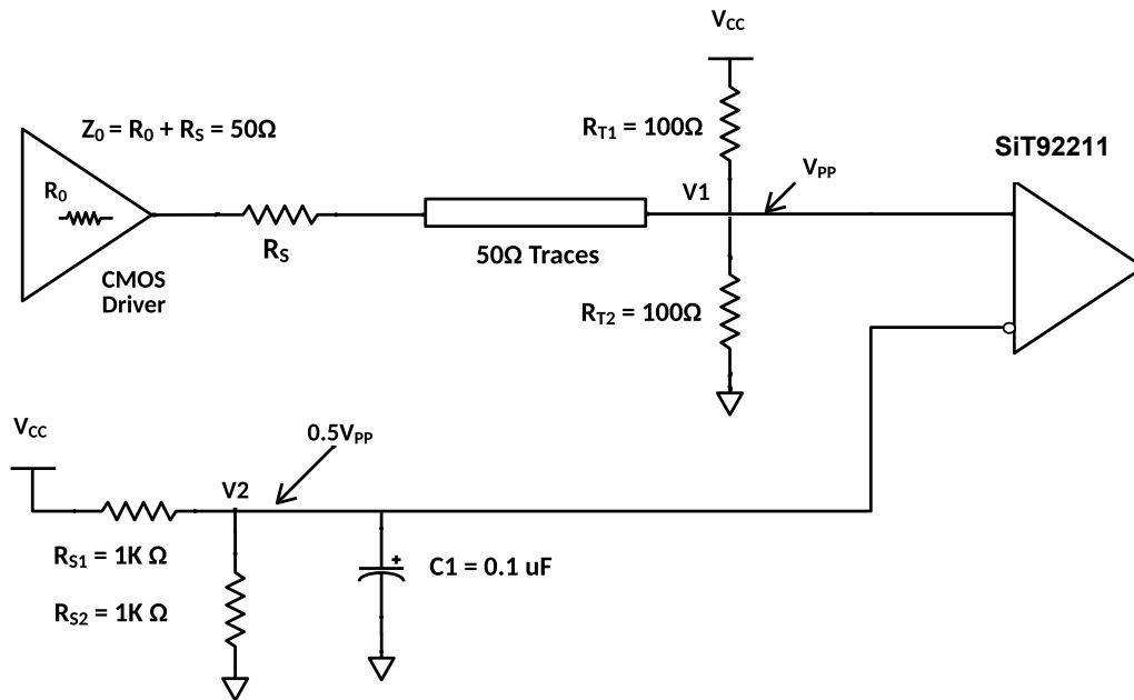
Figure 7. DC coupling of LVCMOS clock to SiT92211 – configuration 1
