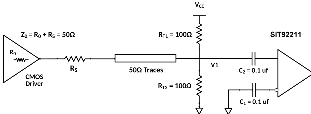
Figure 5. AC coupling LVCMOS clock to SiT92211
