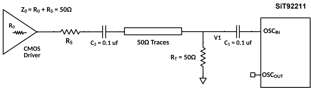
Figure 12. Single ended LVCMOS input – configuration 2, AC coupling to crystal input
