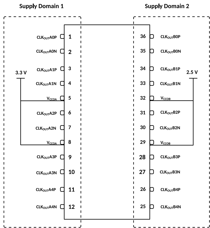
Figure 48. Multi Supply operation of SiT92211
