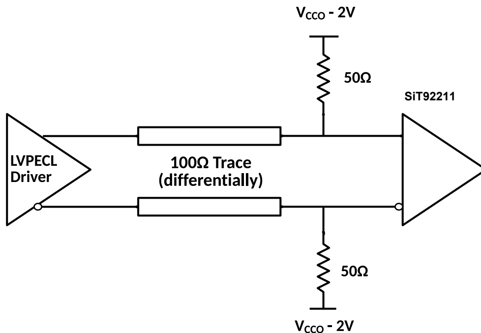
Figure 16. Termination scheme for DC coupled LVPECL
