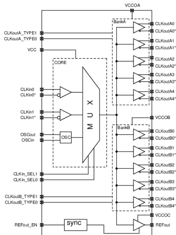
Figure 1. SiT92211 Block Diagram
