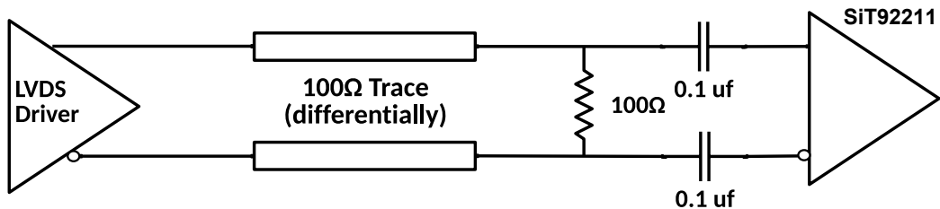
Figure 19. Termination scheme for AC coupled LVDS
