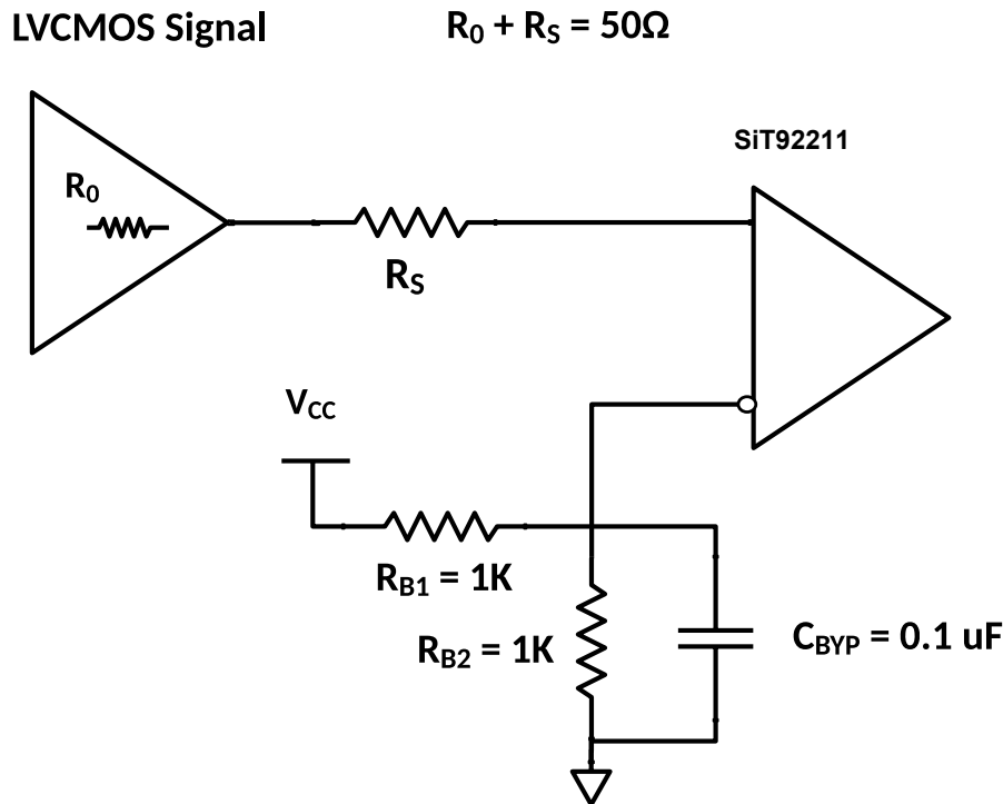
Figure 10: Direct coupling of LVCMOS clock to SiT92211
