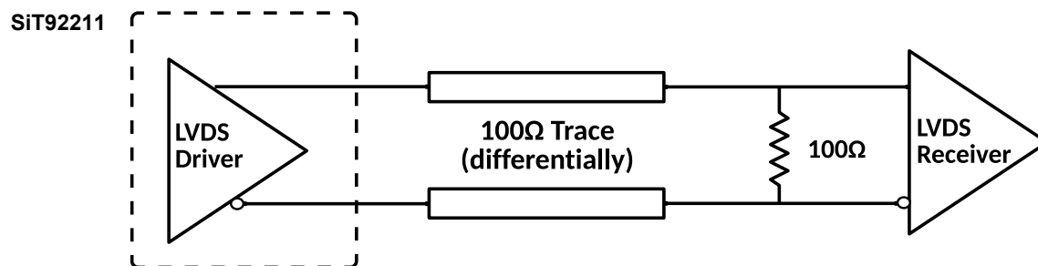
Figure 26. Termination scheme for DC coupled LVDS
