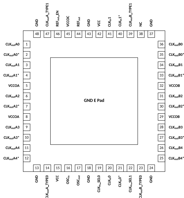
Figure 2. SiT92211 Pin configuration top view
