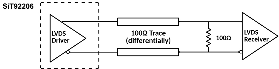
Figure 26. Termination Scheme for DC Coupled LVDS
