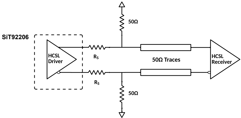
Figure 27. Termination Scheme for DC Coupled HCSL
