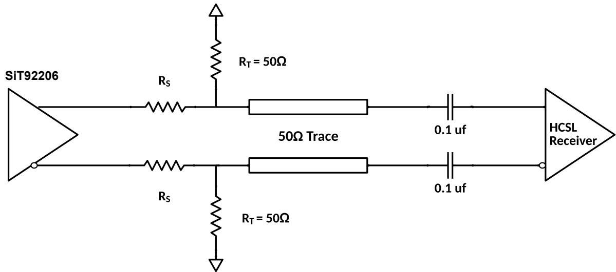
Figure 35. Output Driver Termination in HCSL AC-Coupled Mode
