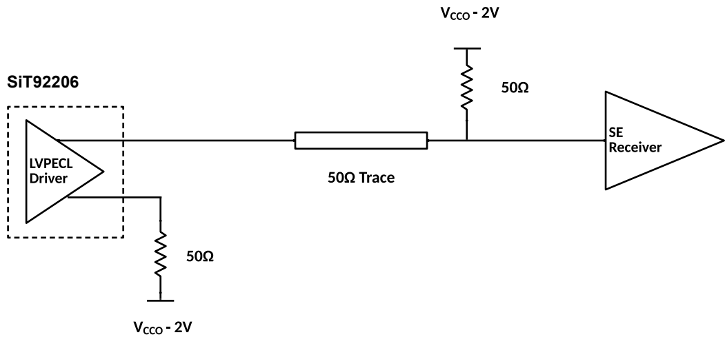
Figure 32. Termination Scheme for DC Coupled LVPECL, Single-Ended
