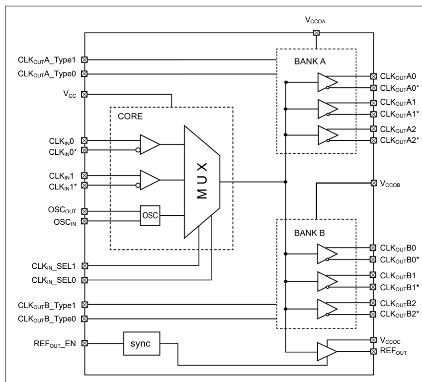
Figure 1. SiT92206 Block Diagram
