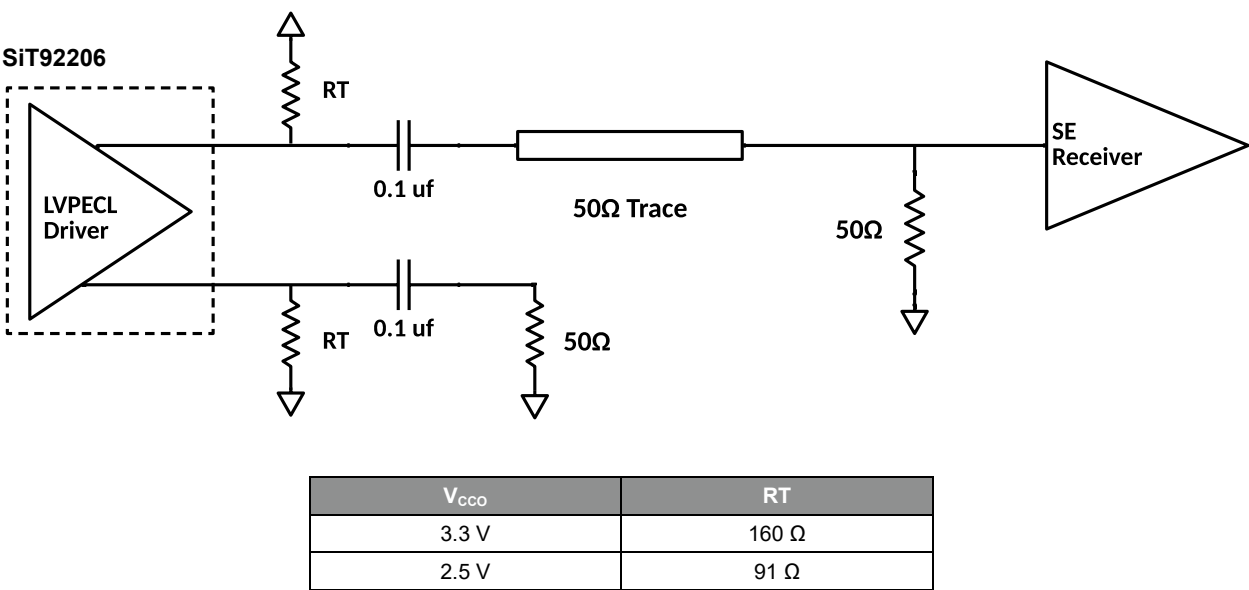
Figure 34. Termination Scheme for AC Coupled LVPECL, Single-Ended
