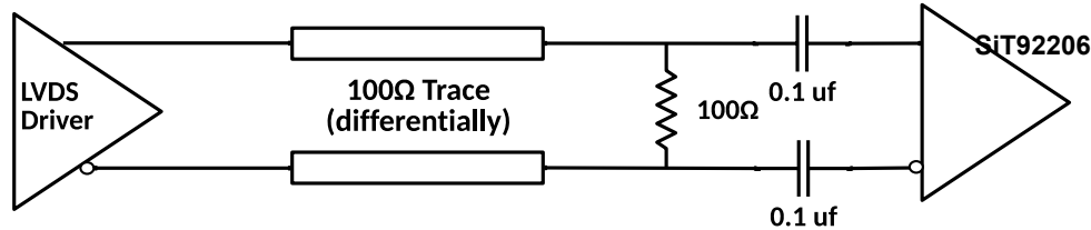
Figure 19. Termination Scheme for AC Coupled LVDS
