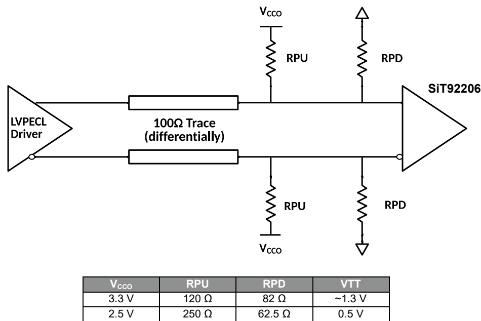
Figure 17. Termination Scheme for DC-Coupled LVPECL, Thevenin Equivalent
