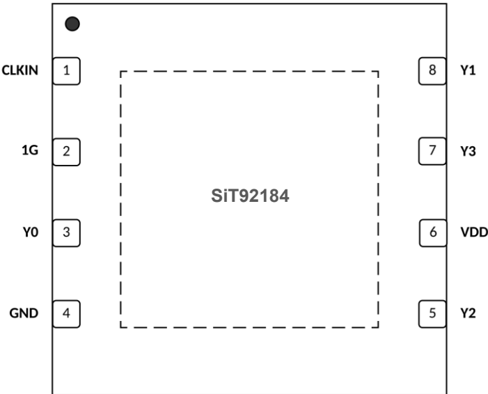
Figure 2. SiT92184 Pin Configuration
