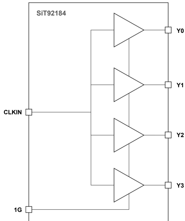
Figure 1. SiT92184 Functional Overview
