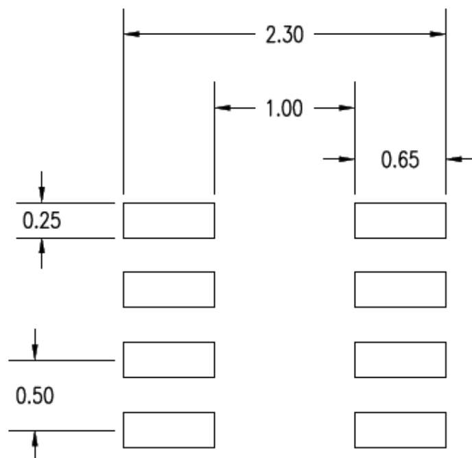
Figure 6. Recommended Land Pattern Dimension
