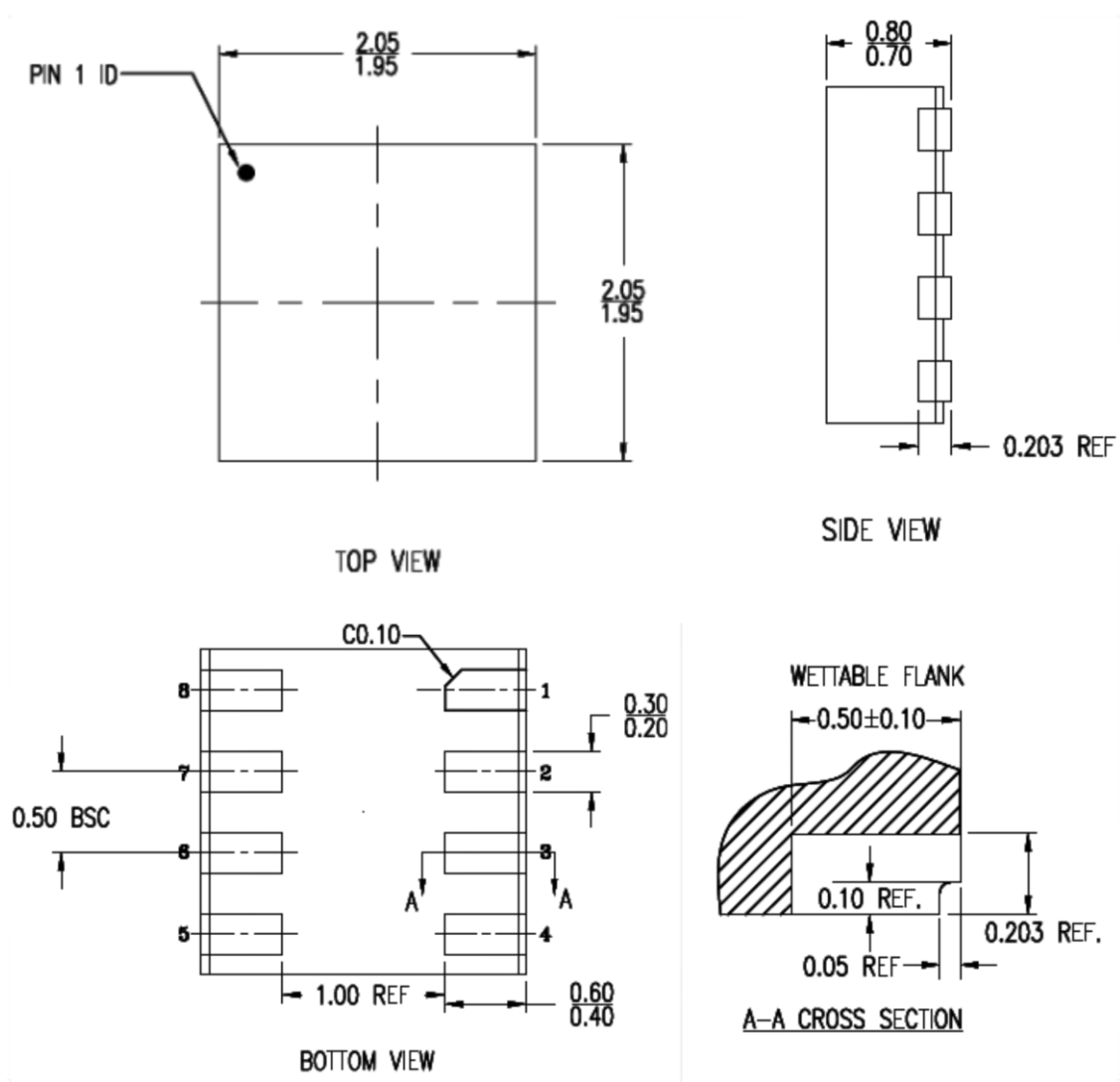
Figure 5. SiT92184 Cross Sections
