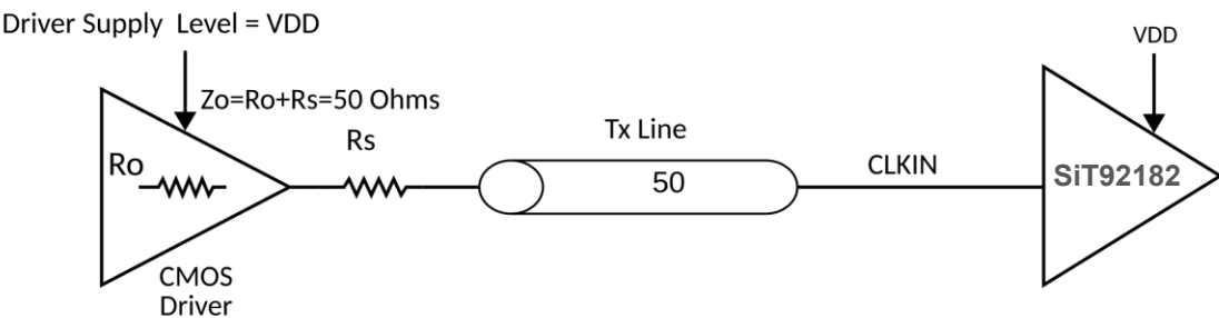
Figure 4. Recommended input clock configuration
