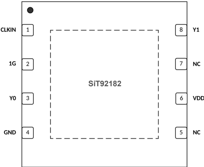
Figure 2. SiT92182 Pin Configuration
