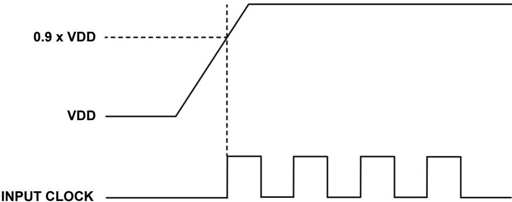
Figure 5. Input clock to VDD ramp timing requirement for SiT92182 LVCMOS
