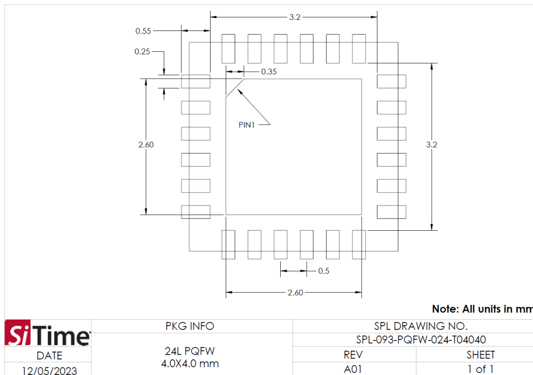
Recommended Land Pattern – Dimensions (Unit: mm)
