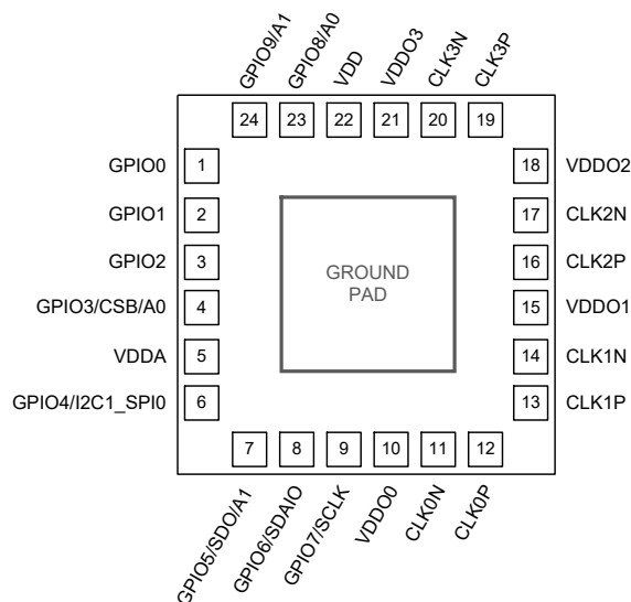
Figure 31. Top View
