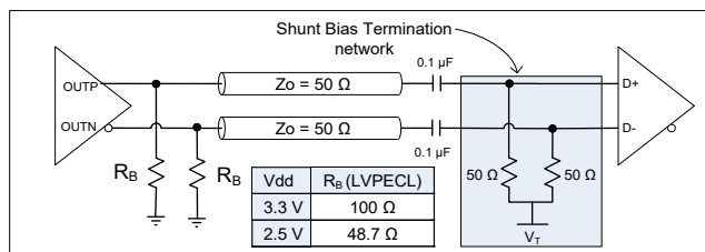
Figure 21. Recommended LVPECL and FlexSwing [9] Termination when AC-coupled
