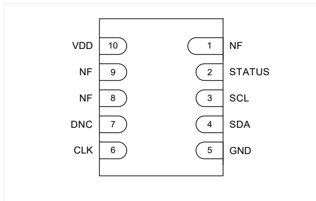
Figure 2. Pin Assignments (Bottom view)
