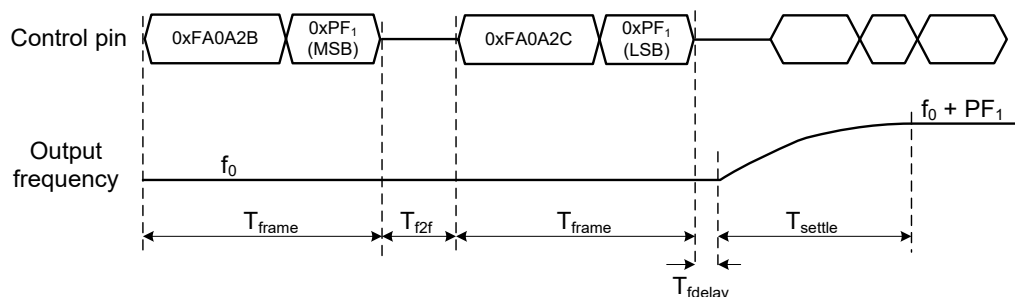
Figure 4. Frame Timing
