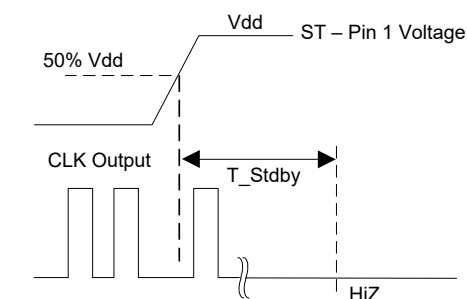
Figure 16. Standby Timing [7]
