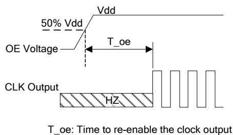
Figure 13. OE Enable Timing (OE Mode Only)
