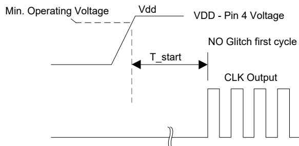
Figure 12. Startup Timing [7]
