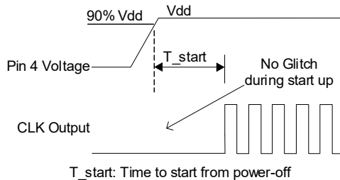
Figure 4. Startup Timing ( \overline{\text{ST}} / \overline{\text{MS}} / NC Mode) [10]
