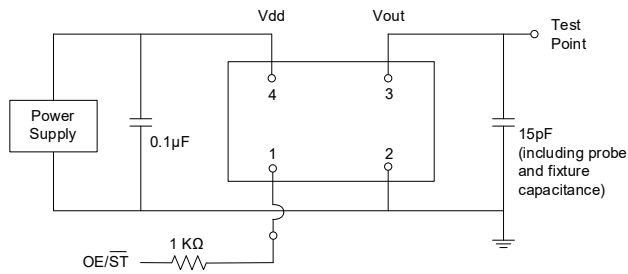
Figure 2. Test Circuit [0]
