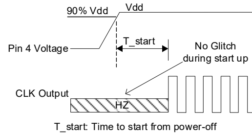
Figure 5. Startup Timing (OE Mode only) [10]
