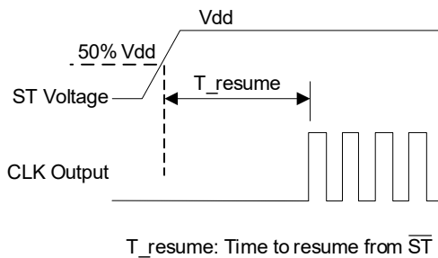
Figure 6. Standby Resume Timing ( \overline{\text{ST}} / \overline{\text{MS}} Mode) [10]
