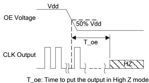
Figure 8. OE Disable Timing (OE Mode Only)
