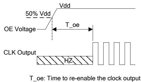
Figure 7. OE Enable Timing (OE Mode Only)
