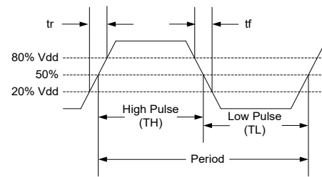
Figure 3. Waveform [0]
